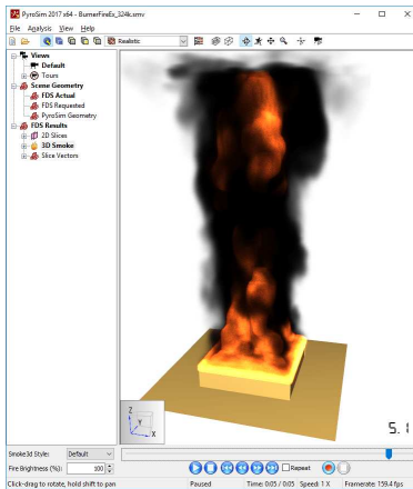
Figure 18. Hardware Shaders
