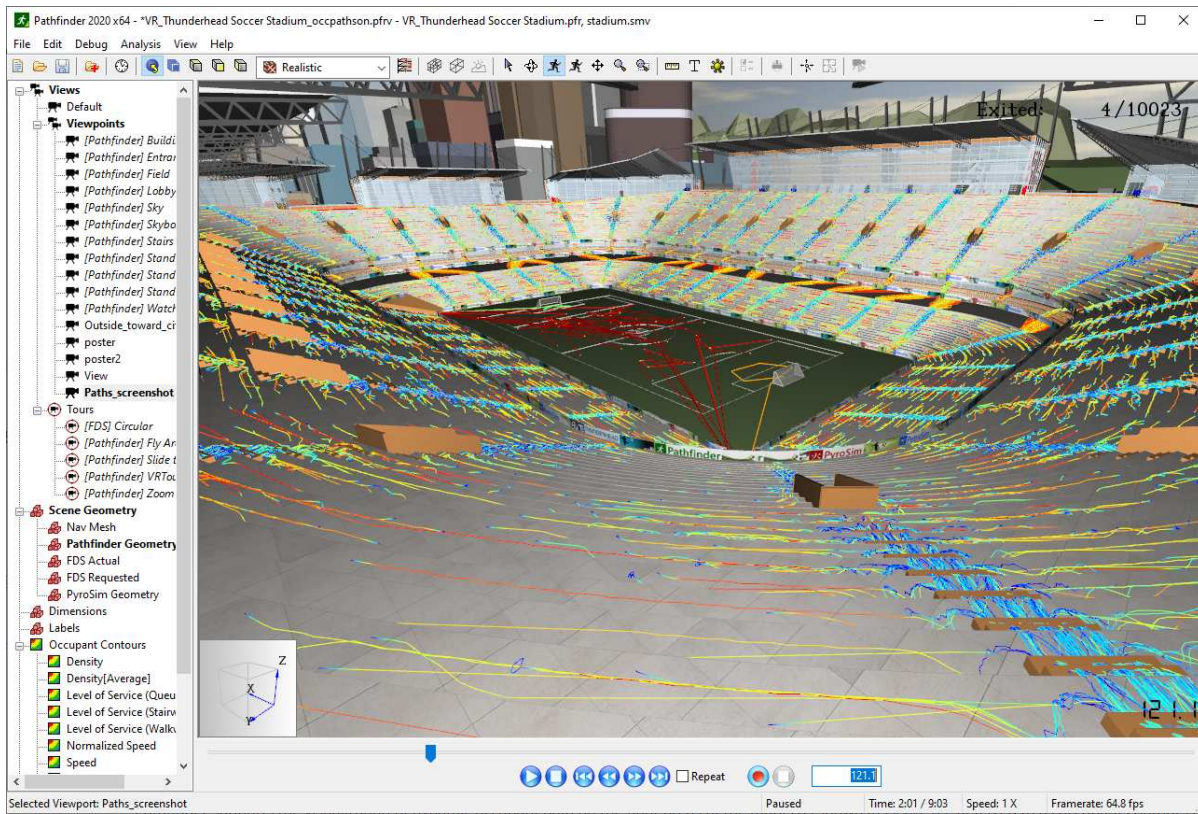
Figure 86. Occupant paths
