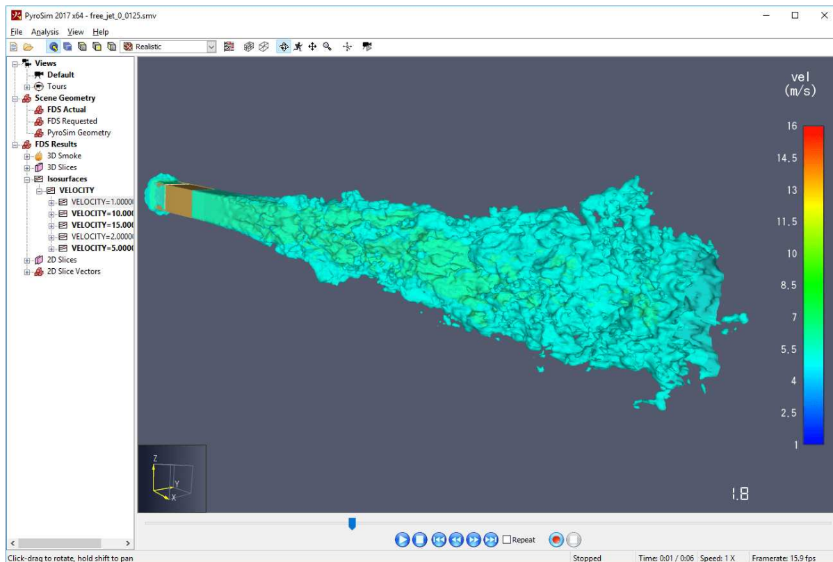
Figure 70. FDS Isosurfaces
