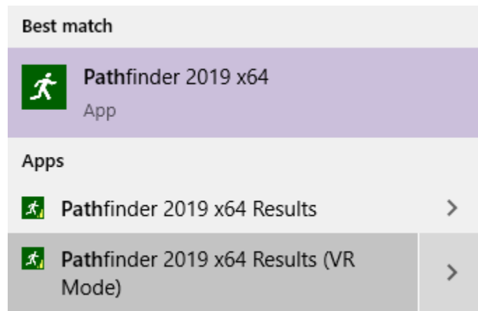
Figure 32. Shortcut Menu
