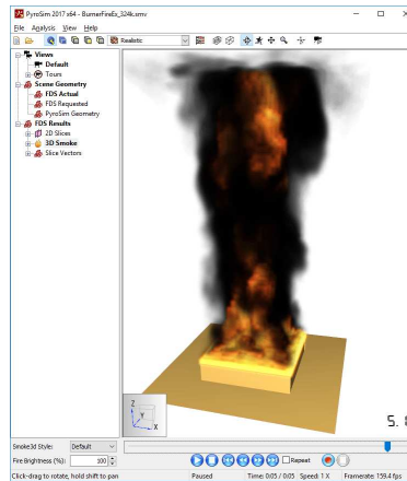
Figure 19. Compatibility Renderer
