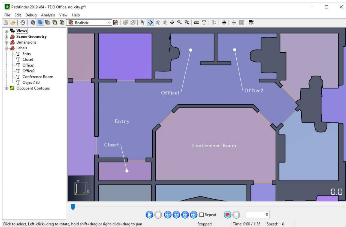
Figure 46. Custom Labels
