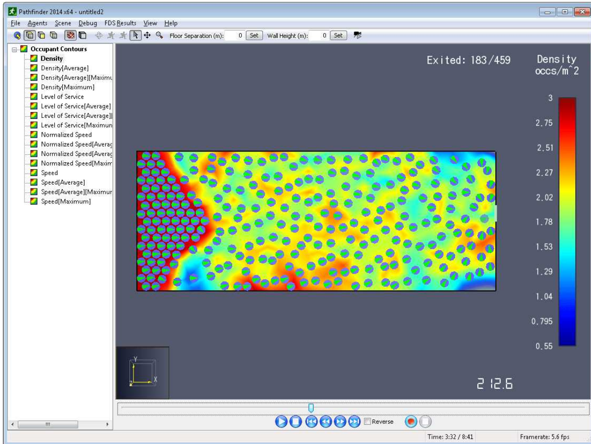
Figure 108. Occupant contours
