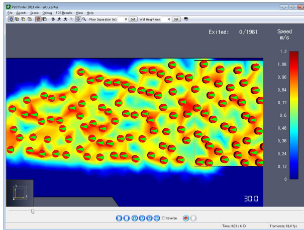
Figure 99. Triangle area= .25\text{m}^2 (default)
