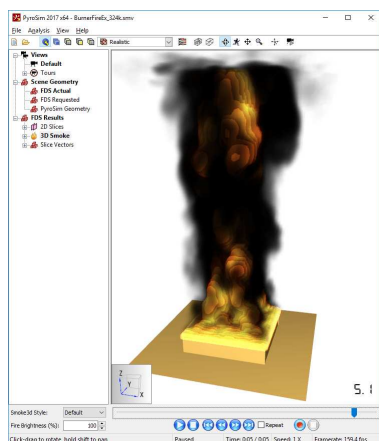
Figure 22. Smokeview Renderer
