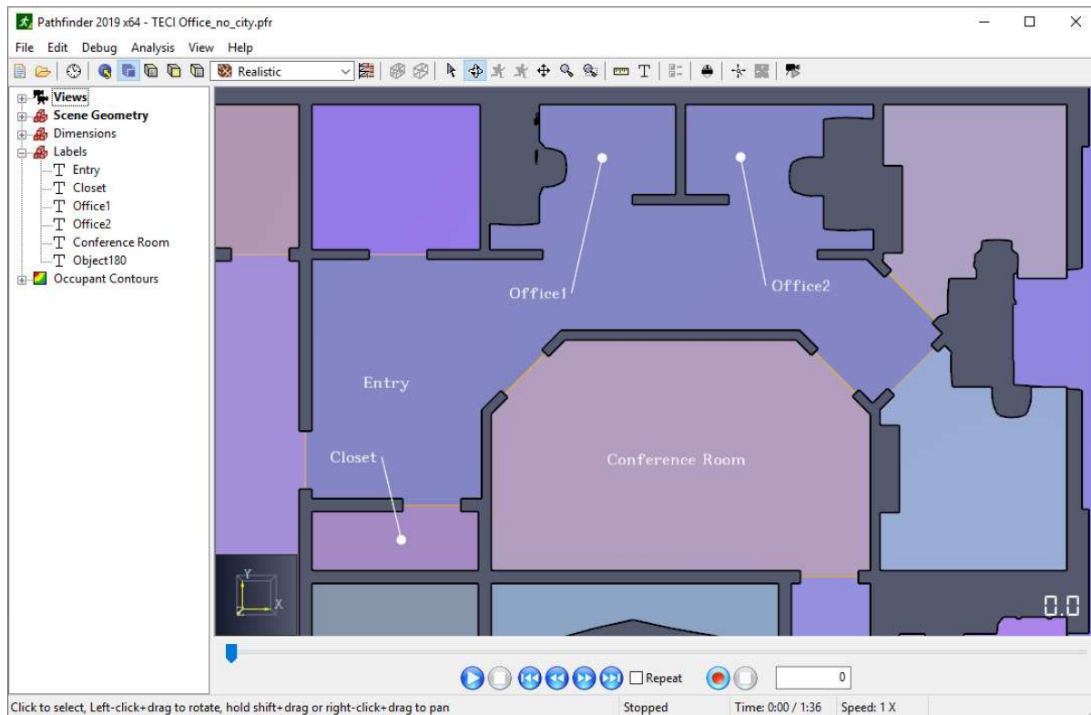
Figure 54. Custom Labels
