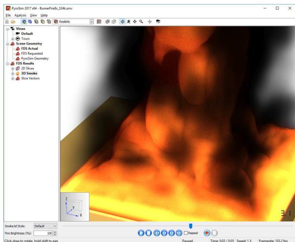
Figure 24. On
