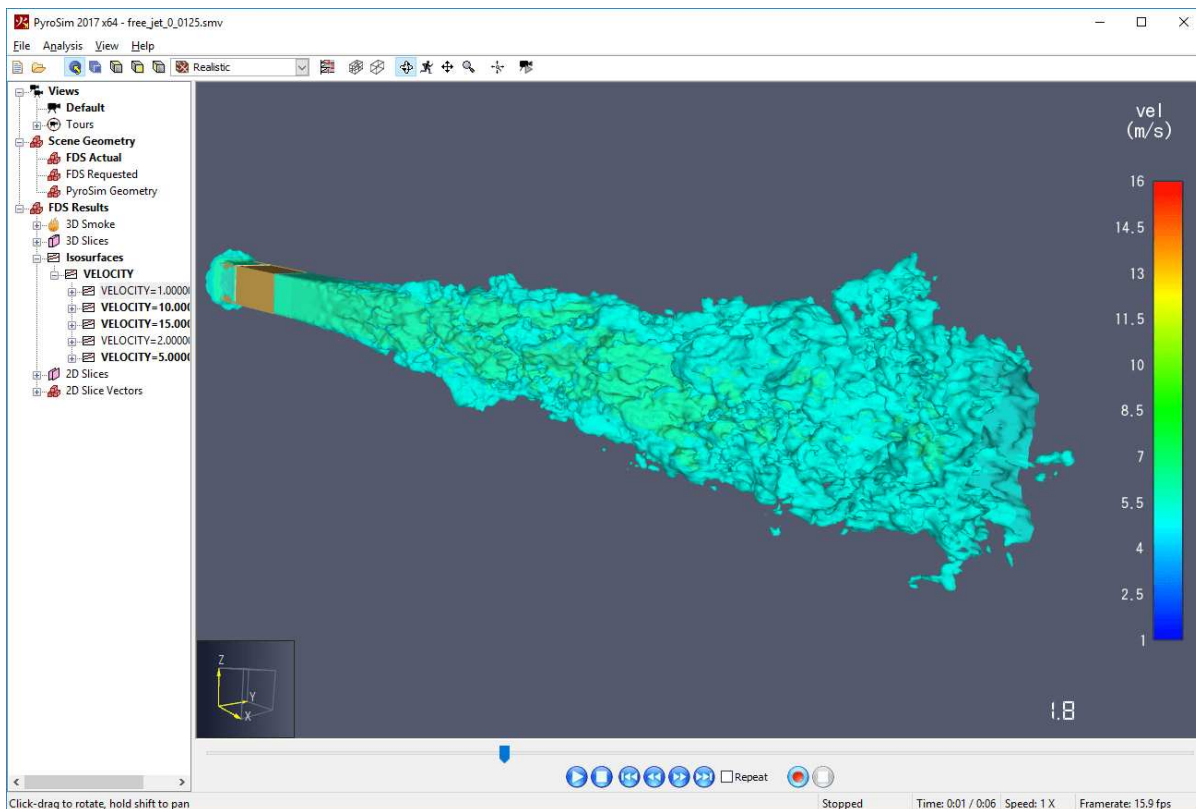
Figure 78. FDS Isosurfaces
