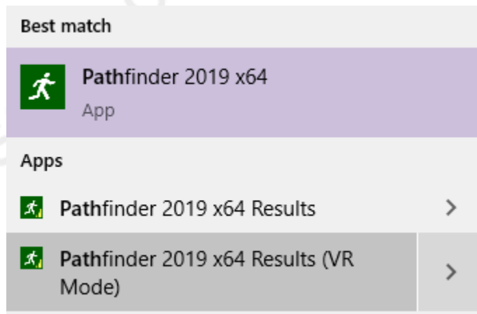
Figure 40. Shortcut Menu
