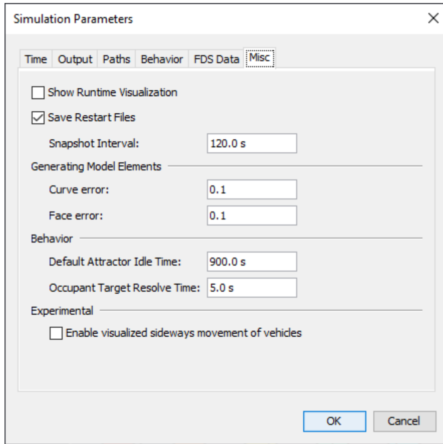
Figure 148. The Miscellaneous tab of the Simulation Parameters dialog
