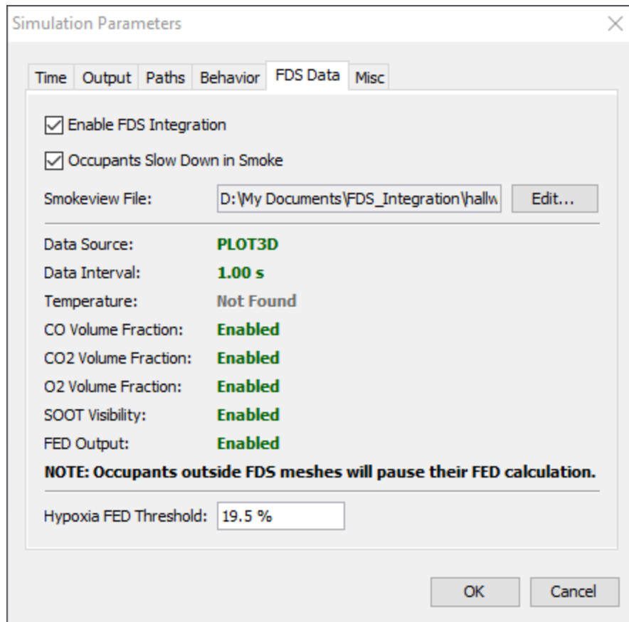
Figure 87. The Solution Parameters dialog after enabling FDS Integration.
