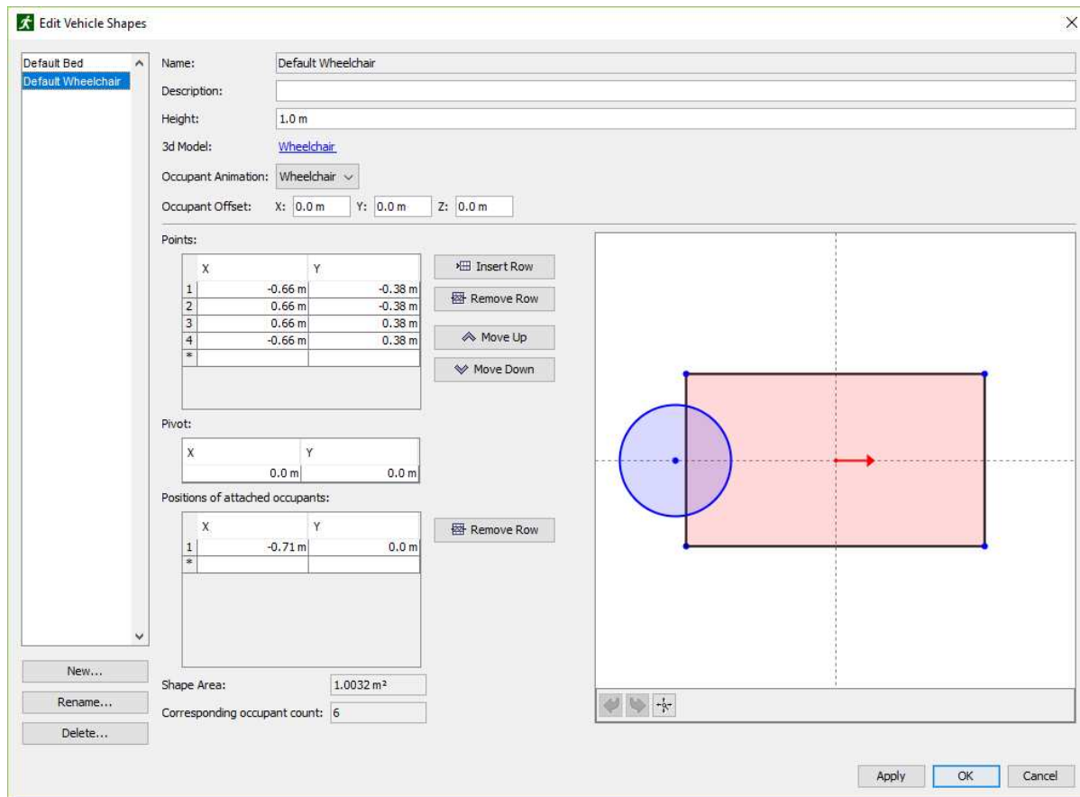
Figure 96. The Edit Vehicle Shapes Dialog
