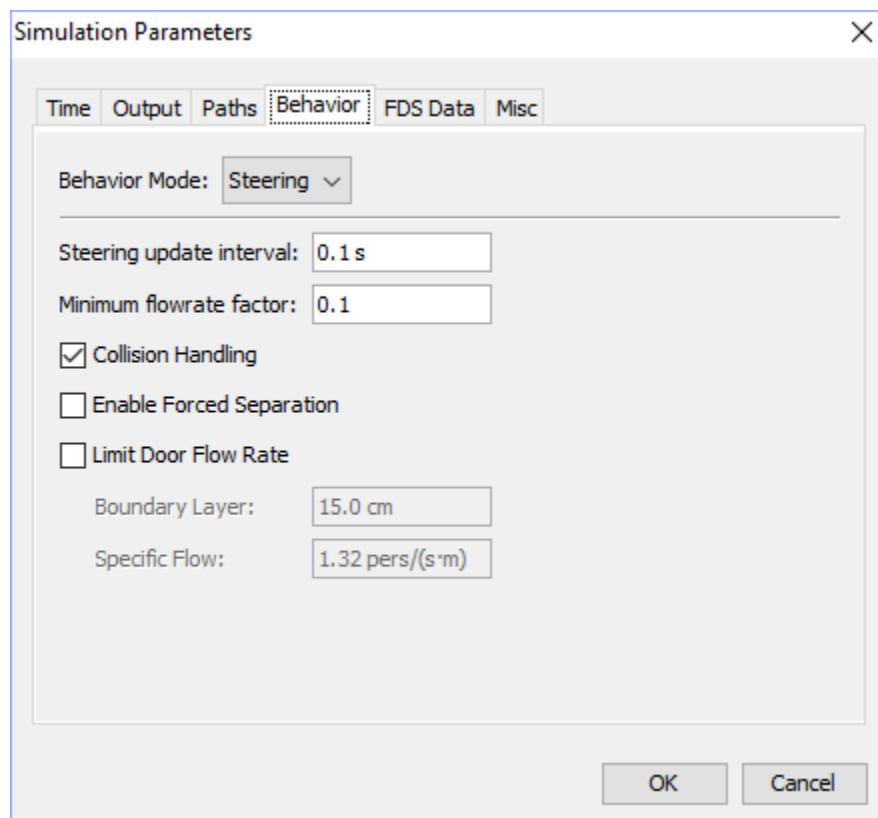
Figure 147. The Steering Behavior tab of the Simulation Parameters dialog
