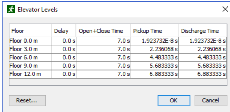
Figure 64. Elevator Levels dialog
