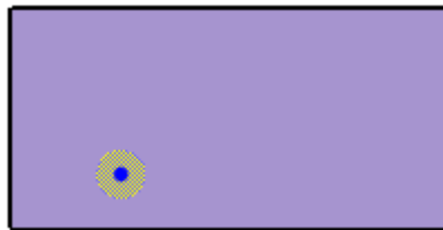
Figure 148. Occupant handle
