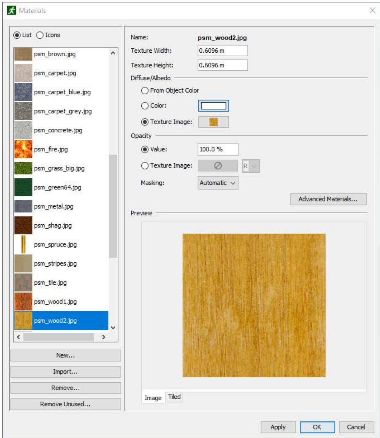
Figure 94. Materials dialog
