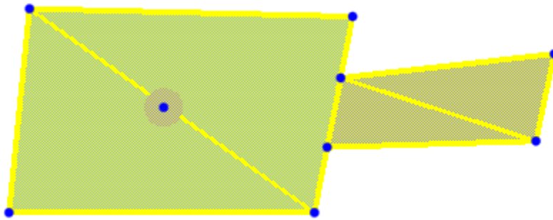
Figure 143. Manipulator handles
