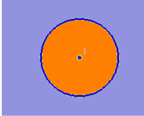
Figure 149. Waypoint handles
