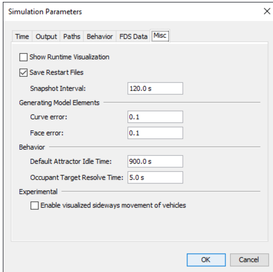
Figure 159. The Miscellaneous tab of the Simulation Parameters dialog
