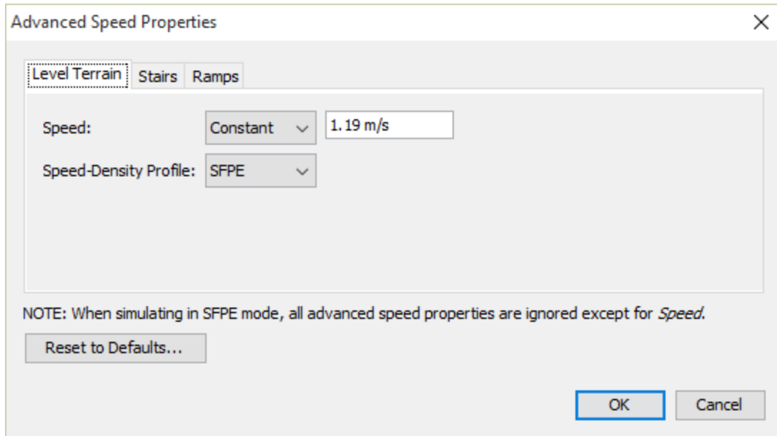
Figure 103. Advanced Speed Properties dialog
