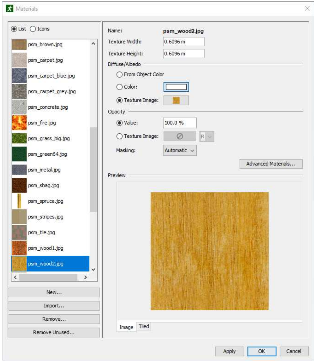
Figure 96. Materials dialog
