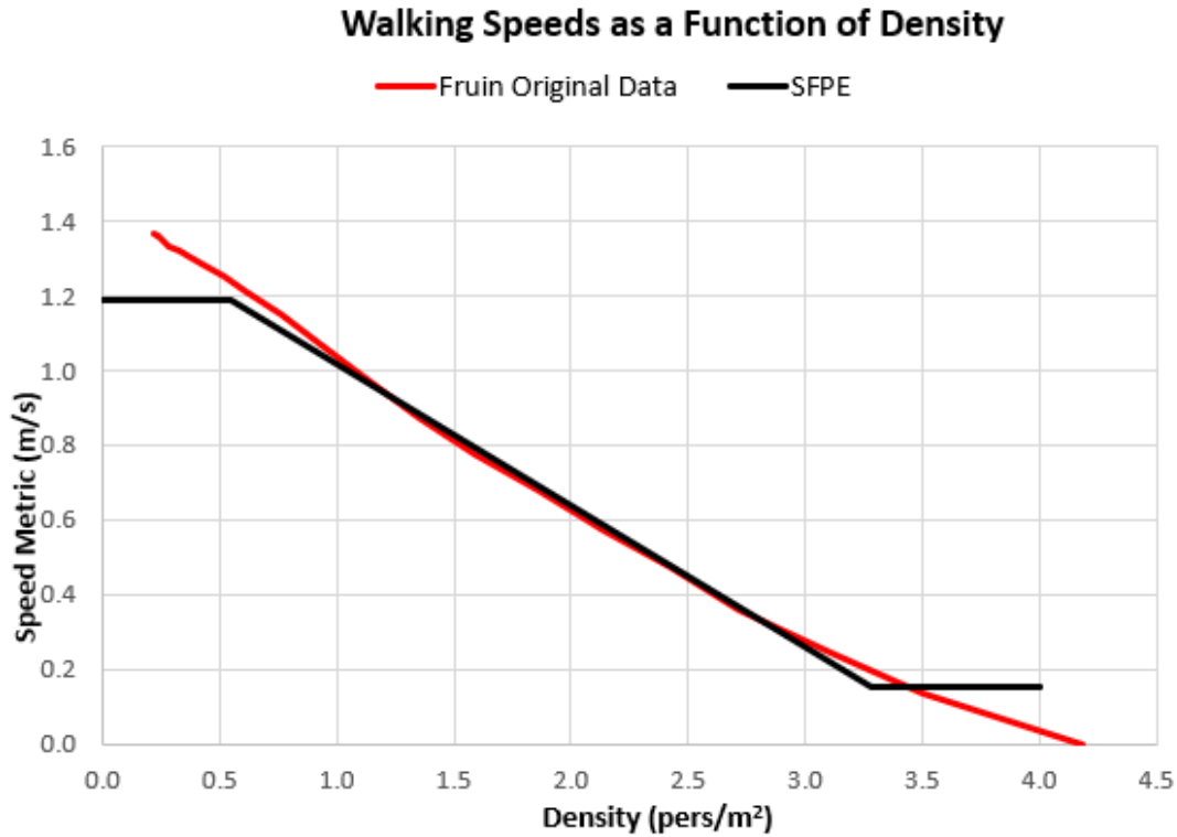
Figure 166. Graph of Walking Speeds as a Function of Density from Fruin
