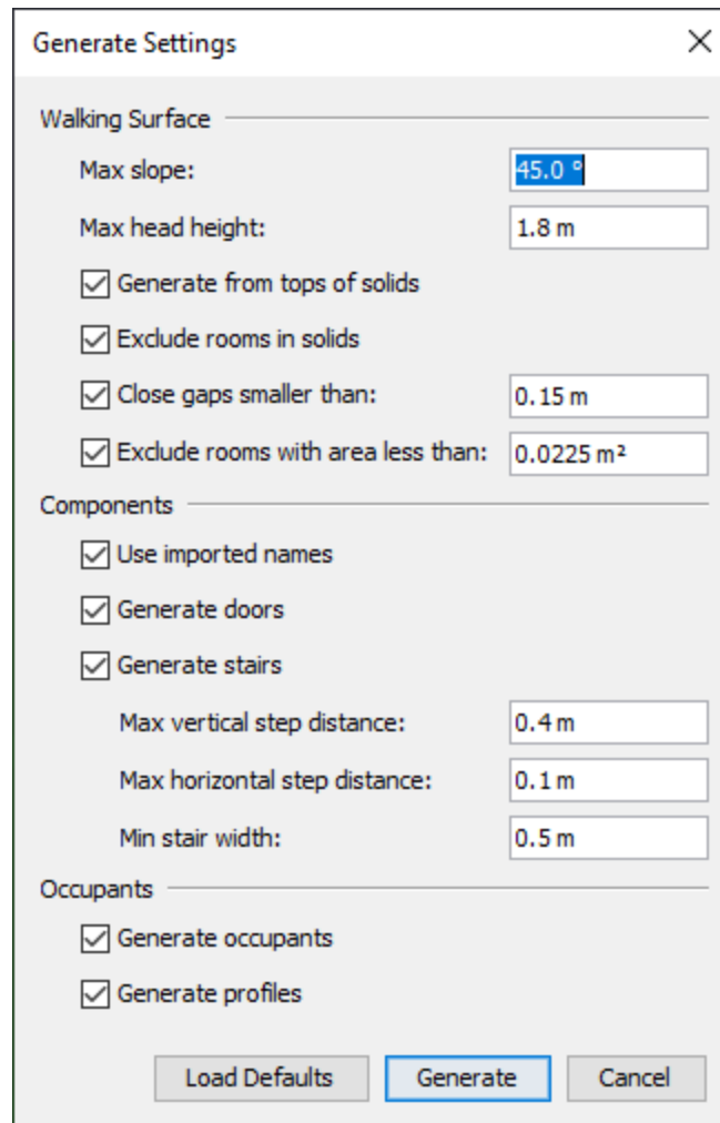
Figure 84. Generate Settings dialog
