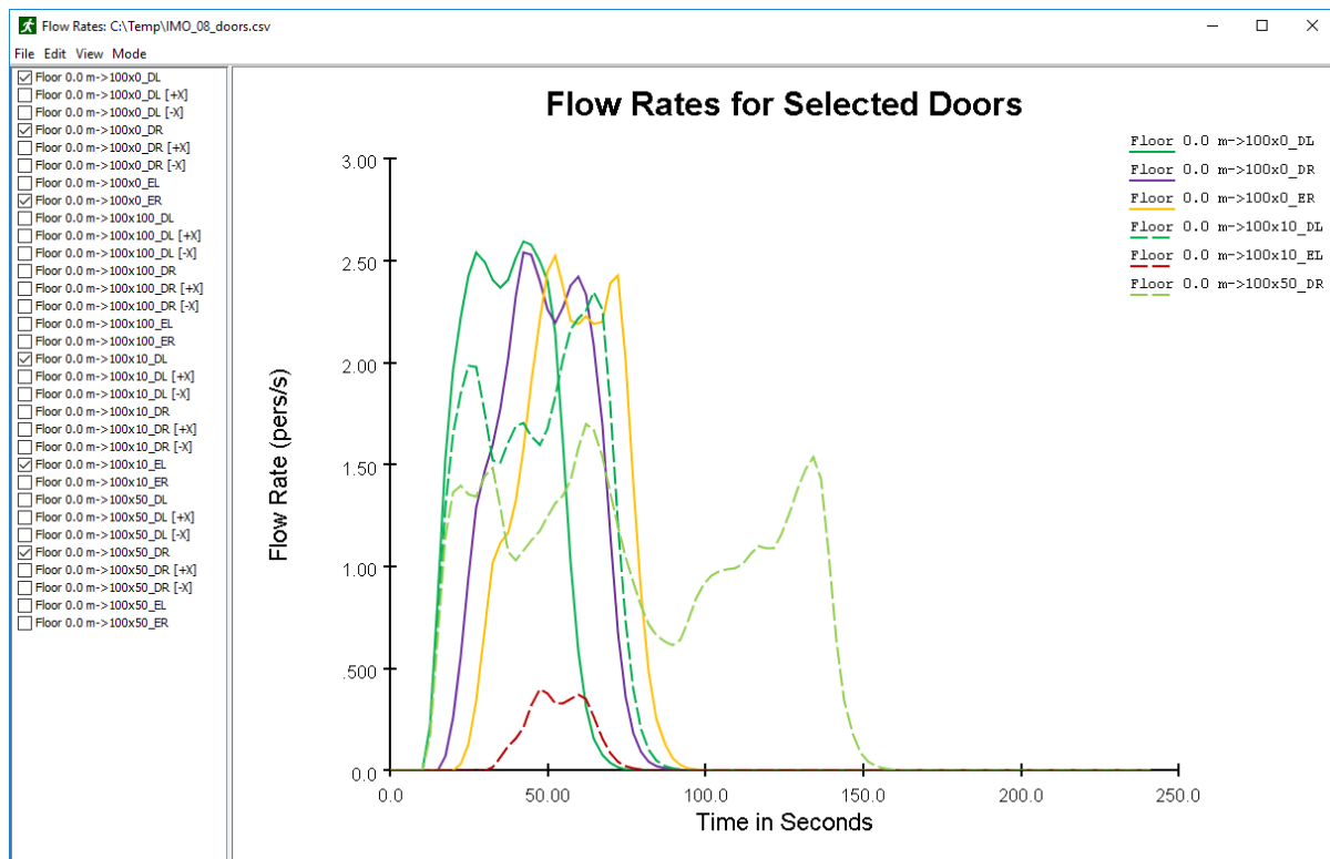
Figure 163. A time history plot for door flow rates
