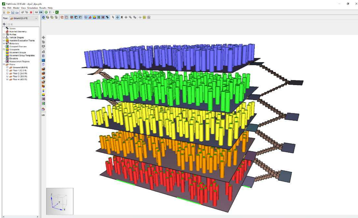
Figure 144. SFPE Example 2 Problem Setup
