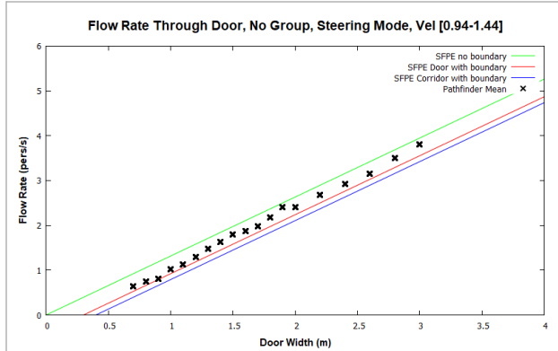
Figure 60. Door flow rates without grouping.
