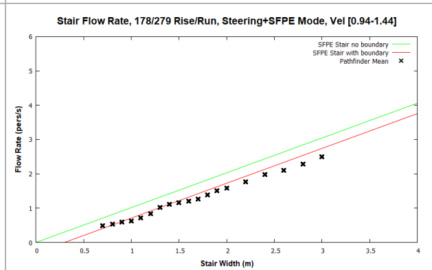
Figure 46. Stair flow rates for Steering+SFPE mode and occupants with a max speed distribution of 1.19 ± 0.25 m/s.
