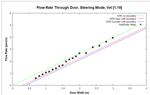
Figure 37. Door flow rates for Steering mode and occupants with a max speed of 1.19 m/s.
