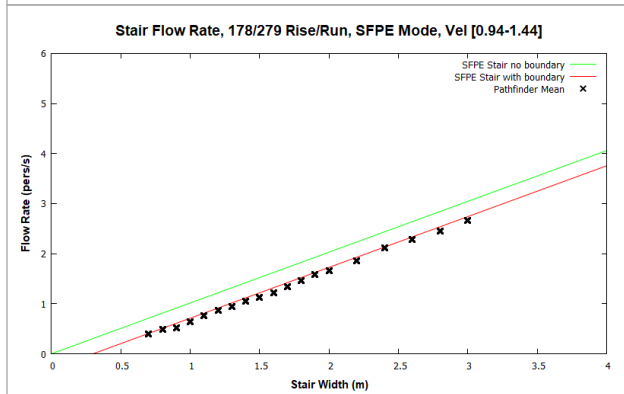
Figure 45. Stair flow rates for SFPE mode and occupants with a max speed distribution of 1.19 ± 0.25 m/s.
