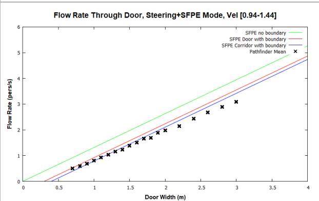
Figure 40. Door flow rates for Steering+SFPE mode and occupants with a max speed distribution of 1.19 ± 0.25 m/s.
