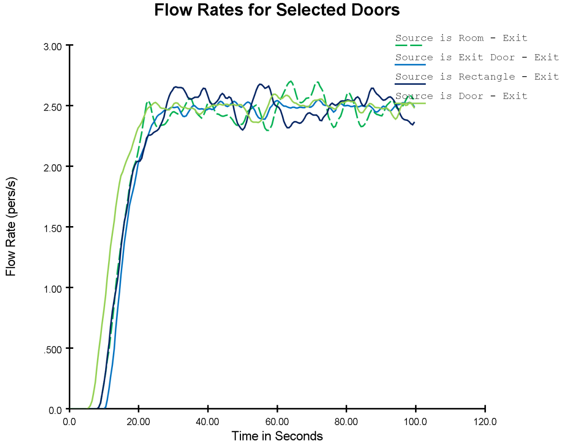
Figure 99. Exit door flow rates for the different source types.
