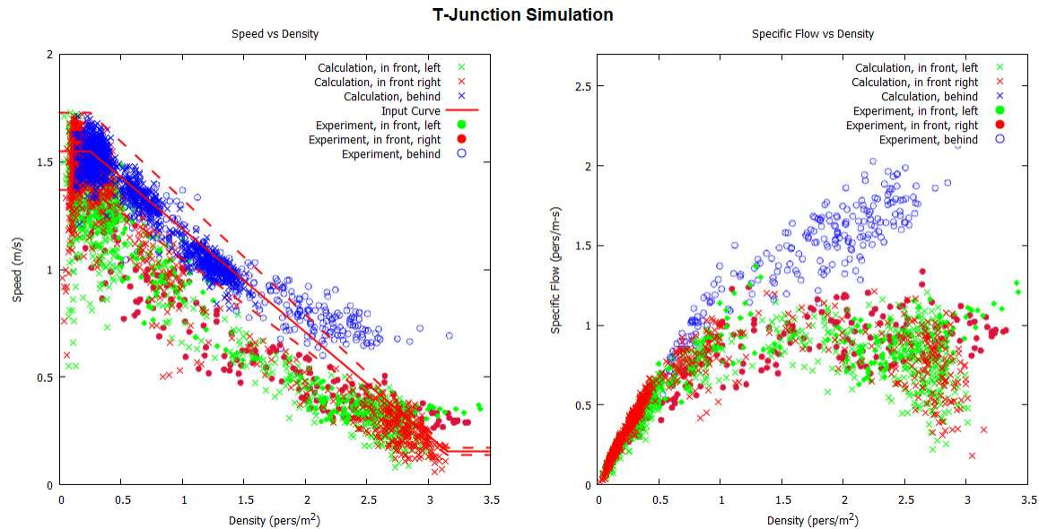
Figure 25. Speed-density results for Zhang and Seyfried experiment with measured speed-density input and uniform velocity distribution 1.55 \pm 0.18 m/s.
