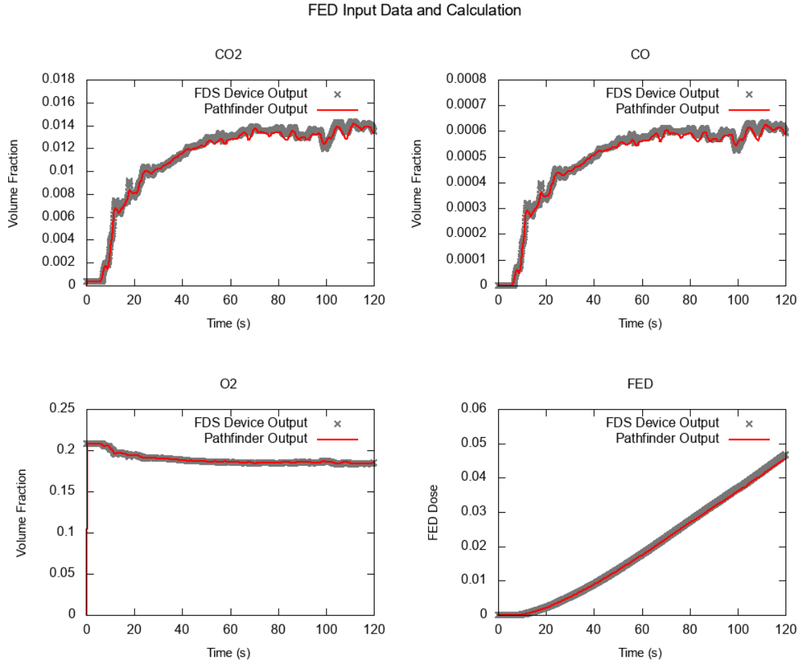
Figure 102. Comparison of FDS device output and Pathfinder input and FED calculation.
