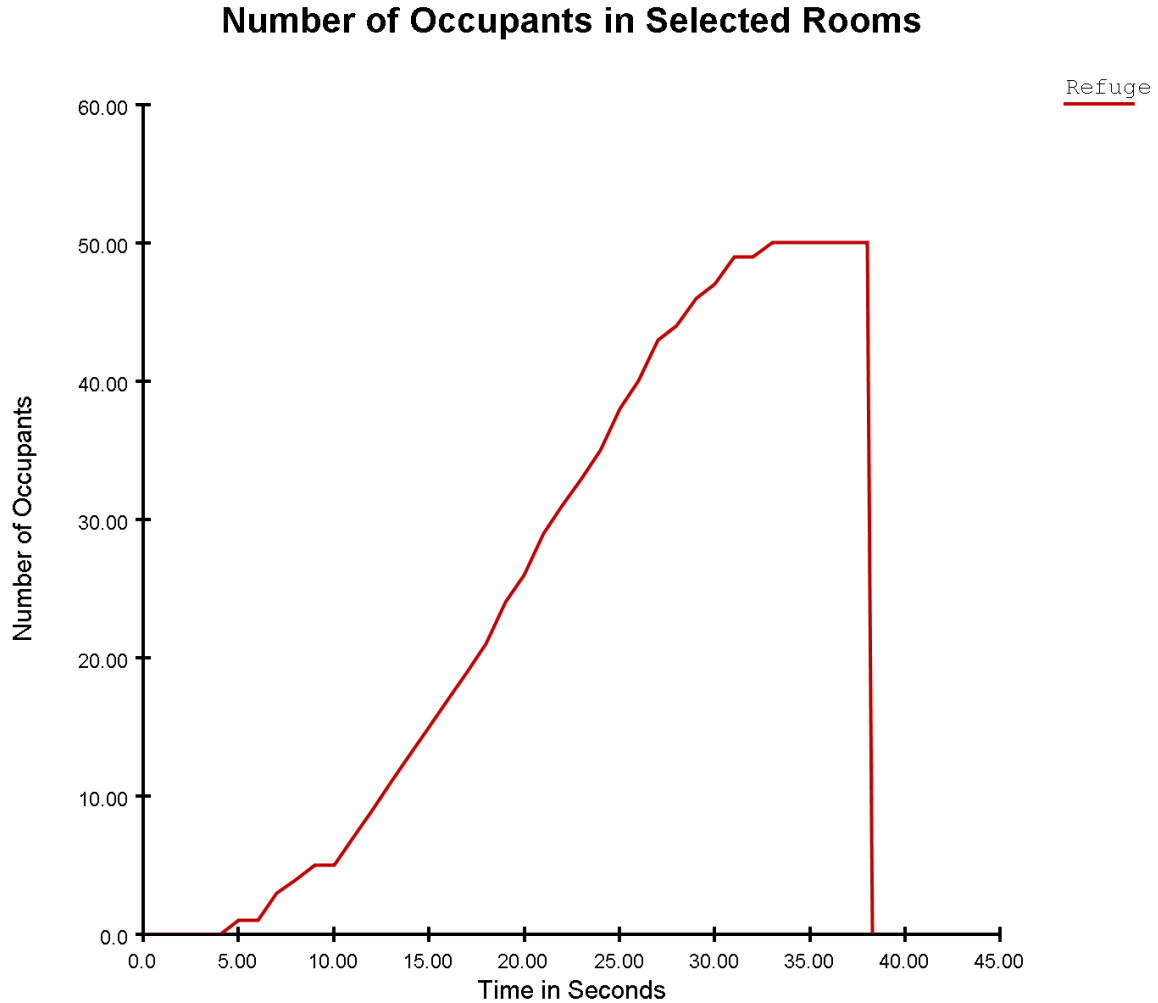
Figure 58. Occupants in the refuge room. Steering mode simulation.
