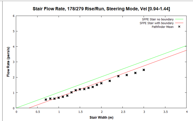
Figure 44. Stair flow rates for Steering mode and occupants with a max speed distribution of 1.19 ± 0.25 m/s.
