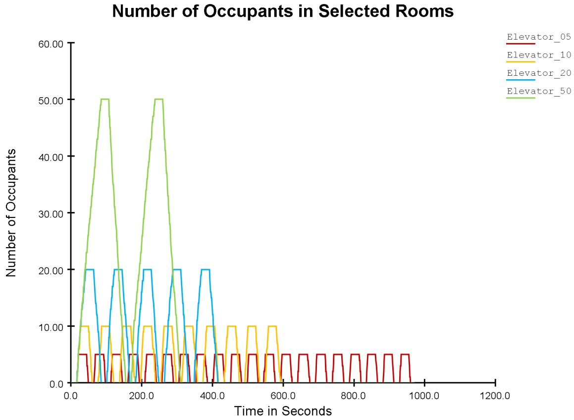
Figure 84. Observed elevator loading for steering mode
