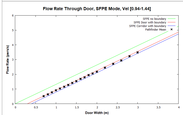
Figure 39. Door flow rates for SFPE mode and occupants with a max speed distribution of 1.19 ± 0.25 m/s.
