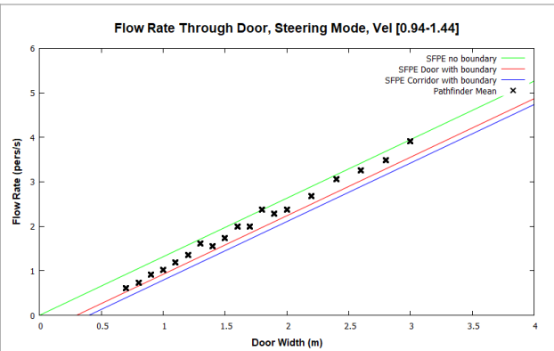
Figure 38. Door flow rates for Steering mode and occupants with a max speed distribution of 1.19 ± 0.25 m/s.
