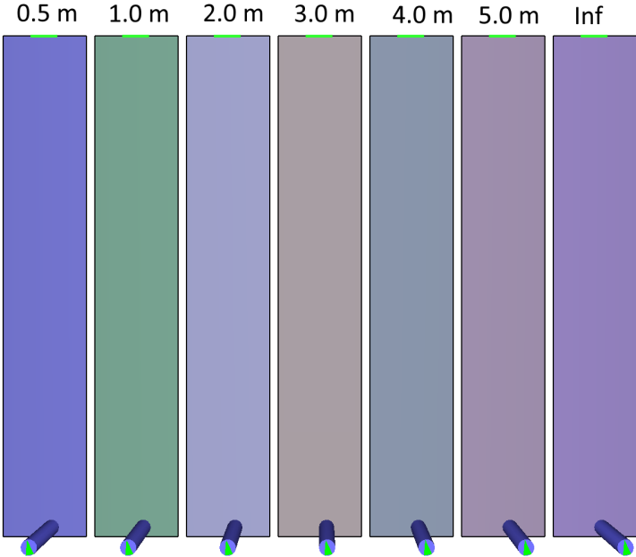
Figure 123. Pathfinder model to calculate speed in smoke. The values indicate visibility in the different rooms.
