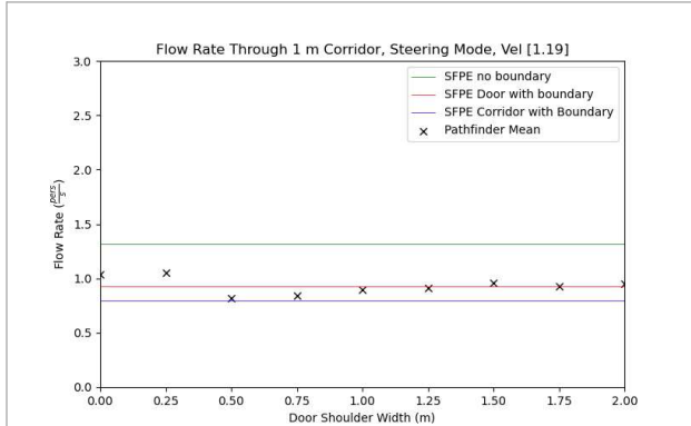
Figure 55. Corridor flow rates for 1 m corridor in Steering Mode with varying entry shoulder widths. Occupants have a constant max speed of 1.19 m/s.
