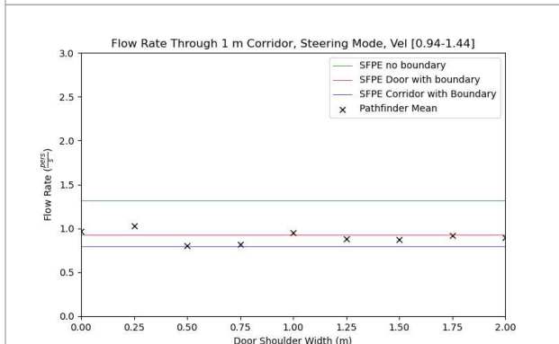
Figure 57. Corridor flow rates for 1 m corridor in Steering Mode with varying entry shoulder widths. Occupants have a max speed distribution of 1.19 \pm 0.25 m/s.
