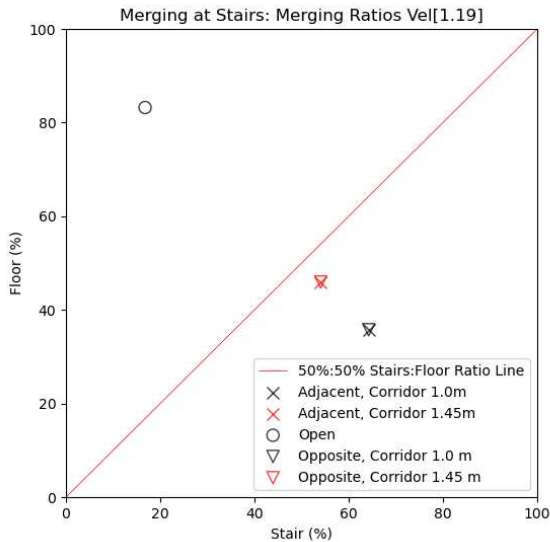
Figure 87. Merging ratios for stair merging with a constant maximum occupant speed of 1.19 m/s.
