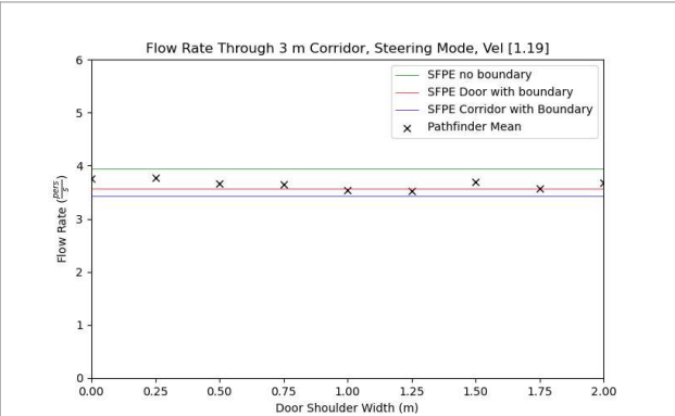
Figure 56. Corridor flow rates for 3 m corridor in Steering Mode with varying entry shoulder widths. Occupants have a constant max speed of 1.19 m/s.
