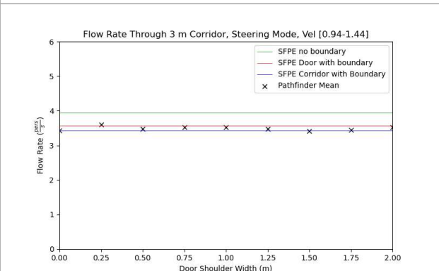
Figure 58. Corridor flow rates for 3 m corridor in Steering Mode with varying entry shoulder widths. Occupants have a max speed distribution of 1.19 \pm 0.25 m/s.
