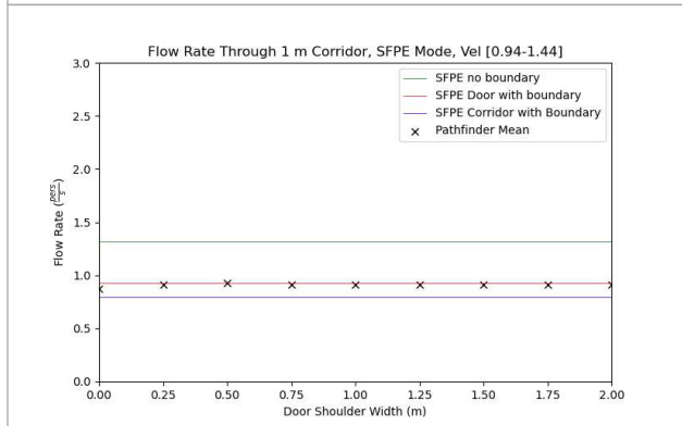
Figure 59. Corridor flow rates for 1 m corridor in SFPE Mode with varying entry shoulder widths. Occupants have a max speed distribution of 1.19 \pm 0.25 m/s.
