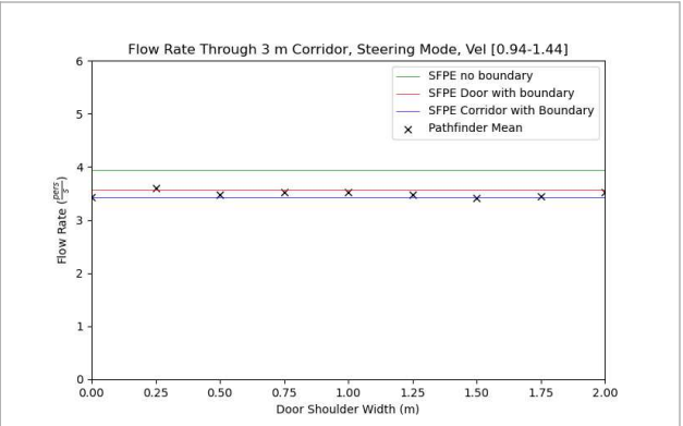
Figure 58. Corridor flow rates for 3 m corridor in Steering Mode with varying entry shoulder widths. Occupants have a max speed distribution of 1.19 \pm 0.25 m/s.
