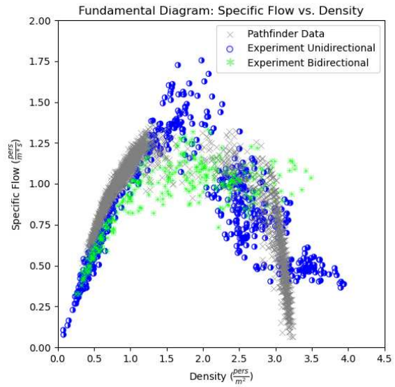
Figure 8. Specific Flow-Density results with measured speed-density input and uniform velocity distribution 1.55 \pm 0.18 m/s.
