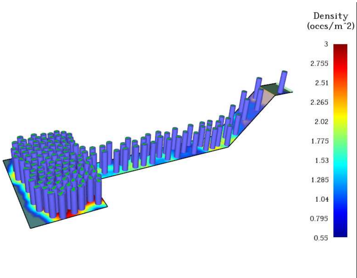
Figure 147. Visual demonstration of congestion at base of stairs.
