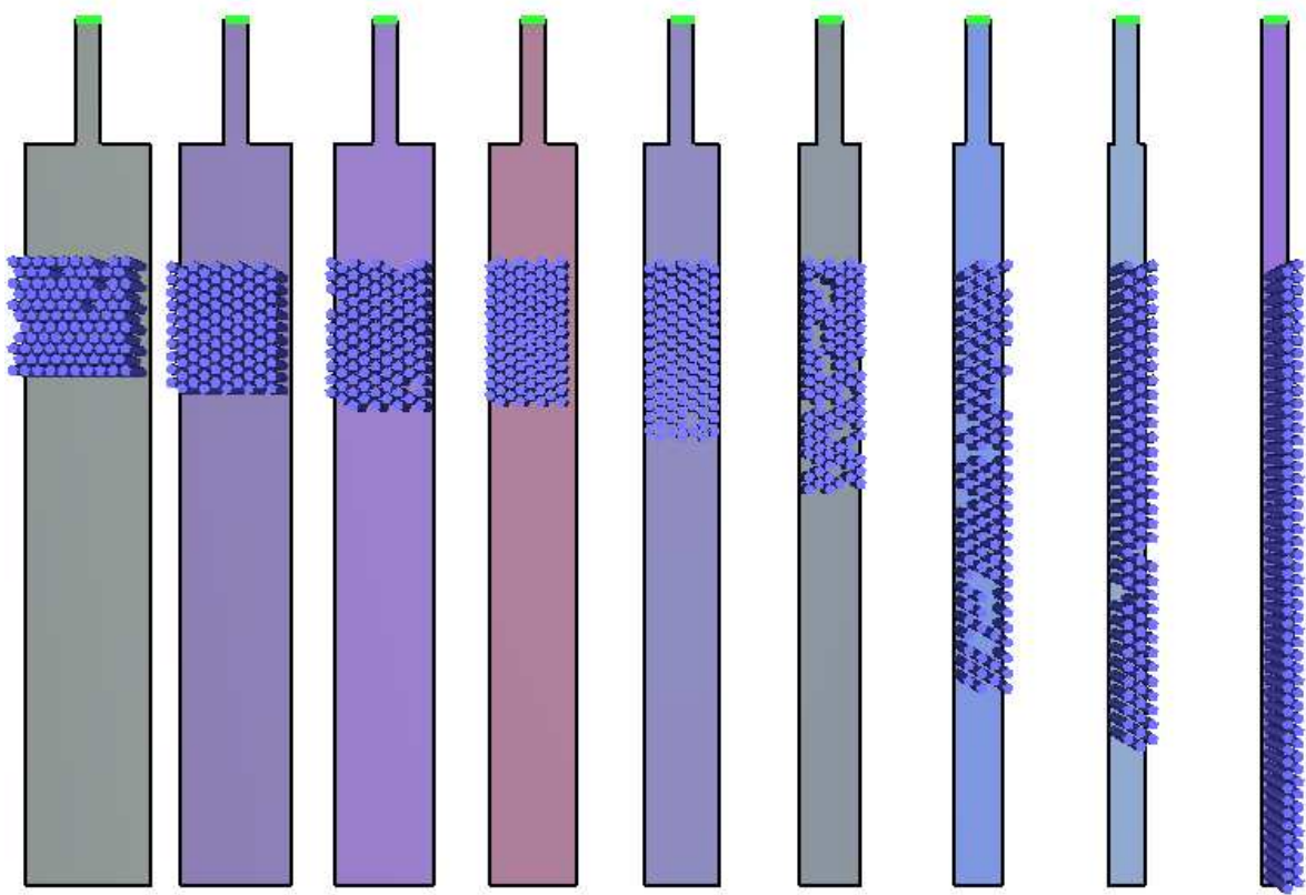
Figure 53. Pathfinder model used to study 1\text{ m} wide corridor flow rates.
