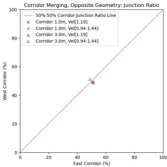
Figure 77. Merging ratios for merging at a corridor junction with "opposite" configuration.
