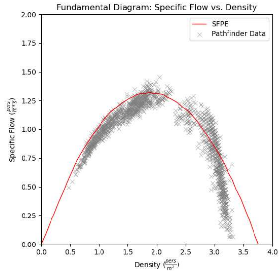
Figure 12. Specific Flow-Density results with SFPE speed-density input and uniform velocity distribution 1.19 \pm 0.25 m/s.
