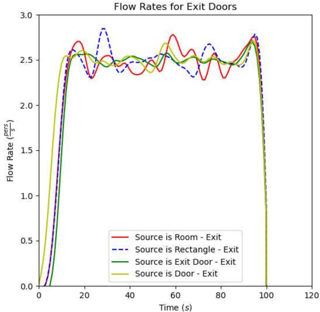
Figure 109. Exit door flow rates for the different source types.
