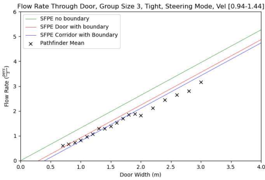
Figure 68. Door flow rates for steering mode with default parameters and tight group of size 3.
