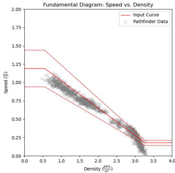
Figure 11. Speed-Density results with SFPE speed-density input and uniform velocity distribution 1.19 \pm 0.25 m/s.
