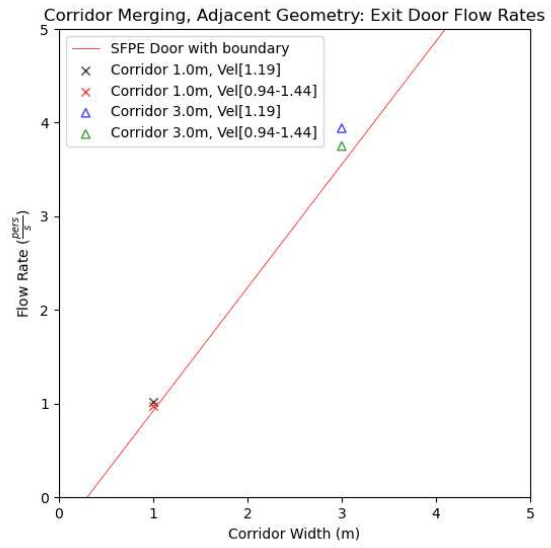
Figure 76. Exit door flow rates for merging at a corridor junction with "adjacent" configuration.
