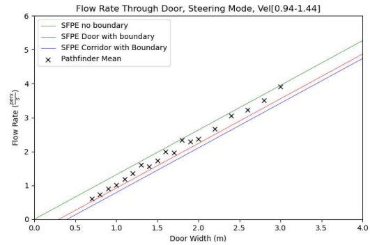
Figure 44. Door flow rates for Steering mode and occupants with a max speed distribution of 1.19 ± 0.25 m/s.
