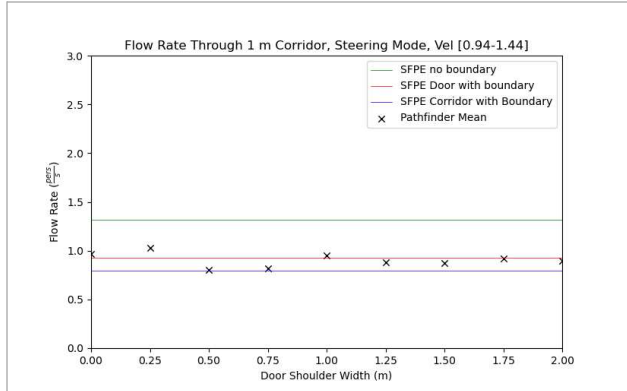
Figure 57. Corridor flow rates for 1 m corridor in Steering Mode with varying entry shoulder widths. Occupants have a max speed distribution of 1.19 \pm 0.25 m/s.
