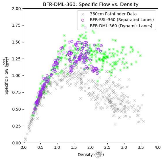
Figure 23. Specific Flow-Density results with assigned destination, unidirectional speed-density input, and uniform velocity distribution 1.55 \pm 0.18 m/s.
