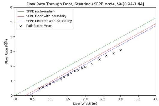
Figure 46. Door flow rates for Steering+SFPE mode and occupants with a max speed distribution of 1.19 ± 0.25 m/s.
