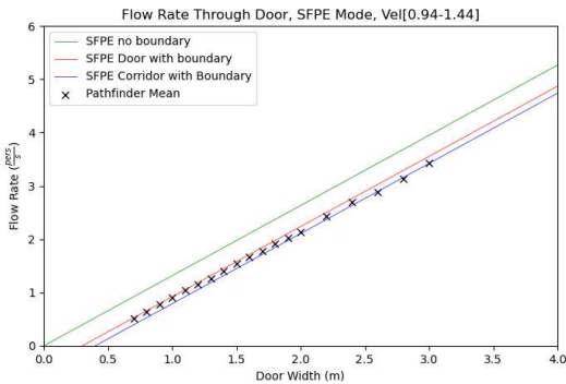
Figure 45. Door flow rates for SFPE mode and occupants with a max speed distribution of 1.19 ± 0.25 m/s.
