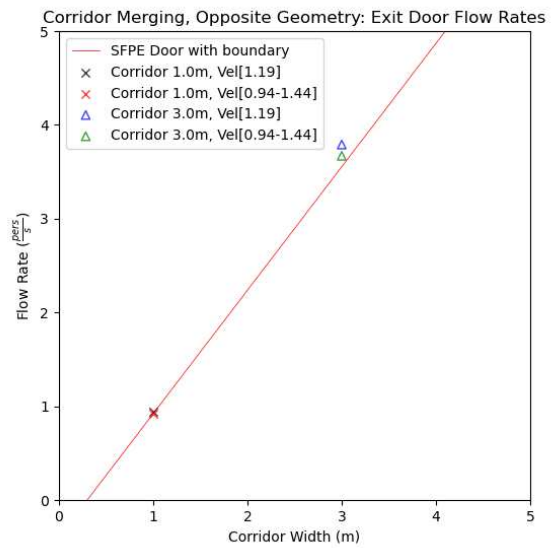
Figure 78. Exit door flow rates for merging at a corridor junction with "opposite" configuration.
