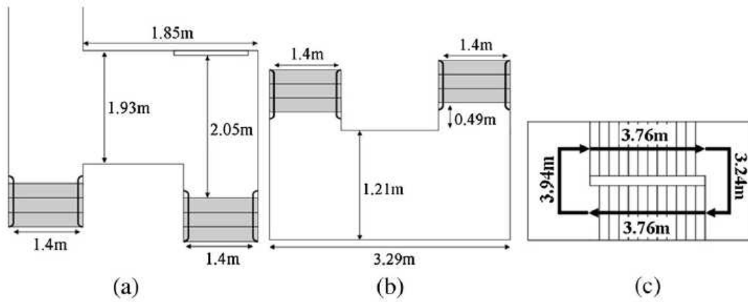
Figure 4. Stair dimensions.
