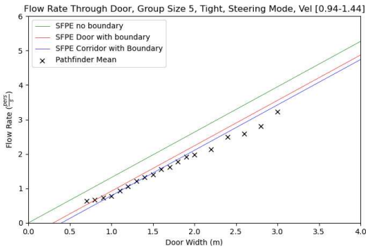
Figure 70. Door flow rates for steering mode with default parameters and tight group of size 5.
