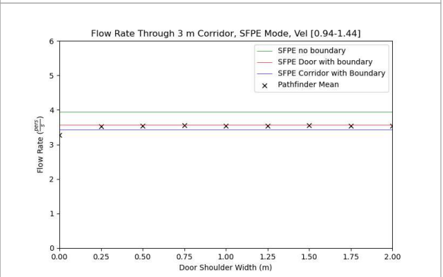
Figure 60. Corridor flow rates for 3 m corridor in SFPE Mode with varying entry shoulder widths. Occupants have a max speed distribution of 1.19 \pm 0.25 m/s.
