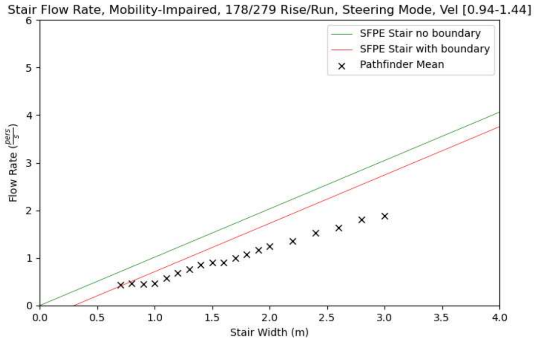
Figure 92. Stair flow rates for Steering mode, 90 percent of occupants have a max speed distribution of 1.19 \pm 0.25 m/s, 10 percent have a constant speed of 0.5 m/s.
