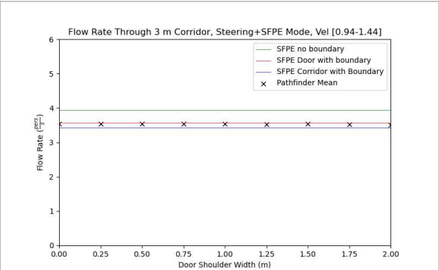
Figure 62. Corridor flow rates for 3 m corridor in Steering+SFPE Mode with varying entry shoulder widths. Occupants have a max speed distribution of 1.19 \pm 0.25 m/s.
