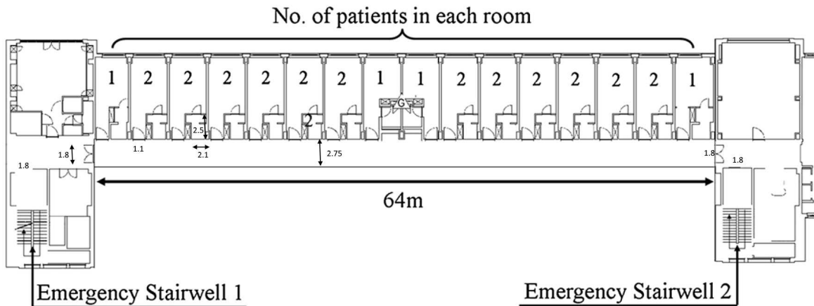
Figure 103. Geometry of floor 11 with patients (Hunt, Galea, and Lawrence 2013).
