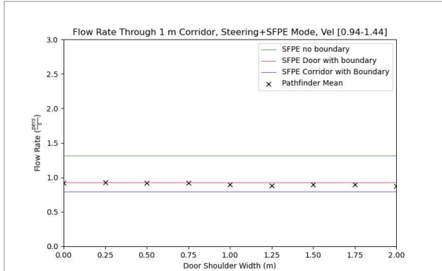
Figure 61. Corridor flow rates for 1 m corridor in Steering+SFPE Mode with varying entry shoulder widths. Occupants have a max speed distribution of 1.19 \pm 0.25 m/s.
