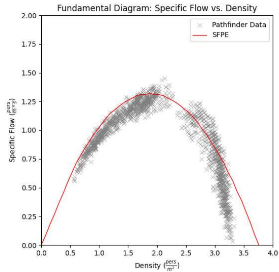
Figure 12. Specific Flow-Density results with SFPE speed-density input and uniform velocity distribution
