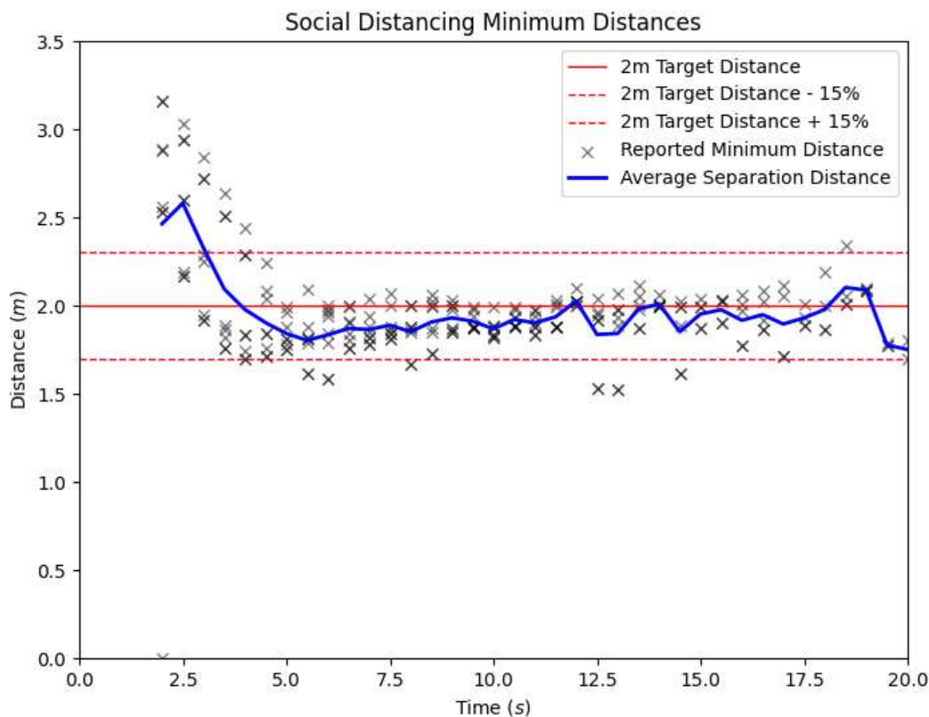
Figure 124. Social Distancing Test Results
