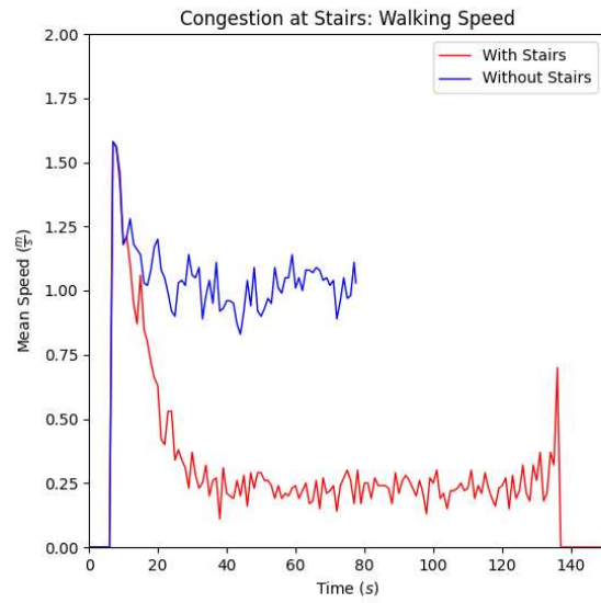
Figure 148. Comparison of walking speeds at base of stairs with and without stairs.
