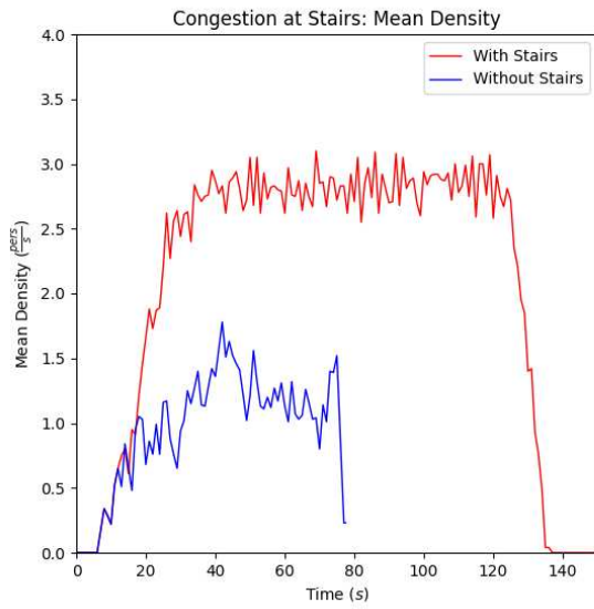
Figure 147. Comparison of mean density at base of stairs with and without stairs.
