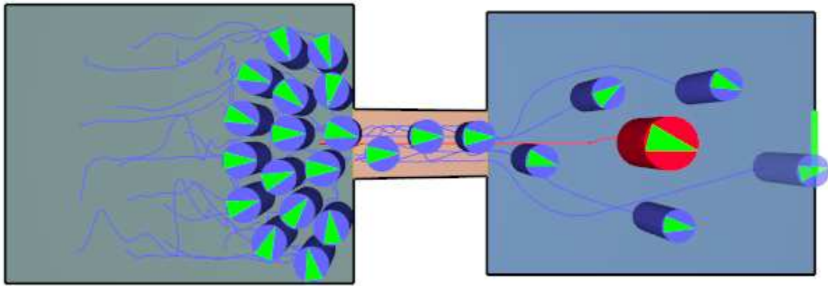
Figure 161. Steering mode showing how faster occupants move around disabled occupant past ramp. Lines show paths.
