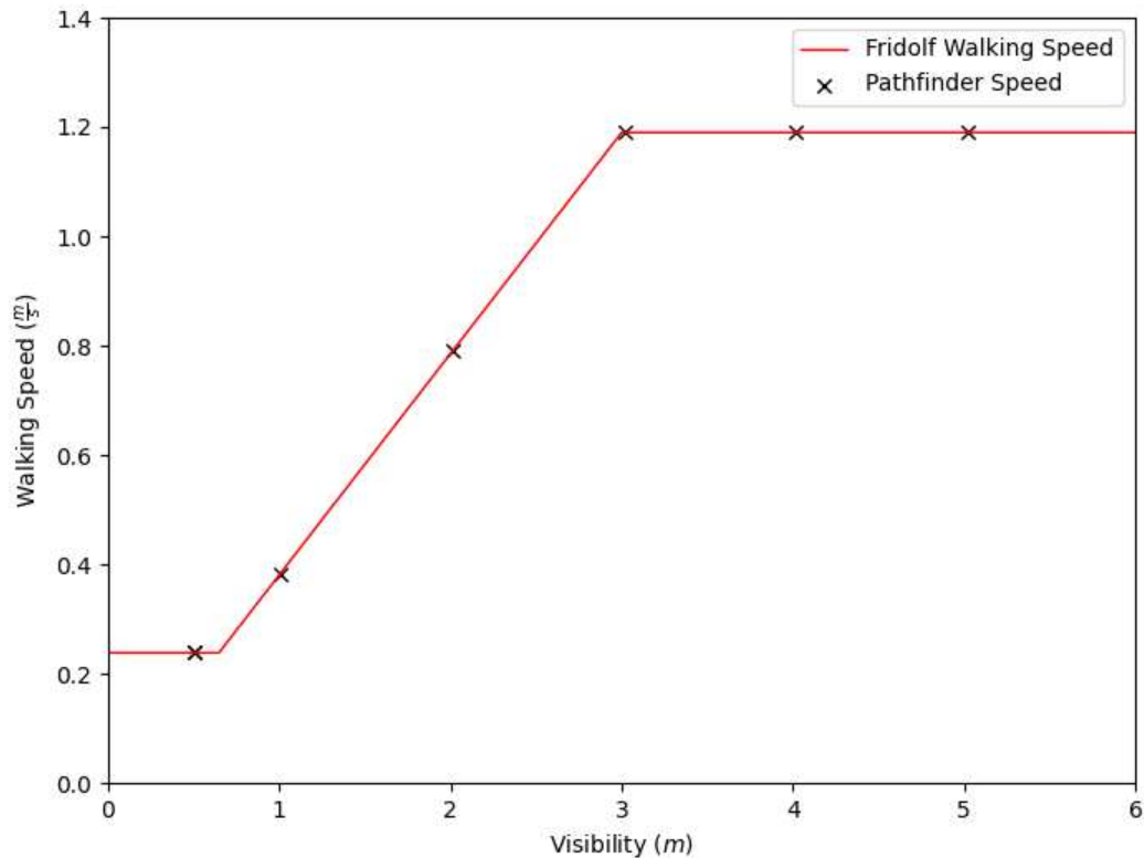
Figure 123. Comparison of expected and calculated speeds in smoke.
