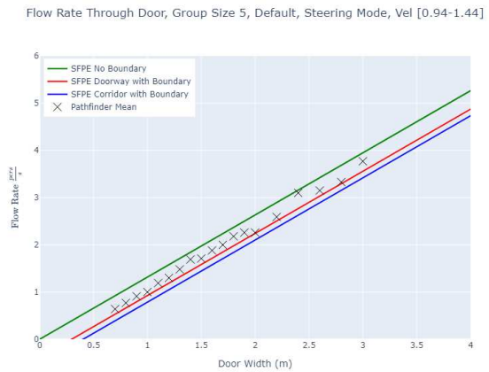
Figure 69. Door flow rates for steering mode with default parameters and group of size 5.
