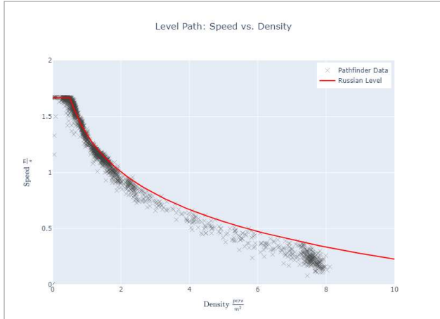
Figure 37. Speed-density results for Russian evacuation simulation, level path.
