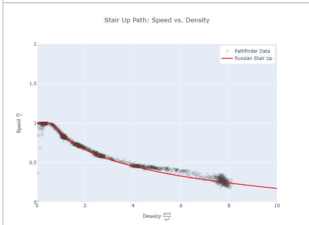
Figure 39. Speed-density results for Russian evacuation simulation, stairs up.
