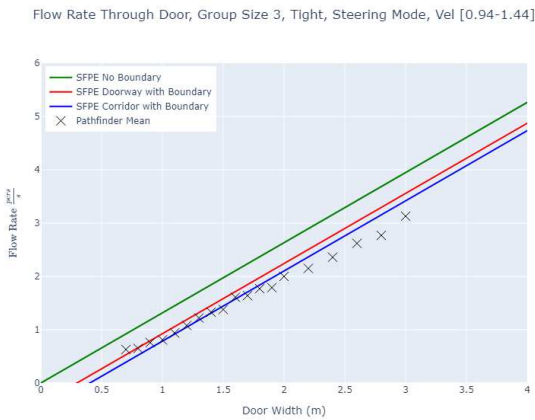
Figure 68. Door flow rates for steering mode with default parameters and tight group of size 3.
