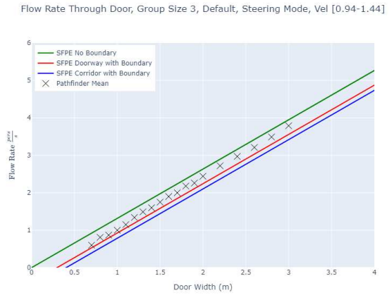
Figure 67. Door flow rates for steering mode with default parameters and group of size 3.
