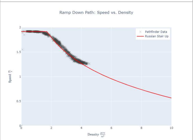
Figure 40. Speed-density results for Russian evacuation simulation, ramp down.
