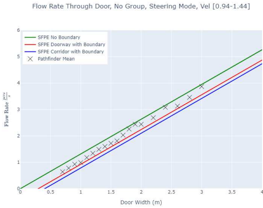
Figure 66. Door flow rates without grouping.
