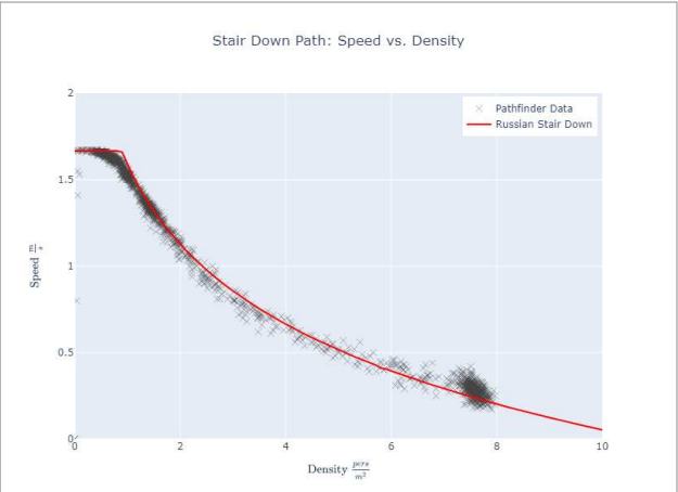
Figure 38. Speed-density results for Russian evacuation simulation, stairs down.
