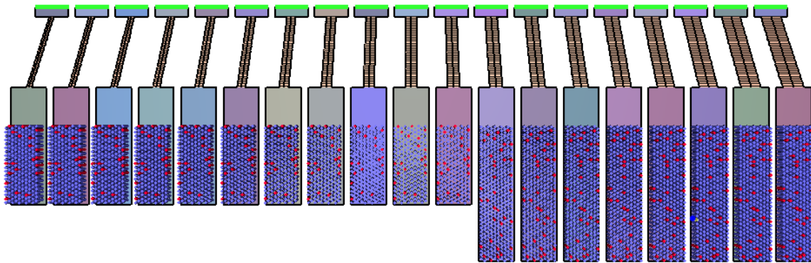
Figure 91. Pathfinder model used to study stair flow rates with mobility-impaired occupants (red).
