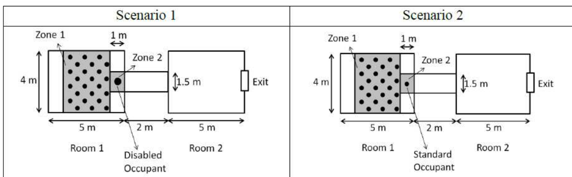
Figure 158. Geometry of movement disabilities verification (Verif.2.10). Figure from NIST Technical Note 1822, 2013.
