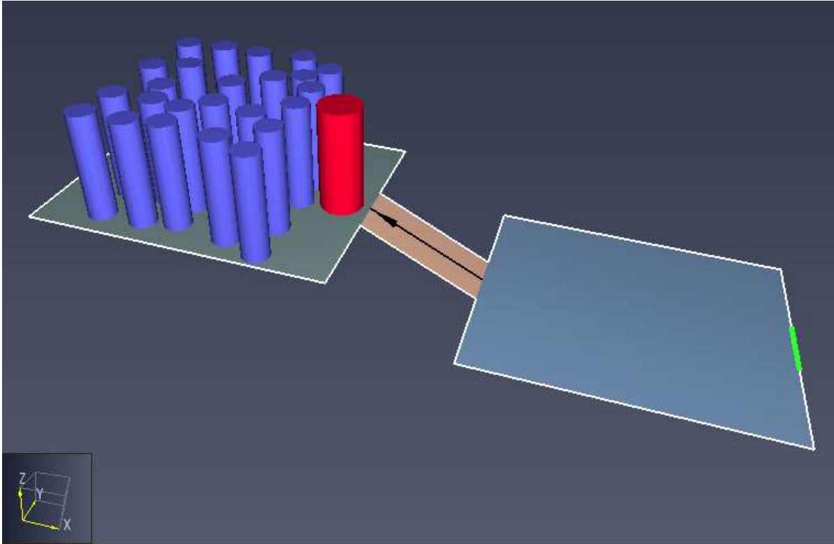
Figure 159. Pathfinder model of movement with disabilities. Red occupant has disabilities.
