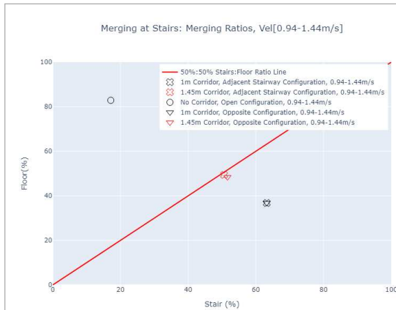
Figure 89. Merging ratios for stair merging with a uniformly distributed maximum occupant speed of 1.19 \pm 0.25 m/s.
