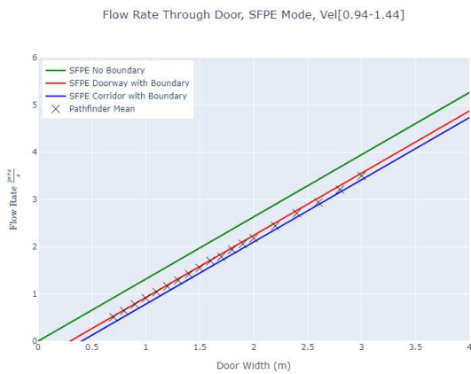
Figure 45. Door flow rates for SFPE mode and occupants with a max speed distribution of 1.19 \pm 0.25 m/s.
