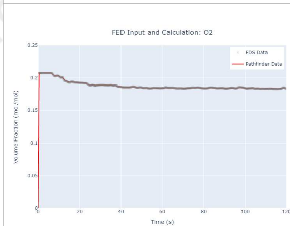
Figure 114. FDS device output vs Pathfinder Input: O2
