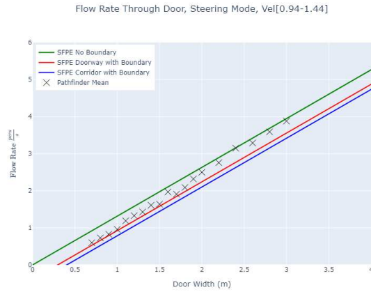
Figure 44. Door flow rates for Steering mode and occupants with a max speed distribution of 1.19 \pm 0.25 m/s.
