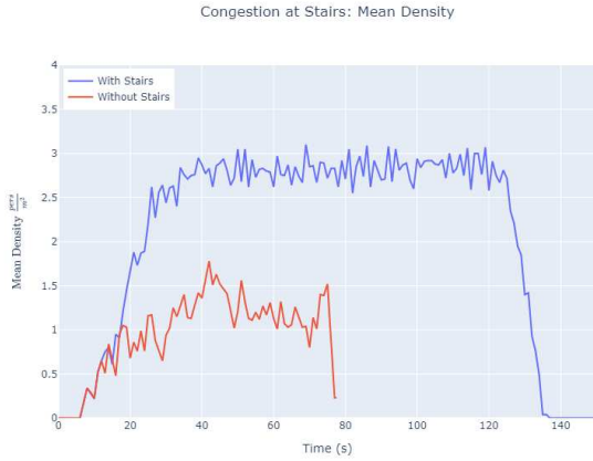
Figure 147. Comparison of mean density at base of stairs with and without stairs.
