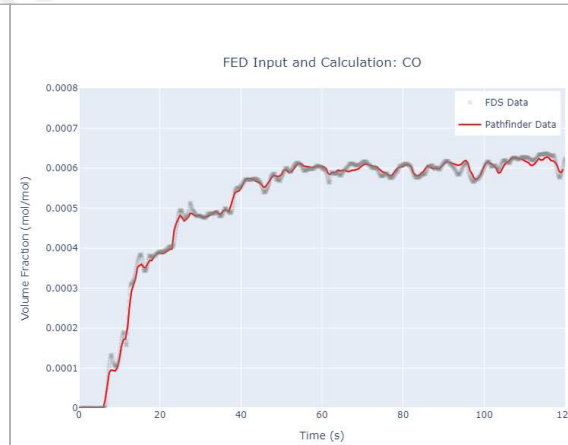
Figure 113. FDS device output vs Pathfinder Input: CO
