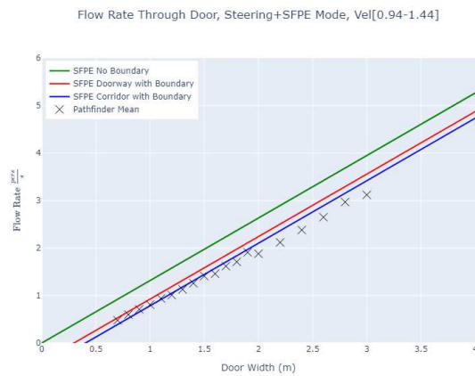
Figure 46. Door flow rates for Steering+SFPE mode and occupants with a max speed distribution of 1.19 \pm 0.25 m/s.
