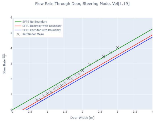
Figure 43. Door flow rates for Steering mode and occupants with a max speed of 1.19 m/s.
