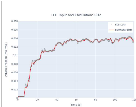
Figure 112. FDS device output vs Pathfinder Input: CO2
