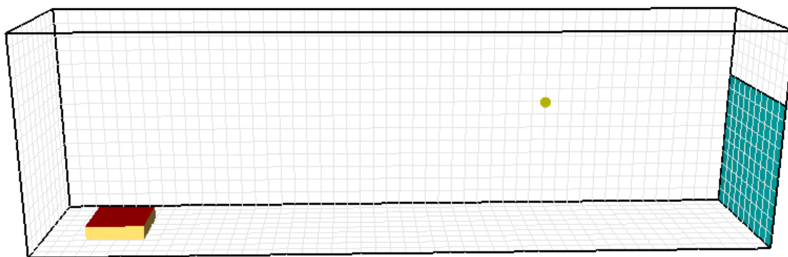
Figure 110. PyroSim model of FED calculation using stationary occupant.
