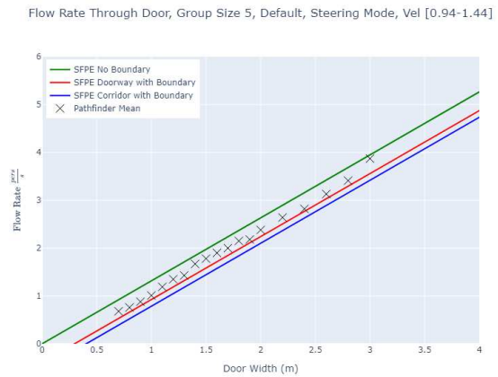
Figure 69. Door flow rates for steering mode with default parameters and group of size 5.
