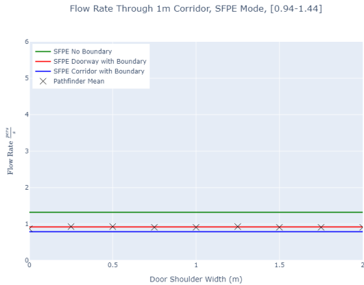
Figure 59. Corridor flow rates for 1 m corridor in SFPE Mode with varying entry shoulder widths. Occupants have a max speed distribution of 1.19 \pm 0.25 m/s.
