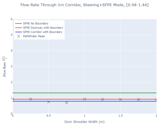
Figure 61. Corridor flow rates for 1 m corridor in Steering+SFPE Mode with varying entry shoulder widths. Occupants have a max speed distribution of 1.19 \pm 0.25 m/s.
