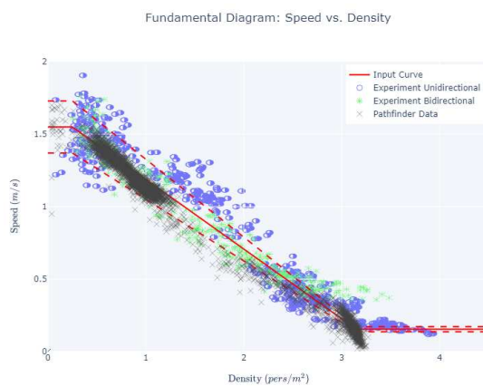
Figure 7. Speed-Density results with measured speed-density input and uniform velocity distribution 1.55 \pm 0.18 m/s.
