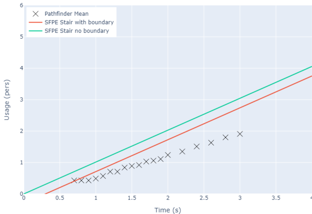
Figure 92. Stair flow rates for Steering mode, 90 percent of occupants have a max speed distribution of 1.19 \pm 0.25 m/s, 10 percent have a constant speed of 0.5 m/s.
