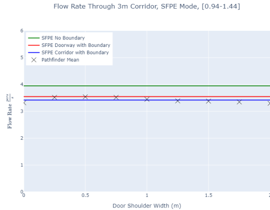
Figure 60. Corridor flow rates for 3 m corridor in SFPE Mode with varying entry shoulder widths. Occupants have a max speed distribution of 1.19 \pm 0.25 m/s.
