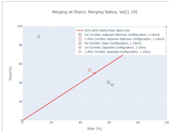
Figure 87. Merging ratios for stair merging with a constant maximum occupant speed of 1.19 m/s.
