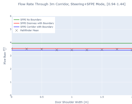
Figure 62. Corridor flow rates for 3 m corridor in Steering+SFPE Mode with varying entry shoulder widths. Occupants have a max speed distribution of 1.19 \pm 0.25 m/s.
