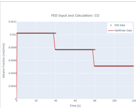
Figure 119. FDS device output vs Pathfinder Input: CO
