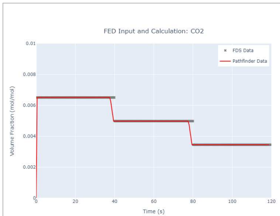
Figure 118. FDS device output vs Pathfinder Input: CO2
