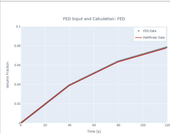
Figure 121. FDS device output vs Pathfinder Input: FED
