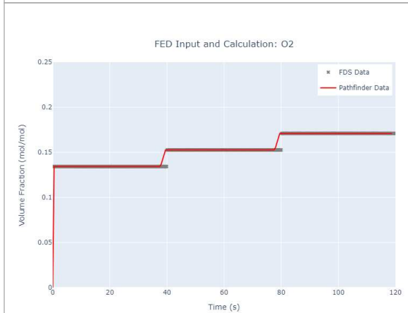
Figure 120. FDS device output vs Pathfinder Input: O2
