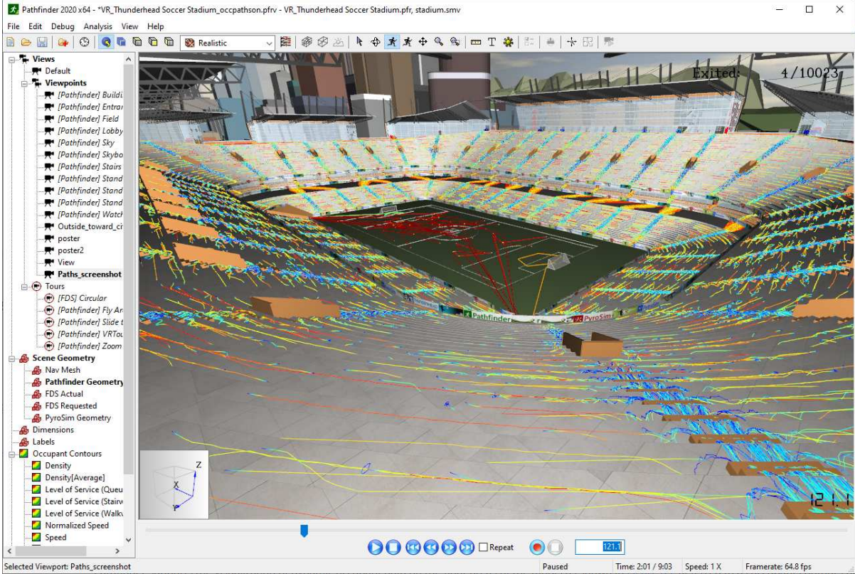
Figure 86. Occupant paths
