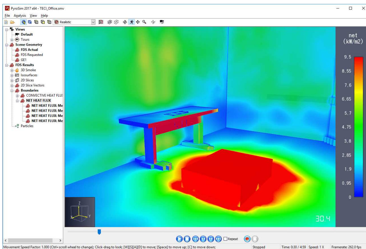
Figure 74. FDS Boundaries
