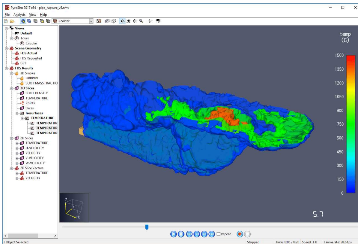
Figure 68. Data3D isosurfaces
