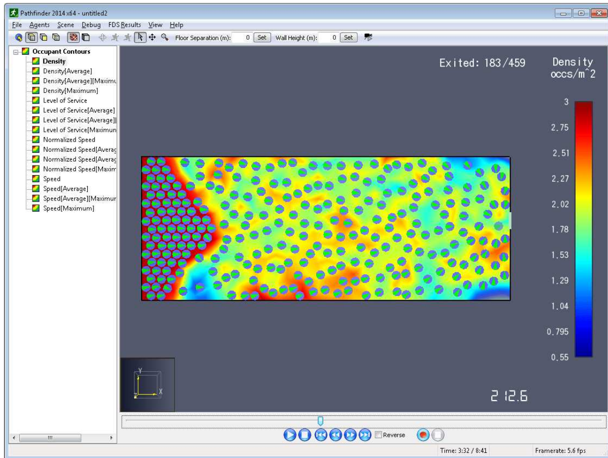
Figure 100. Occupant contours
