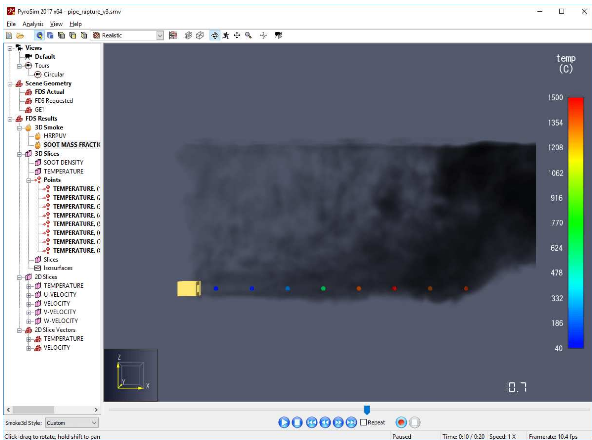
Figure 65. Data3D points
