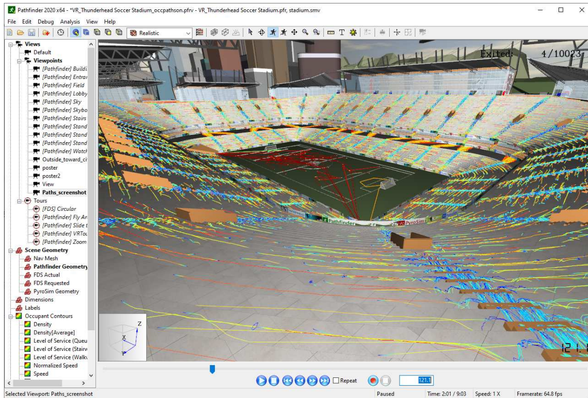
Figure 87. Occupant paths
