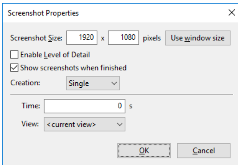
Figure 34. Screenshot dialog
