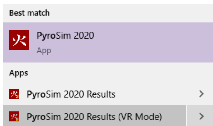
Figure 40. Shortcut Menu
