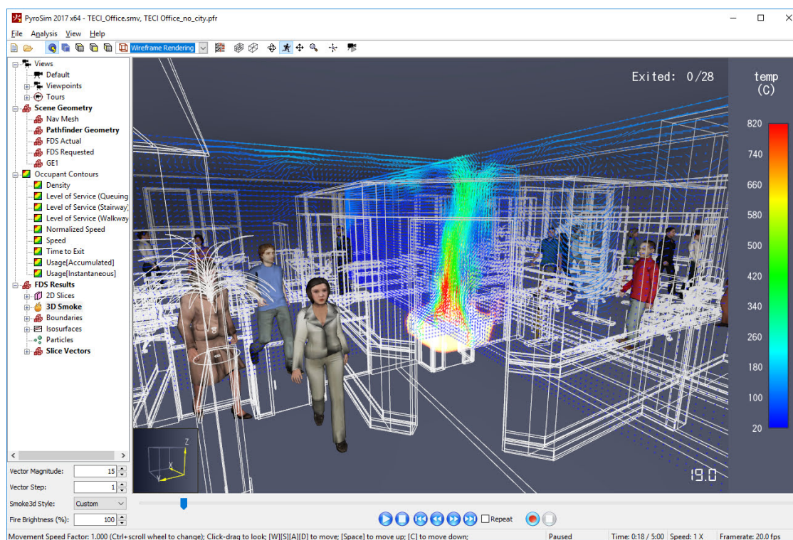
Figure 10. Wireframe Rendering
