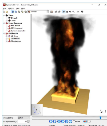
Figure 21. Compatibility Renderer
