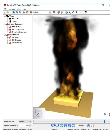
Figure 22. Smokeview Renderer
