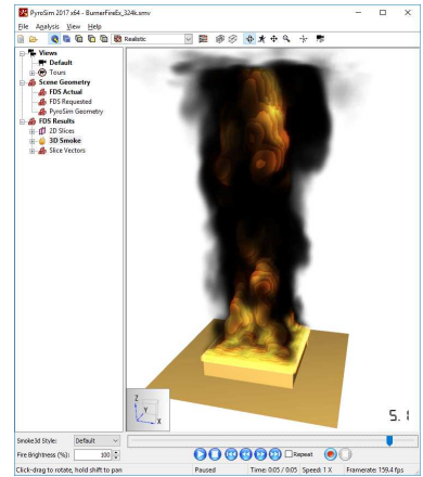
Figure 22. Smokeview Renderer
