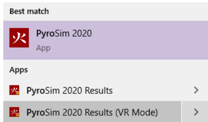
Figure 40. Shortcut Menu
