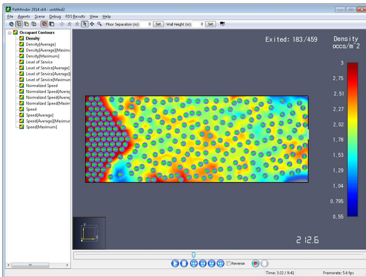
Figure 96. Occupant Contours
