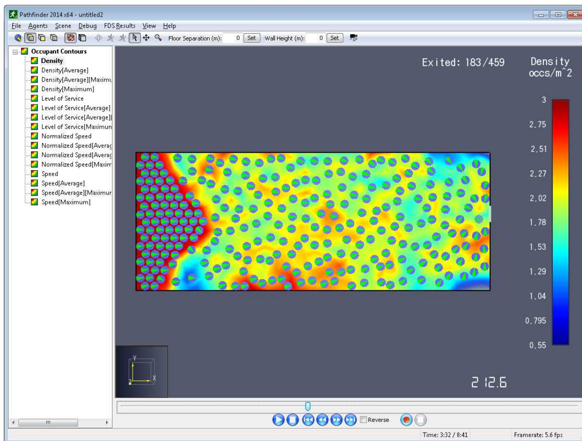
Figure 110. Occupant contours
