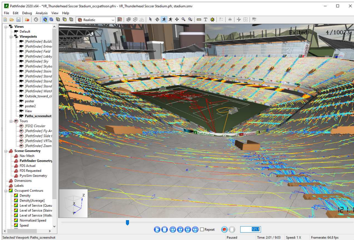
Figure 95. Occupant paths
