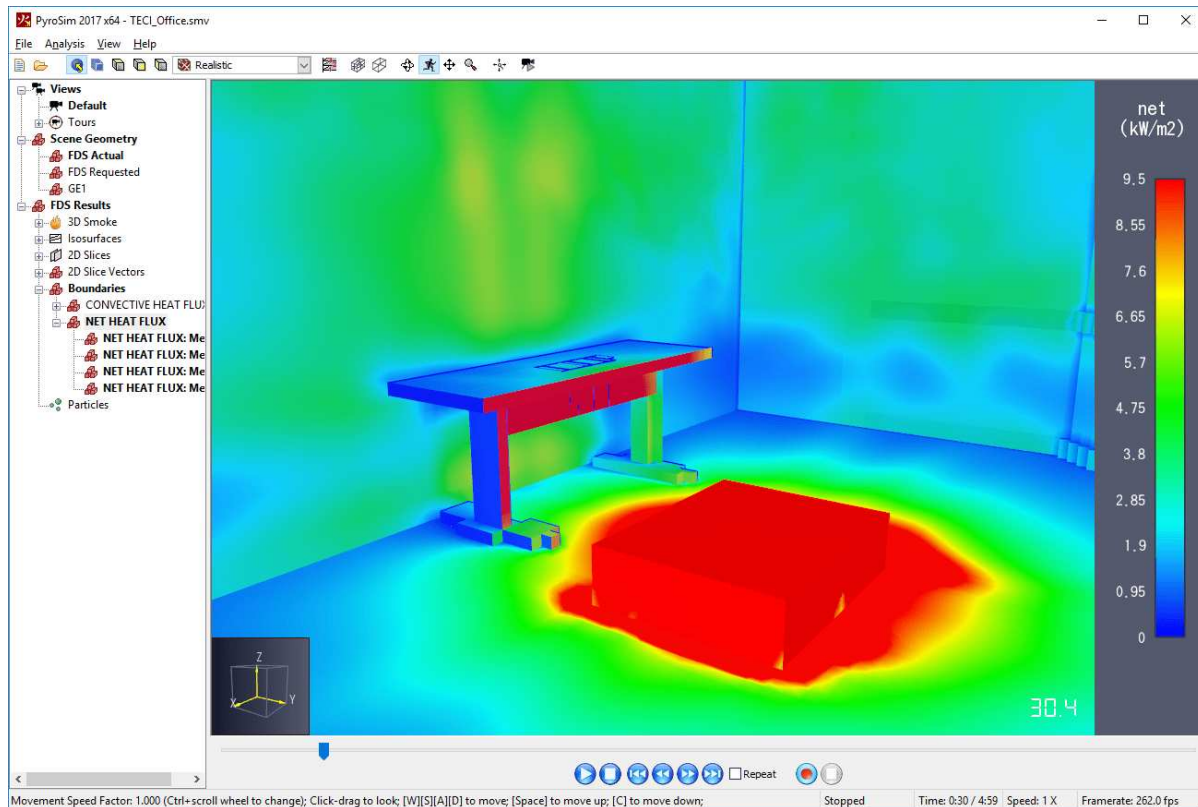
Figure 82. FDS Boundaries
