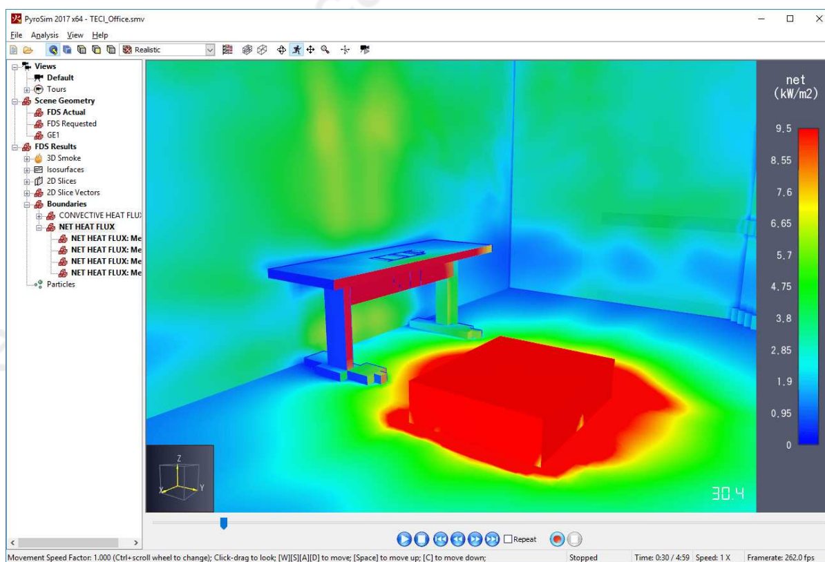
Figure 82. FDS Boundaries
