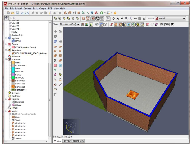
Figure 55. Single floor
