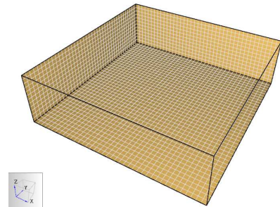
Figure 12. Mesh outline
