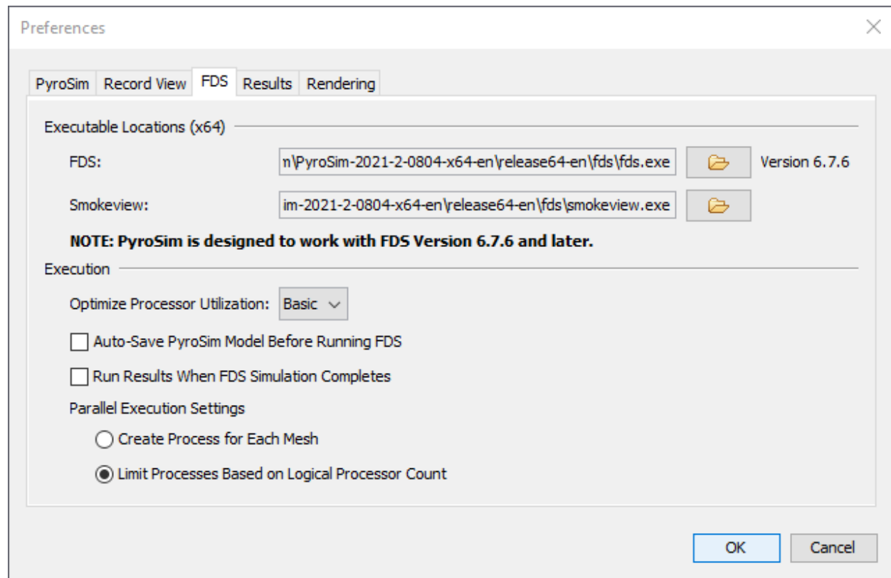
Figure 18. FDS Preferences
