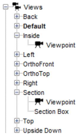
Figure 21. Views Tree
