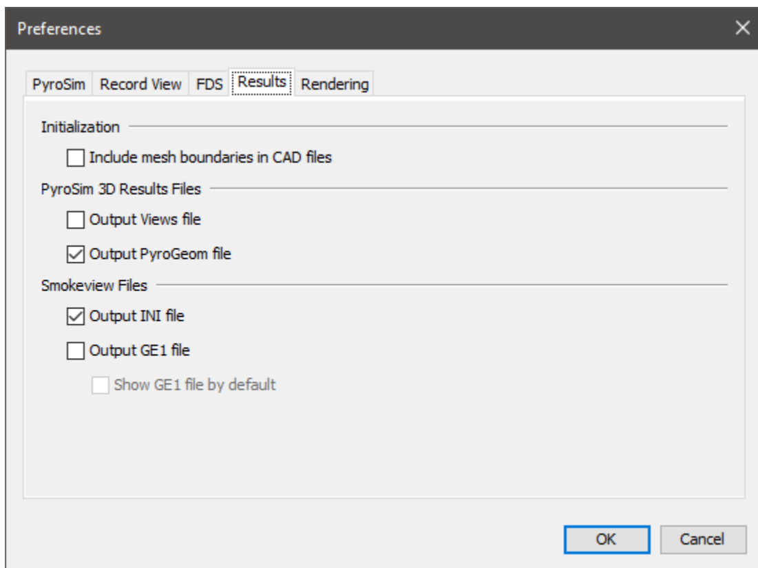
Figure 19. Results Preferences
