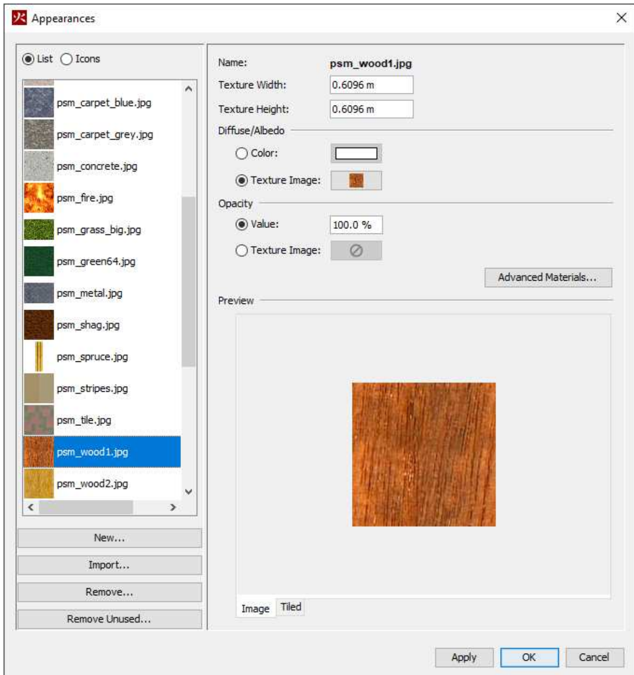
Figure 38. Appearances dialog
