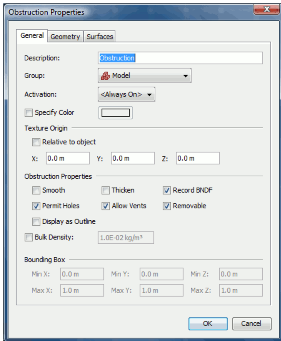
Figure 42. Obstruction dialog
