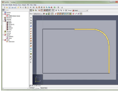
Figure 106. Shorter segments
