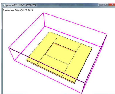
Figure 48. Improperly cut hole along mesh boundary in FDS
