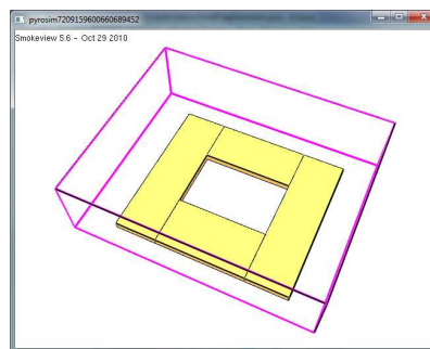
Figure 49. Properly cut hole along mesh boundary in FDS
