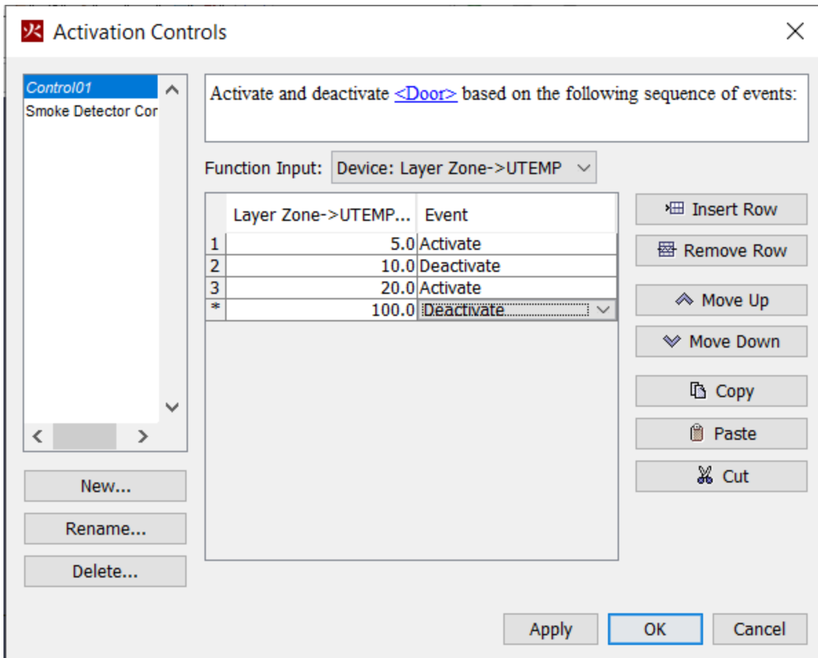
Figure 125. The Custom Control Dialog.
