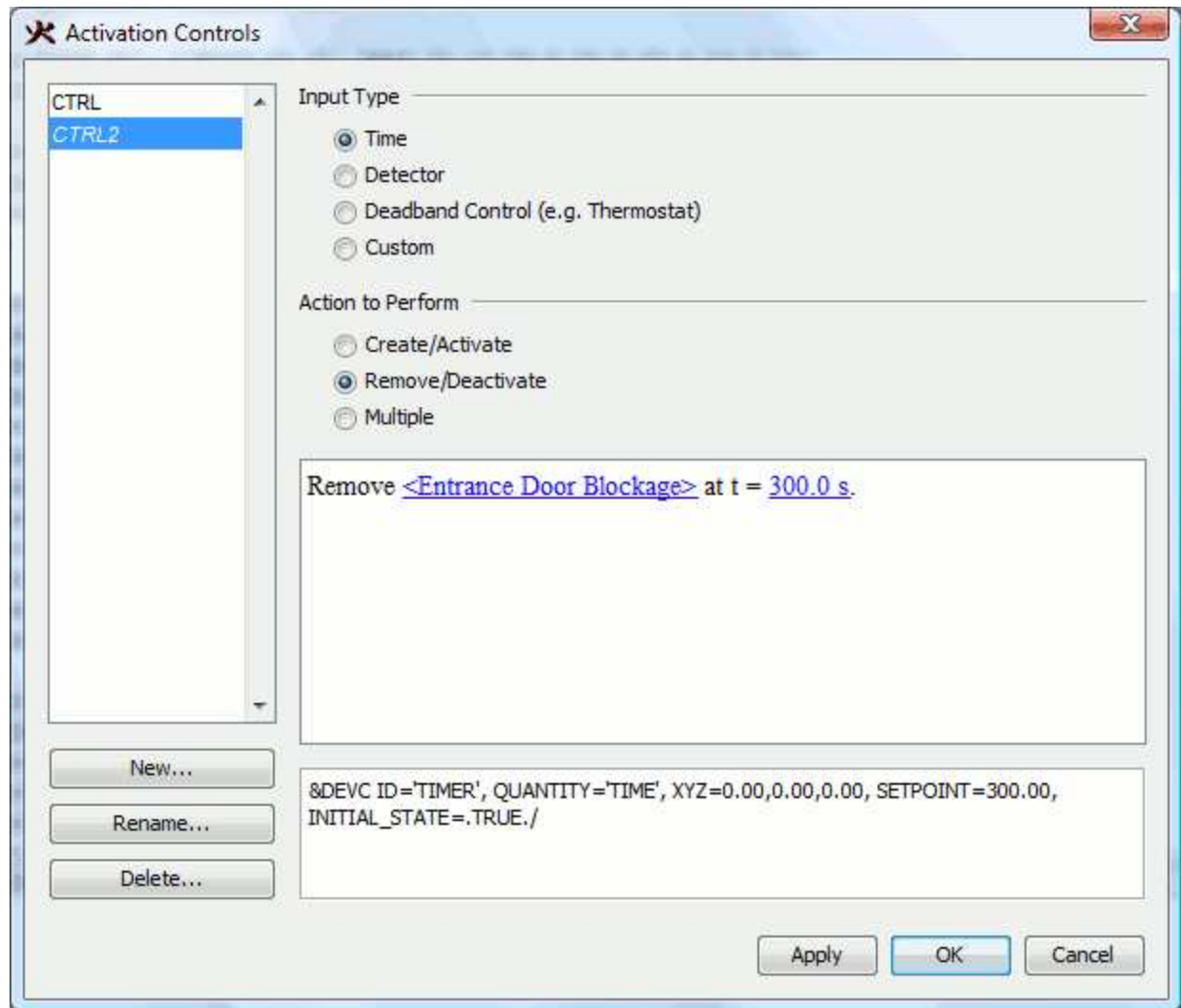
Figure 121. The Activation Controls dialog.
