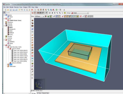
Figure 47. Hole along a mesh boundary
