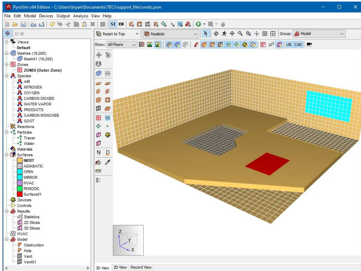
Figure 50. Vents on a mesh boundary and obstruction
