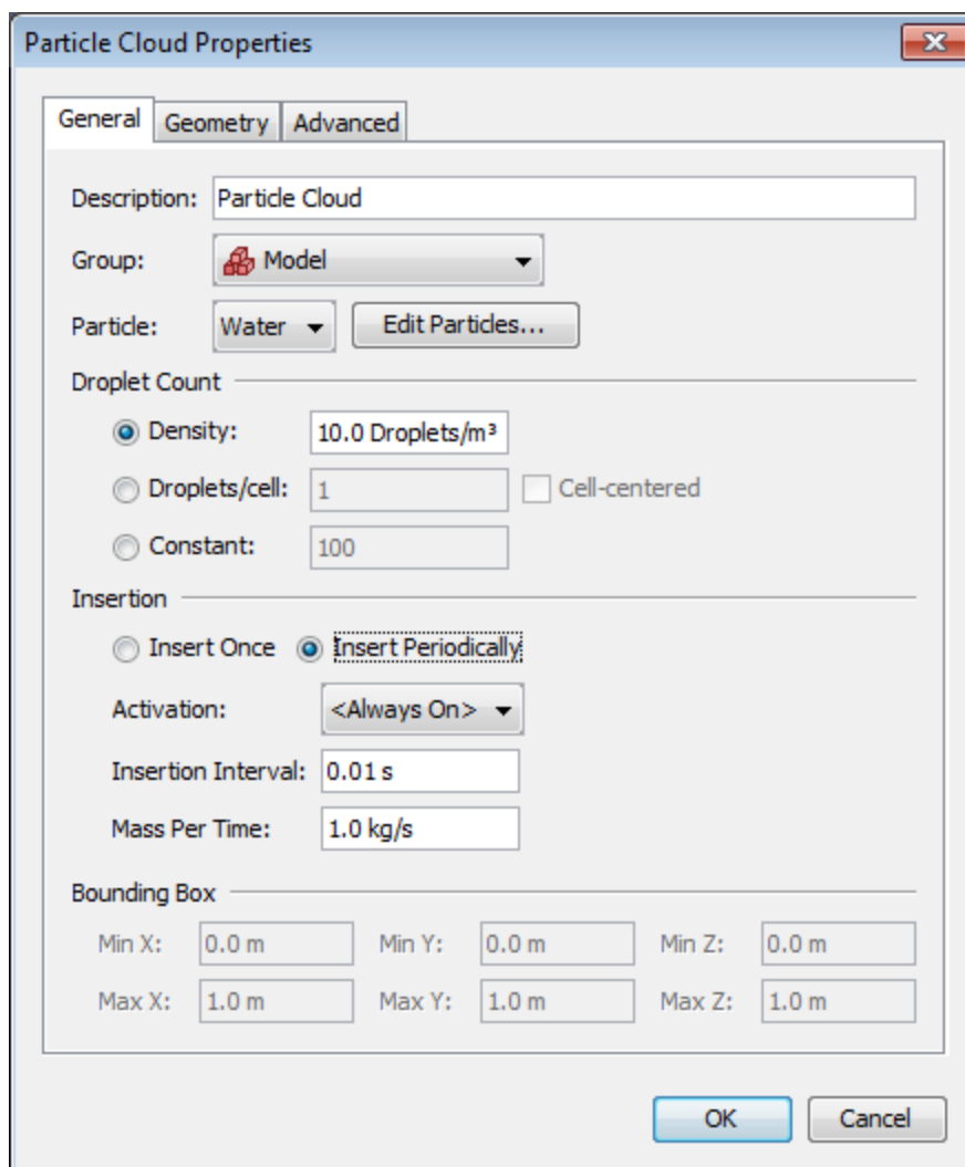
Figure 118. Particle Cloud dialog
