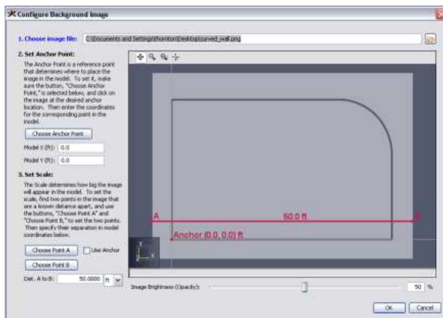
Figure 105. Background image settings for curved wall examples
