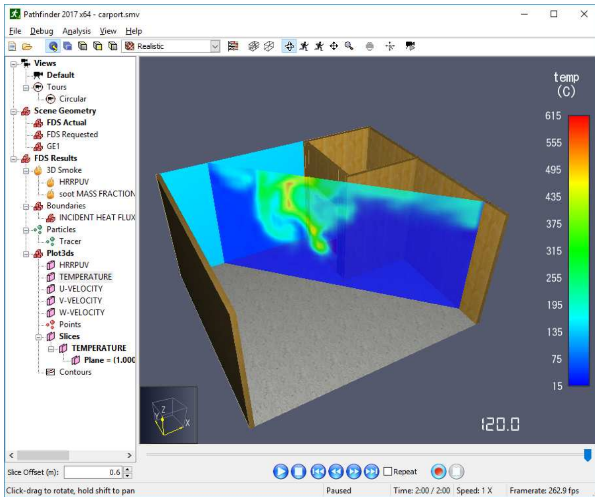
Figure 132. An angled temperature slice through Plot3D data shown in the 3D Results
