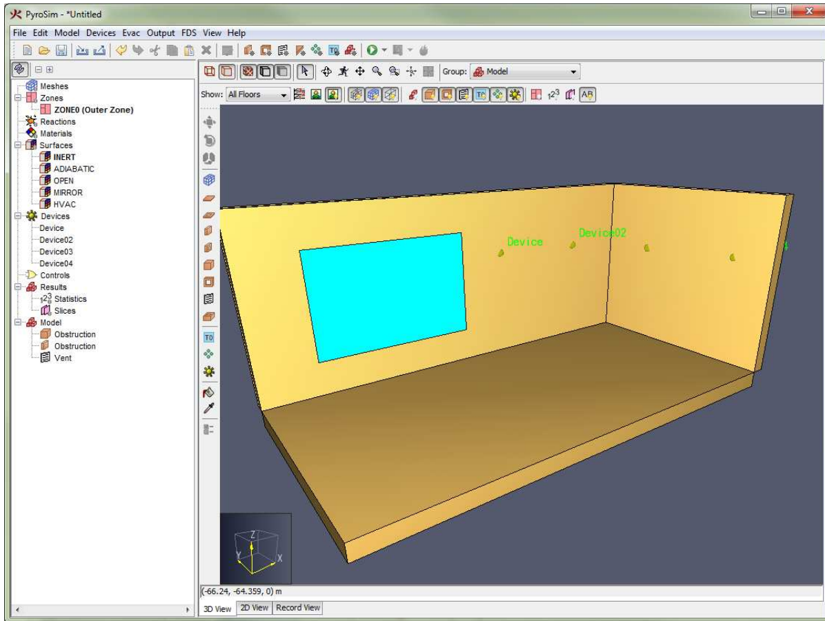
Figure 73. Vent and devices attached to a wall
