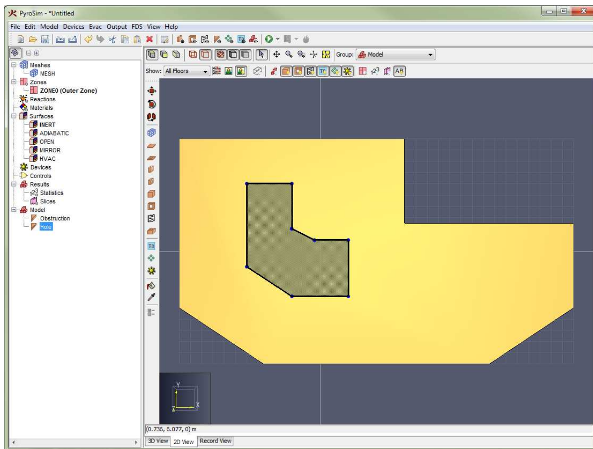
Figure 44. A slab obstruction with a hole cut from it
