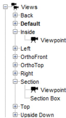
Figure 21. Views Tree
