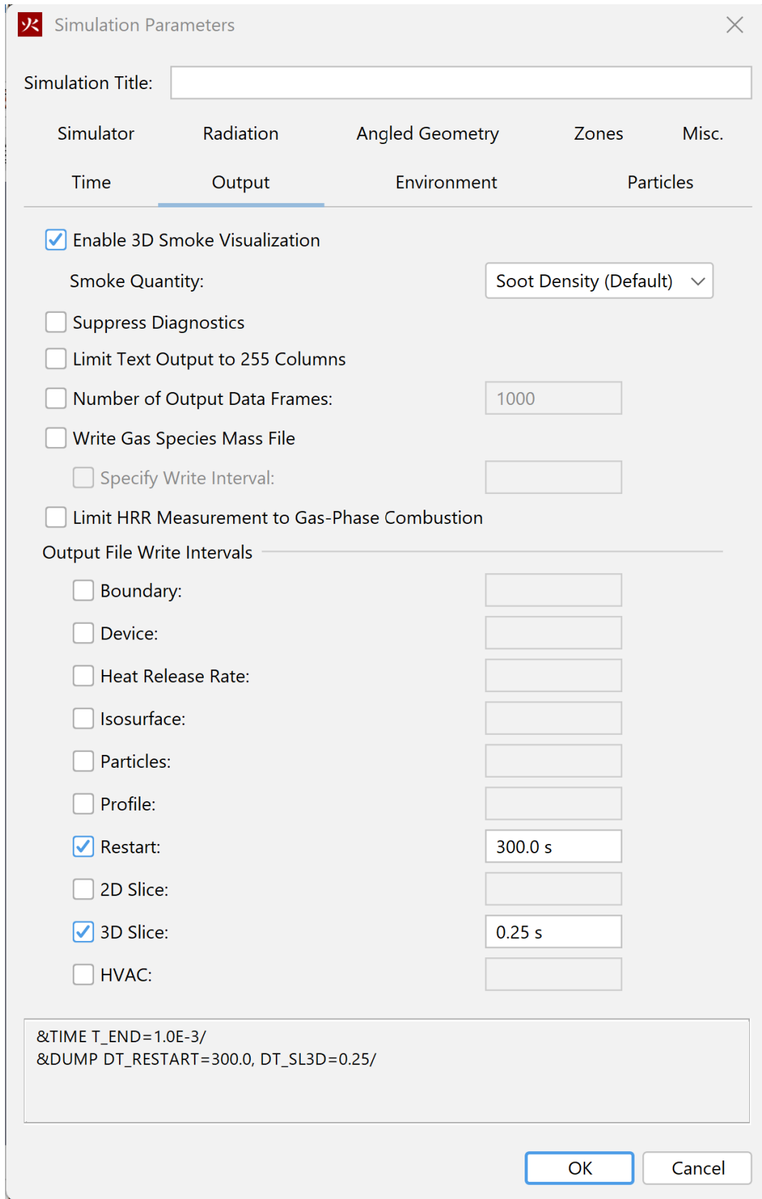
Figure 135. Output tab of the simulation parameters dialog
