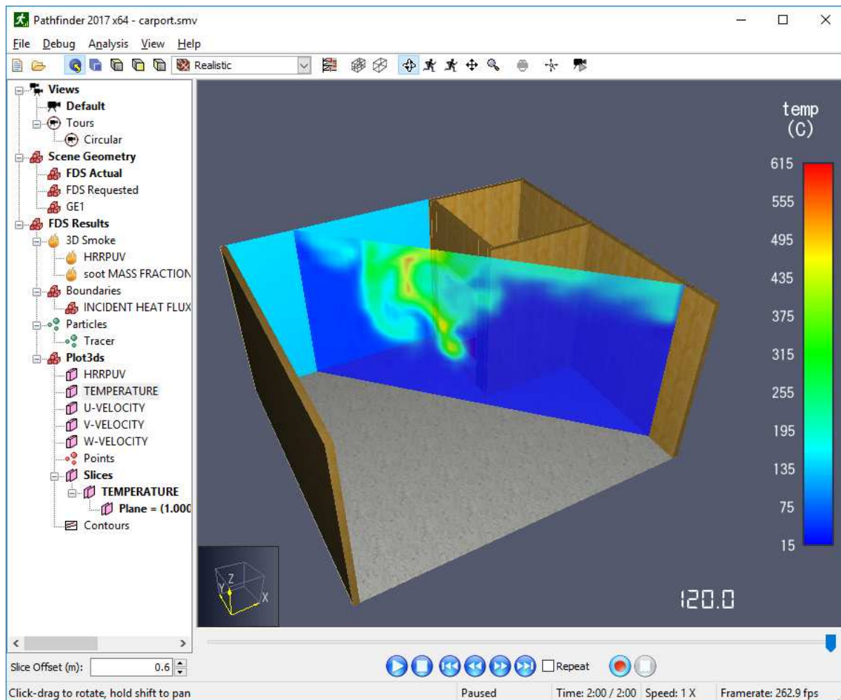
Figure 138. An angled temperature slice through Plot3D data shown in the 3D Results
