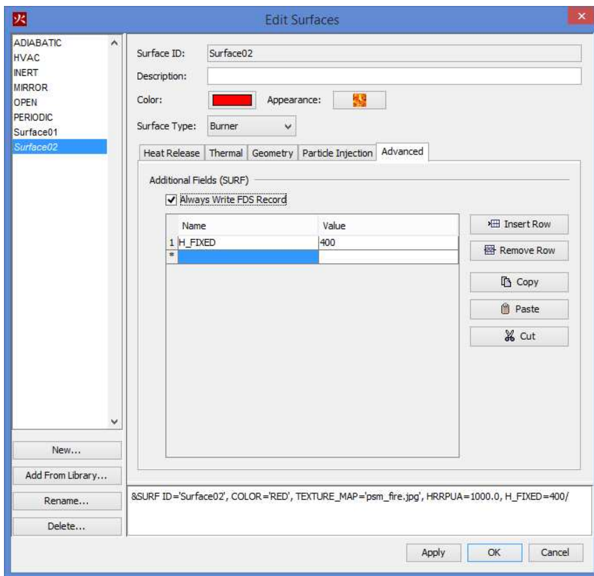
Figure 170. Additional Fields
