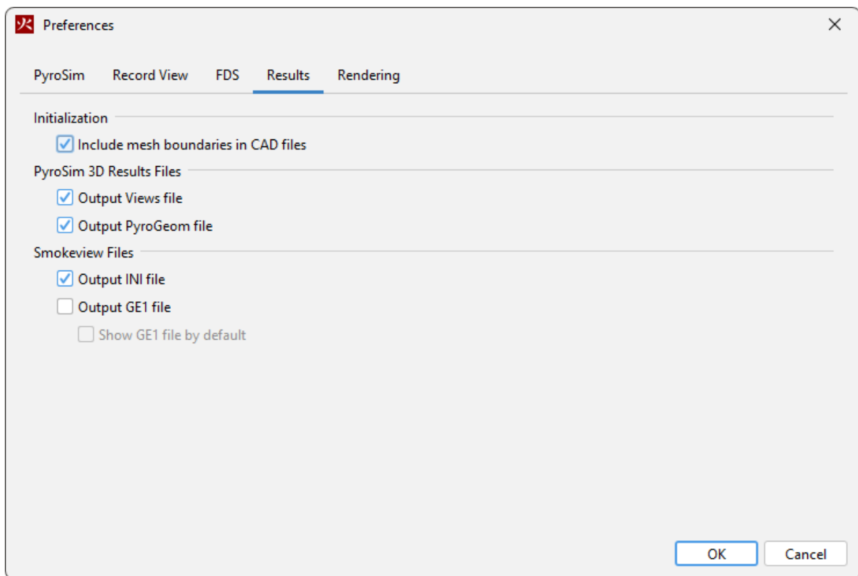
Figure 18. Results Preferences
