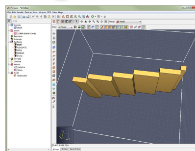
Figure 157. Thicken obstructions
