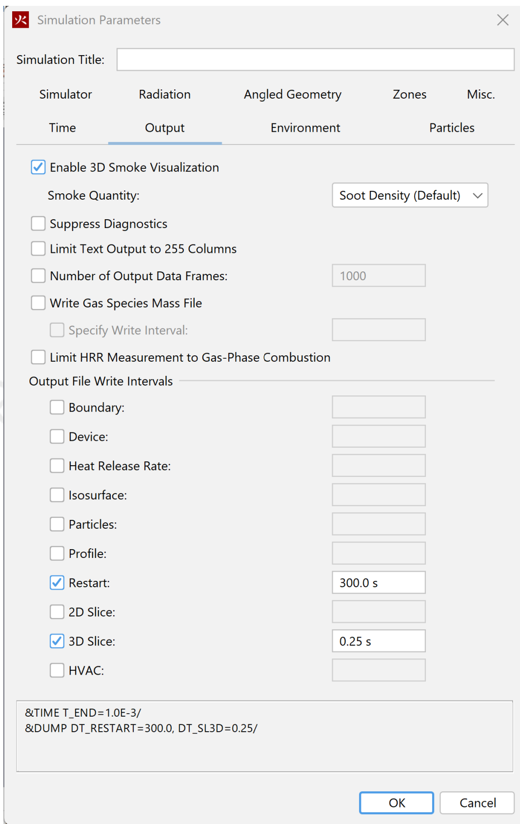
Figure 147. Output tab of the simulation parameters dialog
