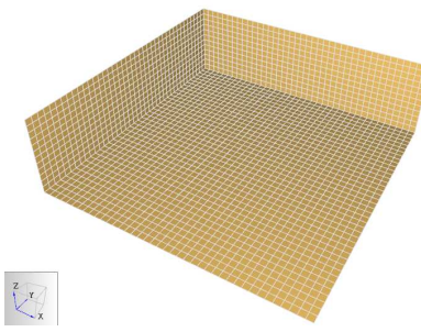
Figure 10. Mesh boundary
