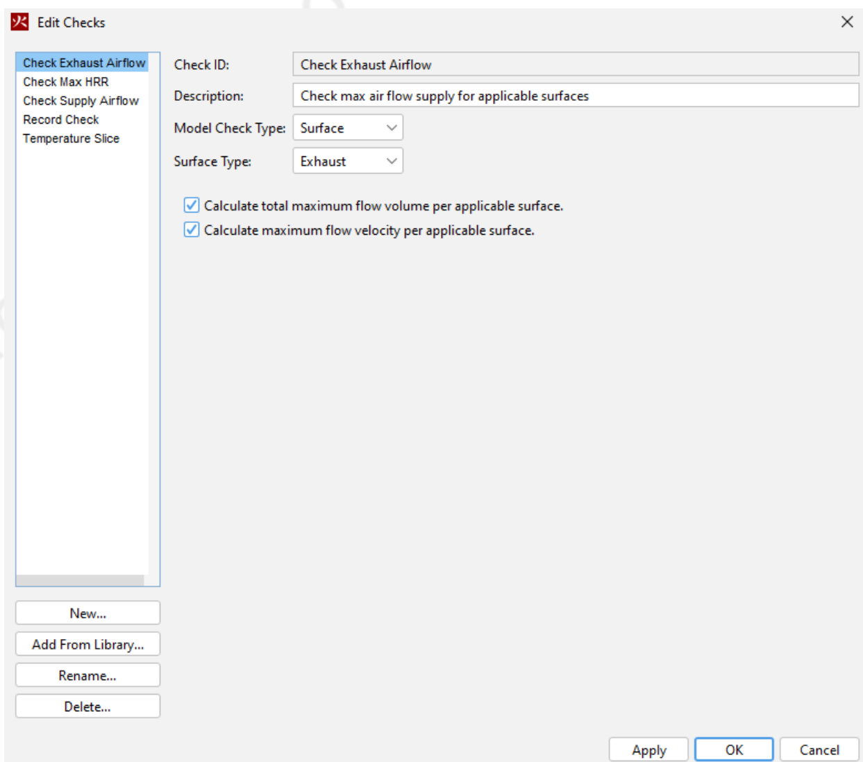
Figure 143. Creating a Surface Check
