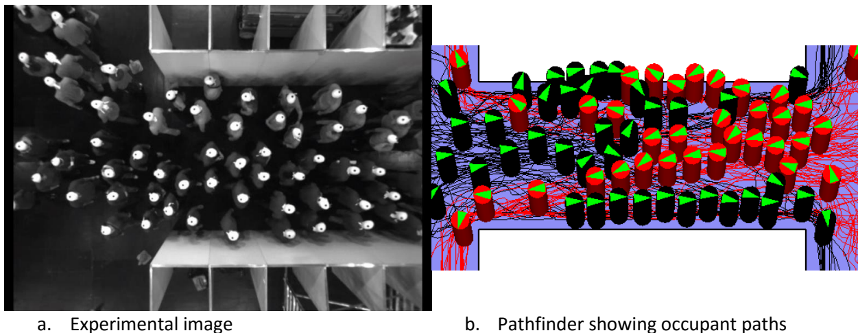
Figure 17: BFR-SSL-360-160-160, comparison of experimental and Pathfinder results at 50 seconds, 1.6 m entry width, free choice of destination.
