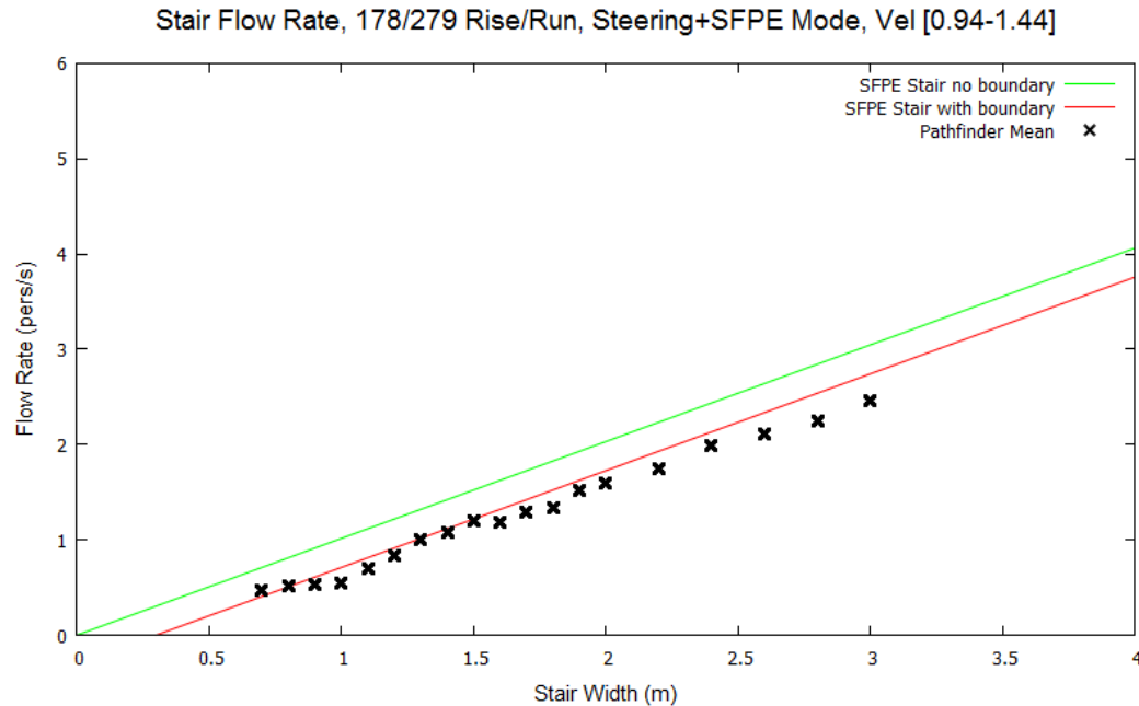
Figure 42: Stair flow rates for Steering+SFPE mode and occupants with a max speed distribution of 1.19 \pm 0.25 m/s.
