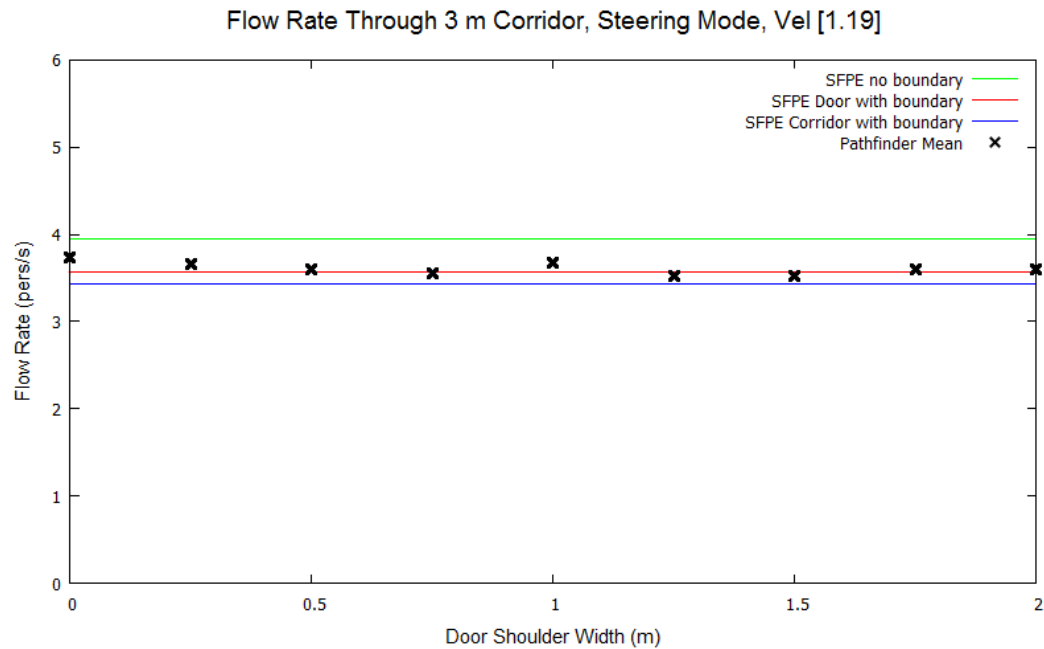
Figure 46: Corridor flow rates for 3 m corridor in Steering Mode with varying entry shoulder widths. Occupants have a constant max speed of 1.19 m/s.
