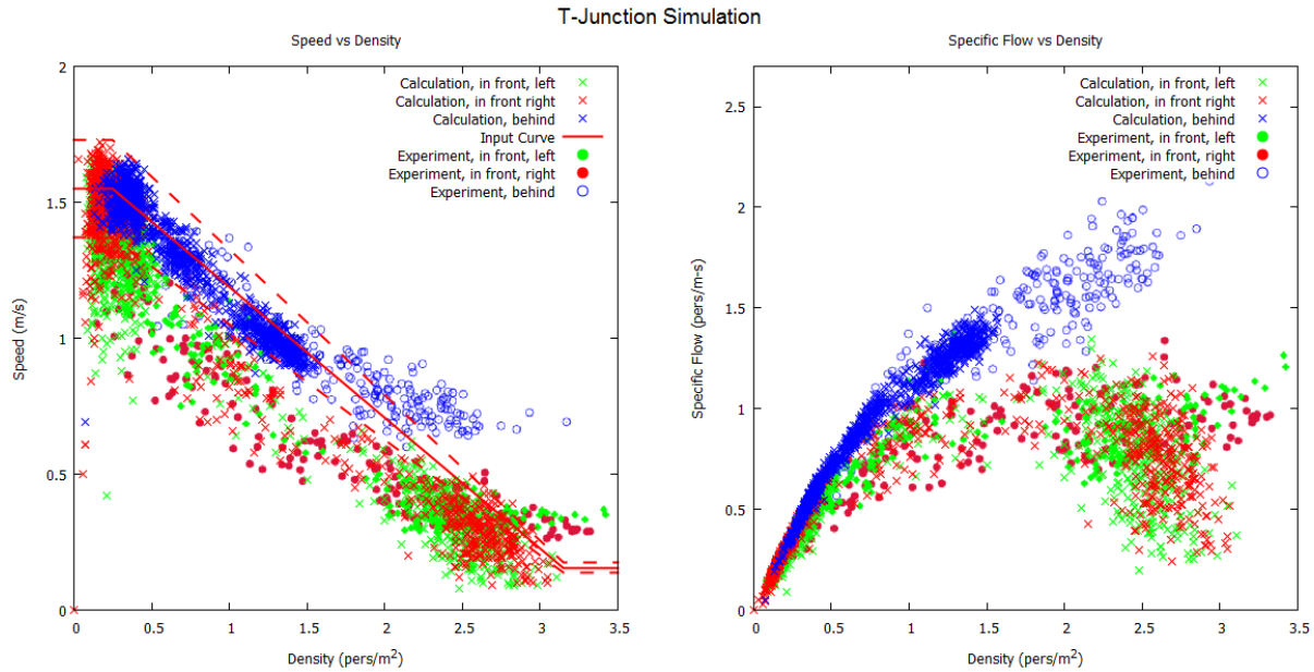
Figure 23: Speed-density results for Zhang and Seyfried experiment with measured speed-density input and uniform velocity distribution 1.55 \pm 0.18 m/s.
