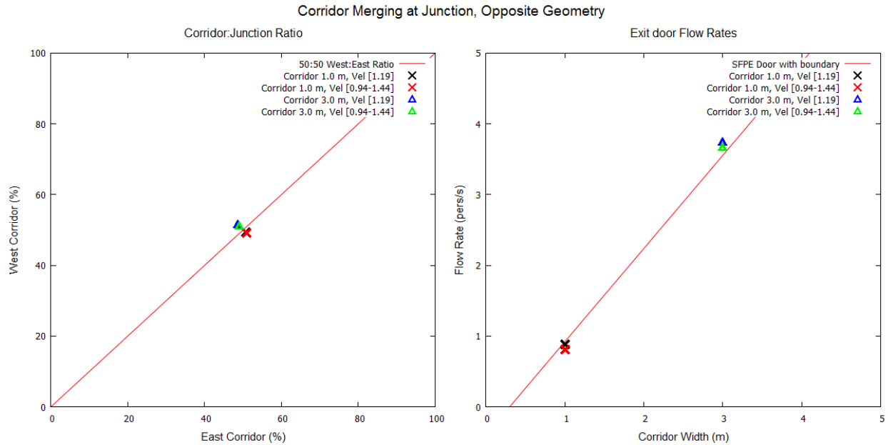
Figure 56: Merging ratios and exit door flow rates for merging at a corridor junction with "opposite" configuration.
