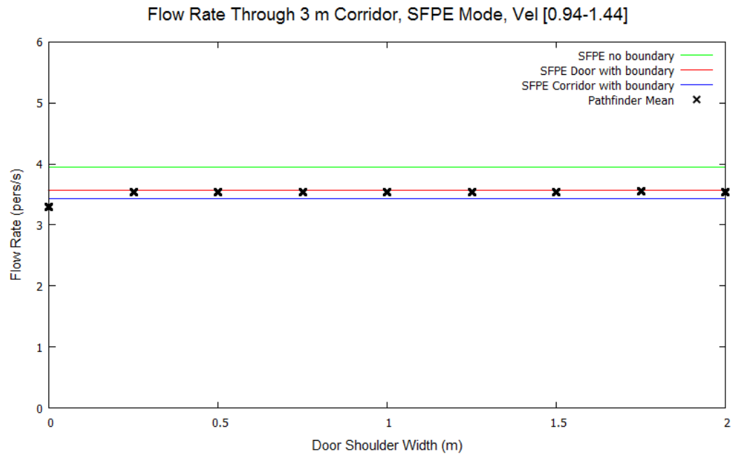
Figure 50: Corridor flow rates for 3 m corridor in SFPE Mode with varying entry shoulder widths. Occupants have a max speed distribution of 1.19 \pm 0.25 m/s.
