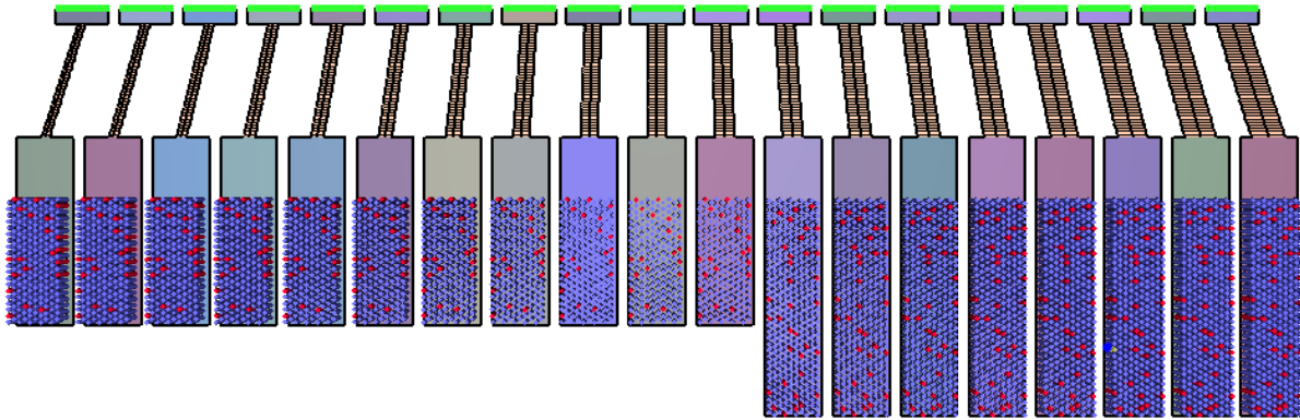
Figure 64: Pathfinder model used to study stair flow rates with mobility-impaired occupants. The door widths range from 0.7 to 3.0 m. Entry corridor width is 5 m. Stairs have a total rise of 7 m and a run of 11 m.
