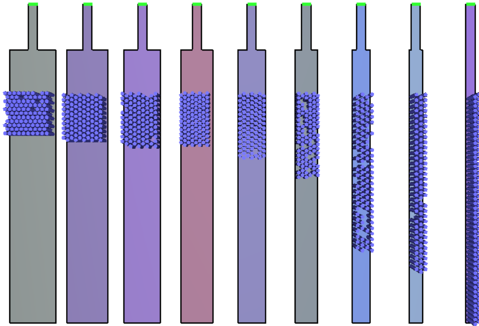
Figure 43: Pathfinder model used to study corridor flow rates. The corridor width is 1 m and the entry shoulders vary from 0 to 2 m.
