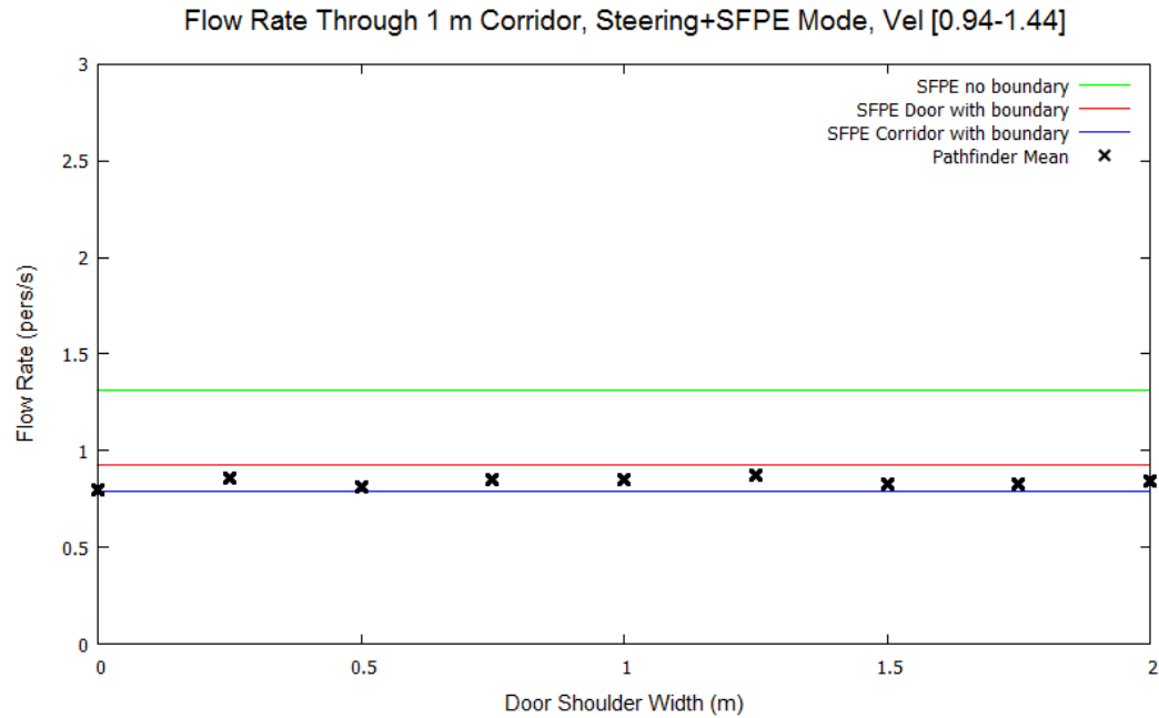
Figure 51: Corridor flow rates for 1 m corridor in Steering+SFPE Mode with varying entry shoulder widths. Occupants have a max speed distribution of 1.19 \pm 0.25 m/s.
