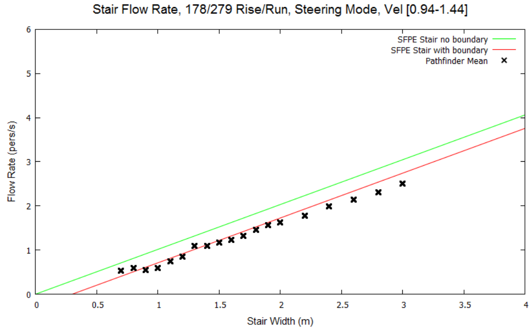
Figure 40: Stair flow rates for Steering mode and occupants with a max speed distribution of 1.19 \pm 0.25 m/s.
