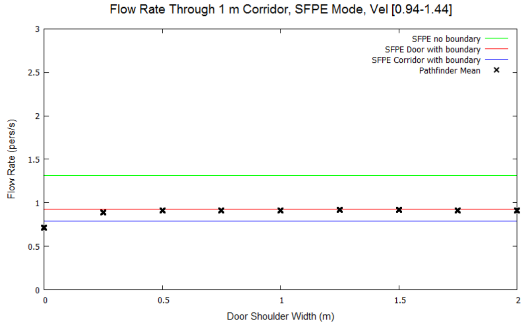
Figure 49: Corridor flow rates for 1 m corridor in SFPE Mode with varying entry shoulder widths. Occupants have a max speed distribution of 1.19 \pm 0.25 m/s.
