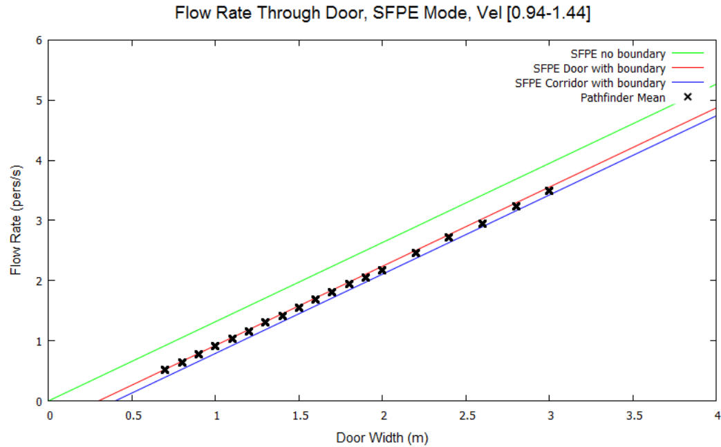
Figure 36: Door flow rates for SFPE mode and occupants with a max speed distribution of 1.19 \pm 0.25 m/s.
