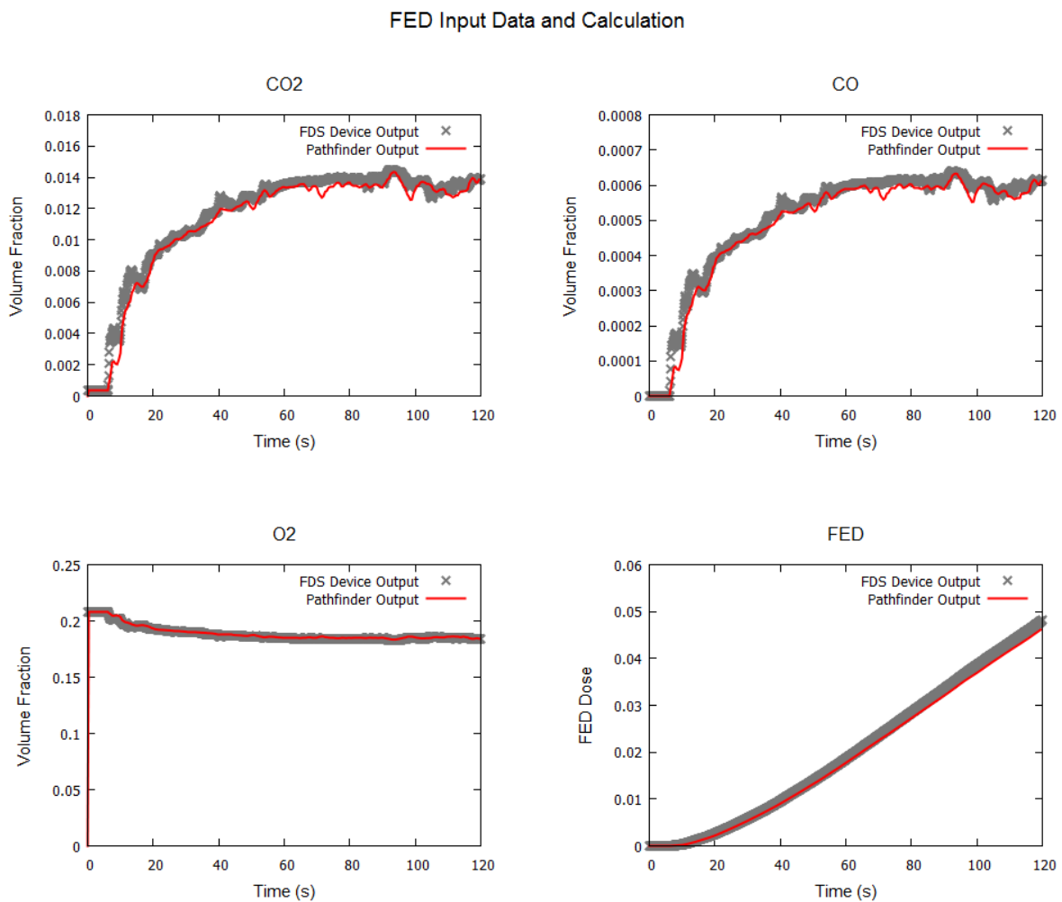
Figure 72: Comparison of FDS device output and Pathfinder input and FED calculation.
