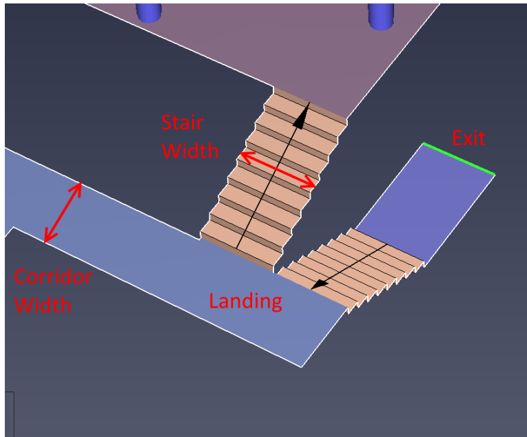
Figure 59: Stair merging geometry. The arrows indicate the “up” direction on the stairs, not the flow direction.
