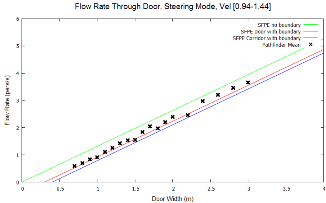
Figure 35: Door flow rates for Steering mode and occupants with a max speed distribution of 1.19 \pm 0.25 m/s.
