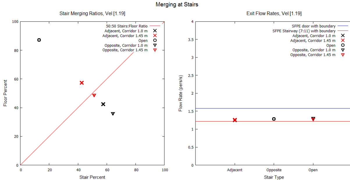
Figure 62: Merging ratios and exit flow rates for stair merging with a constant maximum occupant speed of 1.19 m/s.
