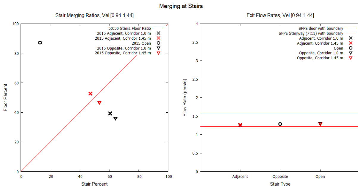
Figure 63: Merging ratios and exit flow rates for stair merging with a uniformly distributed maximum occupant speed of 1.19 \pm 0.25 m/s.
