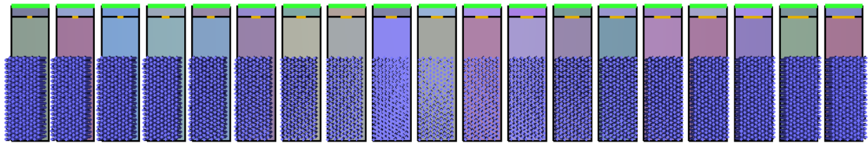
Figure 33: Pathfinder model used to study door flow rates. The door widths range from 0.7 to 3.0 m. Entry corridor width is 5 m.
