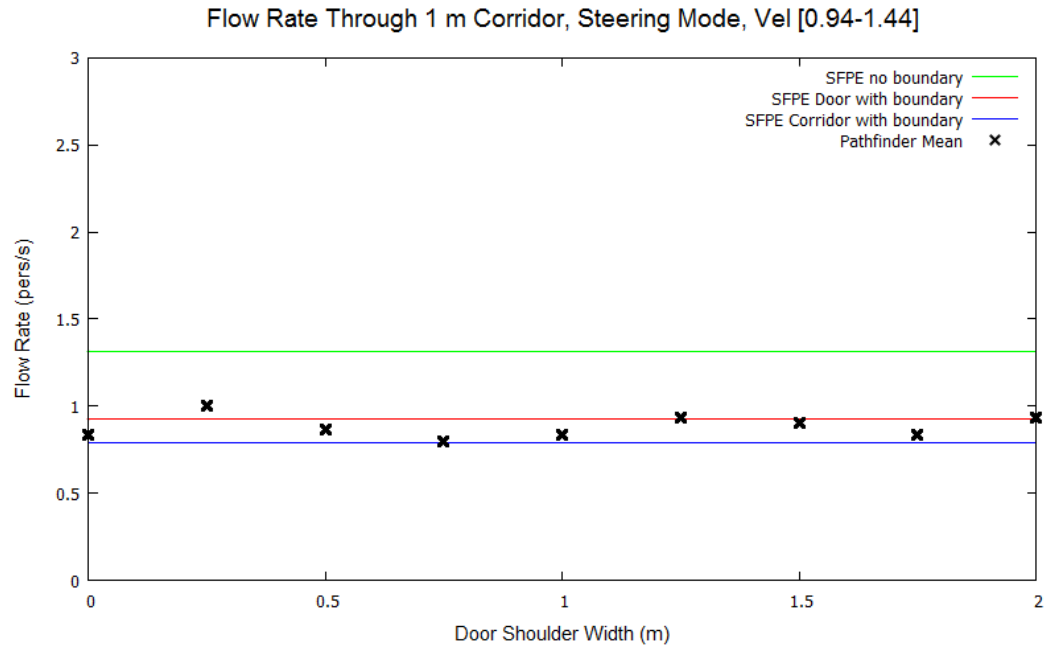
Figure 47: Corridor flow rates for 1 m corridor in Steering Mode with varying entry shoulder widths. Occupants have a max speed distribution of 1.19 \pm 0.25 m/s.
