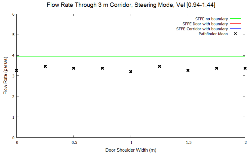
Figure 48: Corridor flow rates for 3 m corridor in Steering Mode with varying entry shoulder widths. Occupants have a max speed distribution of 1.19 \pm 0.25 m/s.
