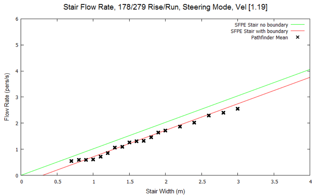
Figure 39: Stair flow rates for Steering mode and occupants with a max speed of 1.19 m/s.
