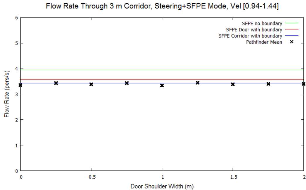
Figure 52: Corridor flow rates for 3 m corridor in Steering+SFPE Mode with varying entry shoulder widths. Occupants have a max speed distribution of 1.19 \pm 0.25 m/s.
