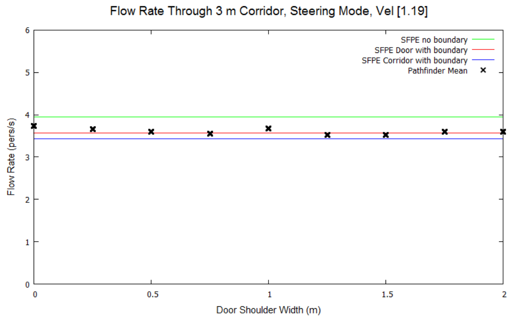
Figure 46: Corridor flow rates for 3 m corridor in Steering Mode with varying entry shoulder widths. Occupants have a constant max speed of 1.19 m/s.
