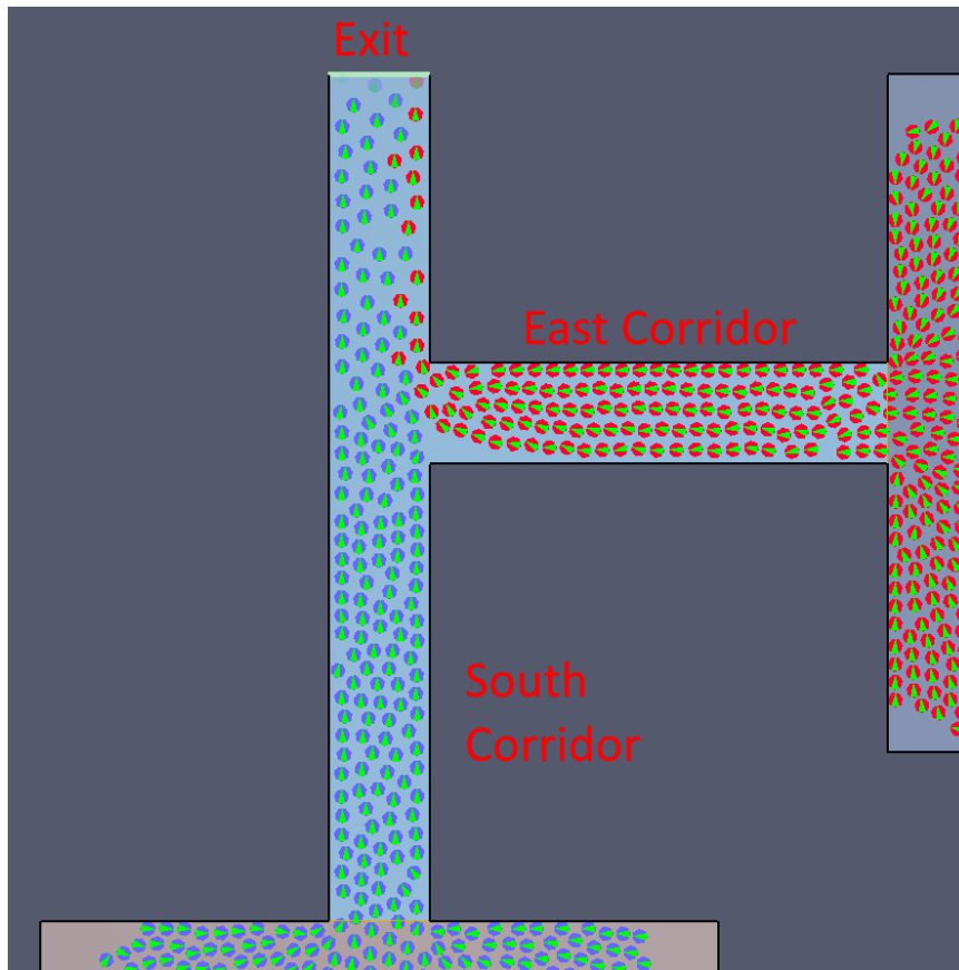
Figure 53: Model for merging at a corridor junction. Called an “adjacent’ geometry.
