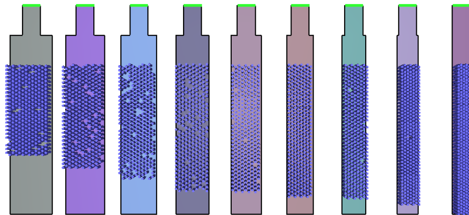
Figure 44: Pathfinder model used to study corridor flow rates. The corridor width is 3 m and the entry shoulders vary from 0 to 2 m.
