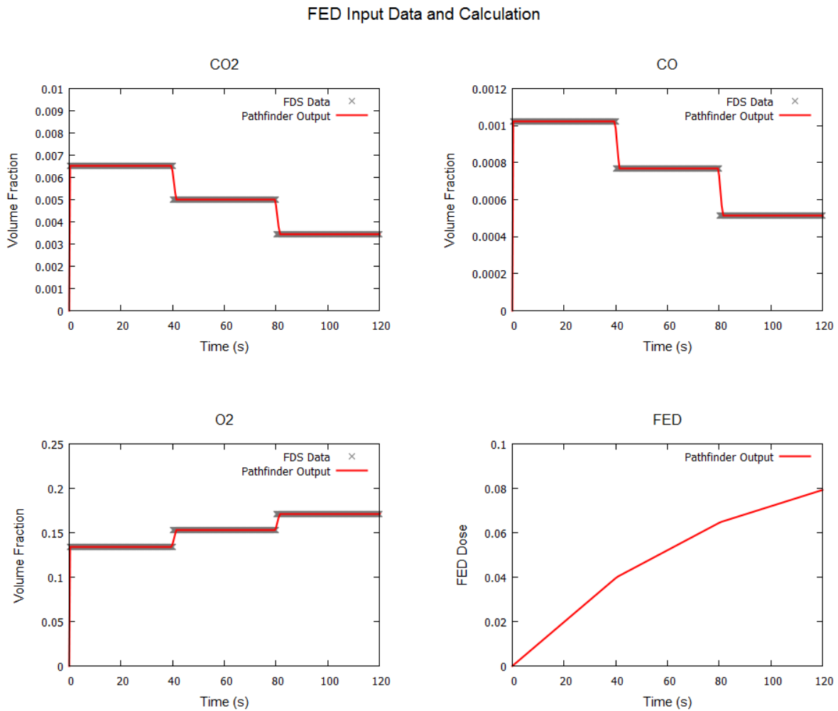
Figure 75: Comparison of FDS device output and Pathfinder input and FED calculation for moving occupant.
