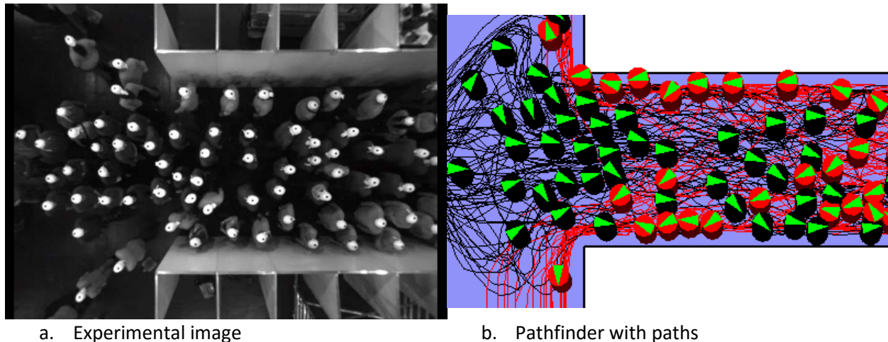
Figure 19: BFR-DML-360-160-160, comparison of experimental and Pathfinder results at 30 seconds, assigned destination.
