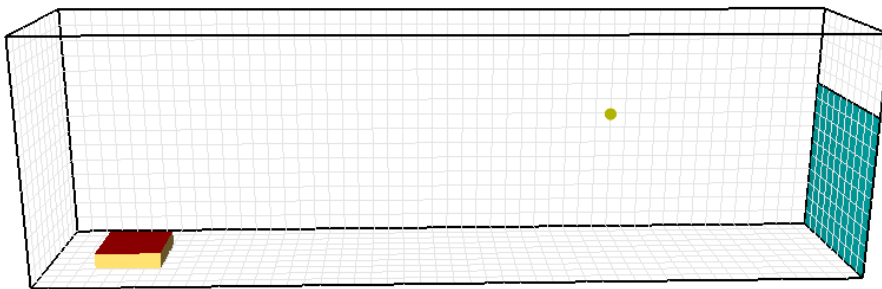
Figure 70: PyroSim model of FED calculation using stationary occupant.
