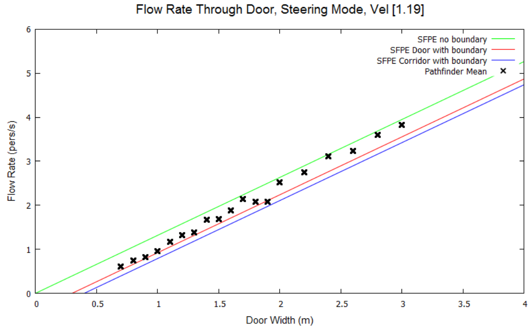
Figure 34: Door flow rates for Steering mode and occupants with a max speed of 1.19 m/s.
