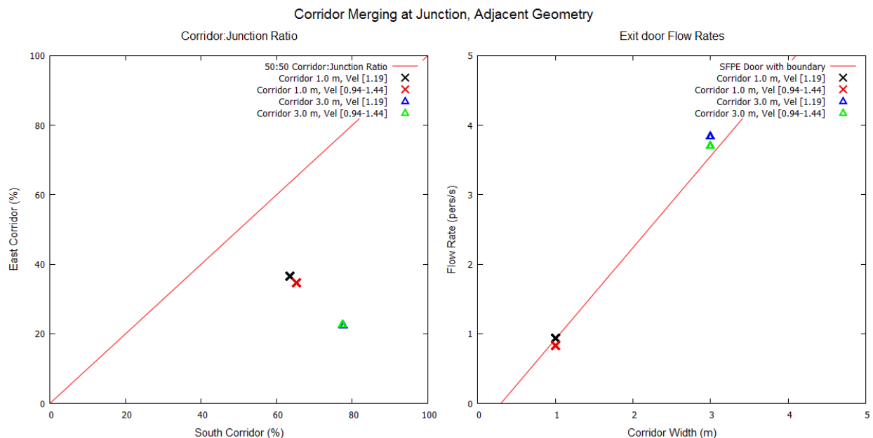
Figure 55: Merging ratios and exit door flow rates for merging at a corridor junction with "adjacent" configuration.
