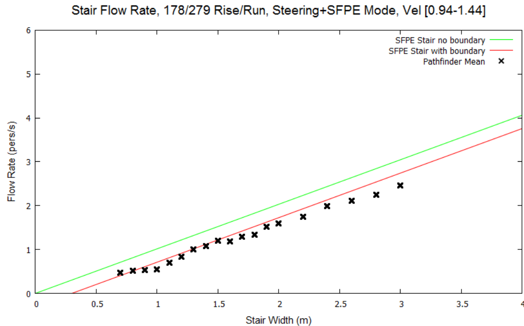
Figure 42: Stair flow rates for Steering+SFPE mode and occupants with a max speed distribution of 1.19 \pm 0.25 m/s.
