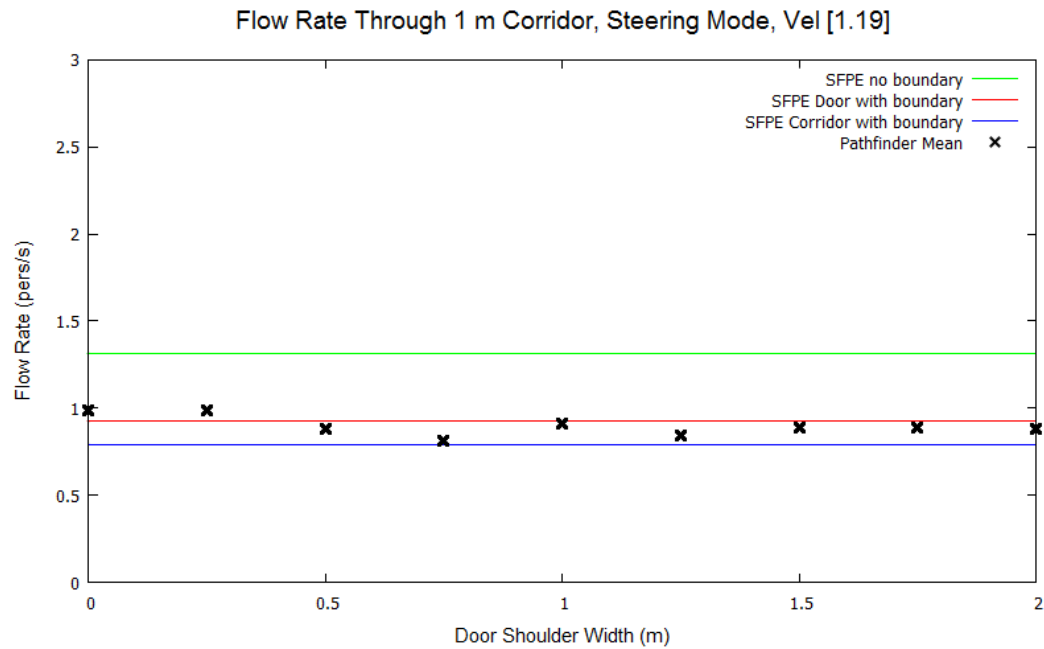
Figure 45: Corridor flow rates for 1 m corridor in Steering Mode with varying entry shoulder widths. Occupants have a constant max speed of 1.19 m/s.
