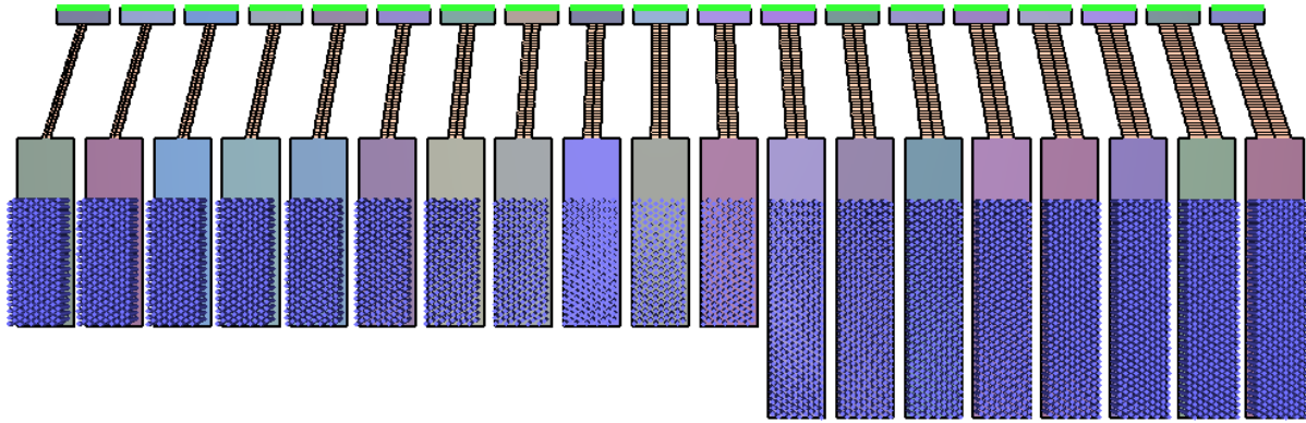
Figure 38: Pathfinder model used to study stair flow rates. The door widths range from 0.7 to 3.0 m. Entry corridor width is 5 m. Stairs have a total rise of 7 m and a run of 11 m.
