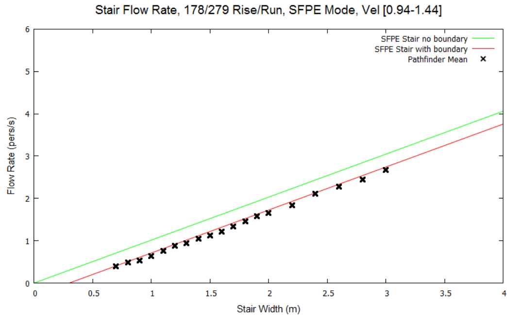
Figure 41: Stair flow rates for SFPE mode and occupants with a max speed distribution of 1.19 \pm 0.25 m/s.
