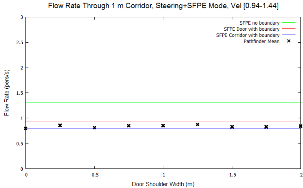
Figure 48: Corridor flow rates for 1 m corridor in Steering+SFPE Mode with varying entry shoulder widths. Occupants have a max speed distribution of 1.19 \pm 0.25 m/s.
