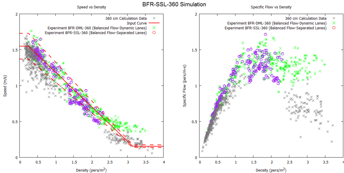
Figure 14: Speed-density results for Zhang and Seyfried experiment geometry, free choice of destination, with unidirectional speed-density input and uniform velocity distribution 1.55 \pm 0.18 m/s.
