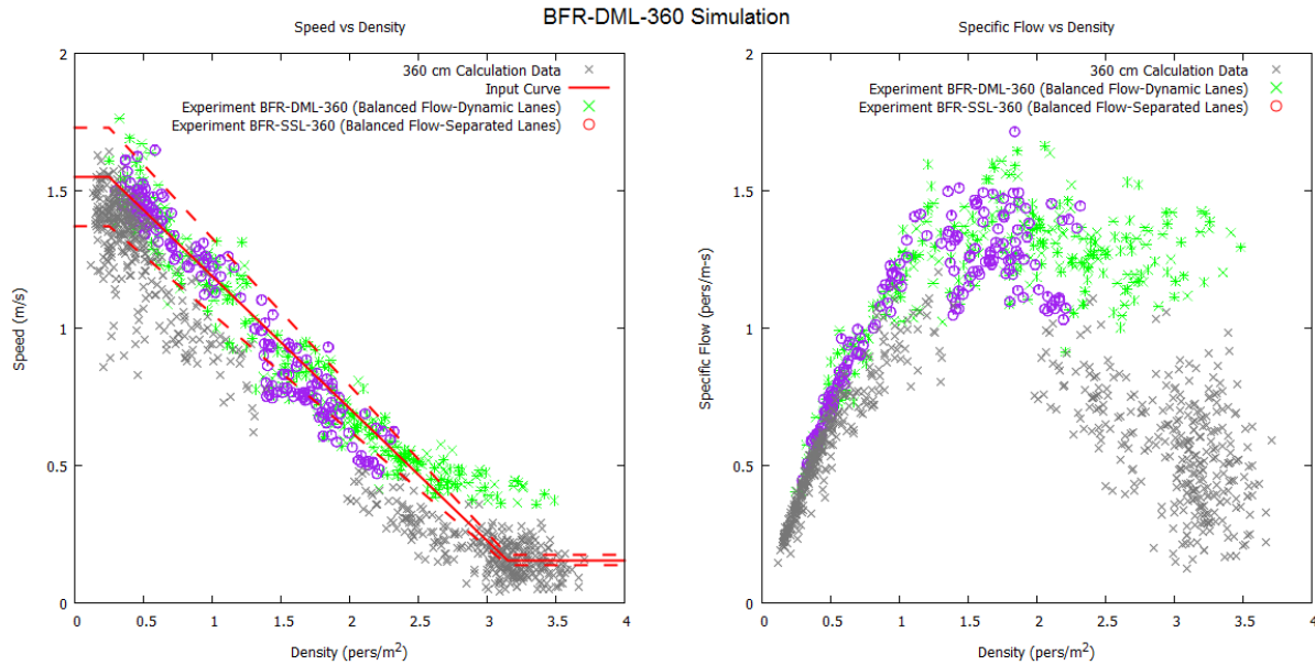
Figure 16: Speed-density results for Zhang and Seyfried experiment geometry, assigned destination, with unidirectional speed-density input and uniform velocity distribution 1.55 \pm 0.18 m/s.
