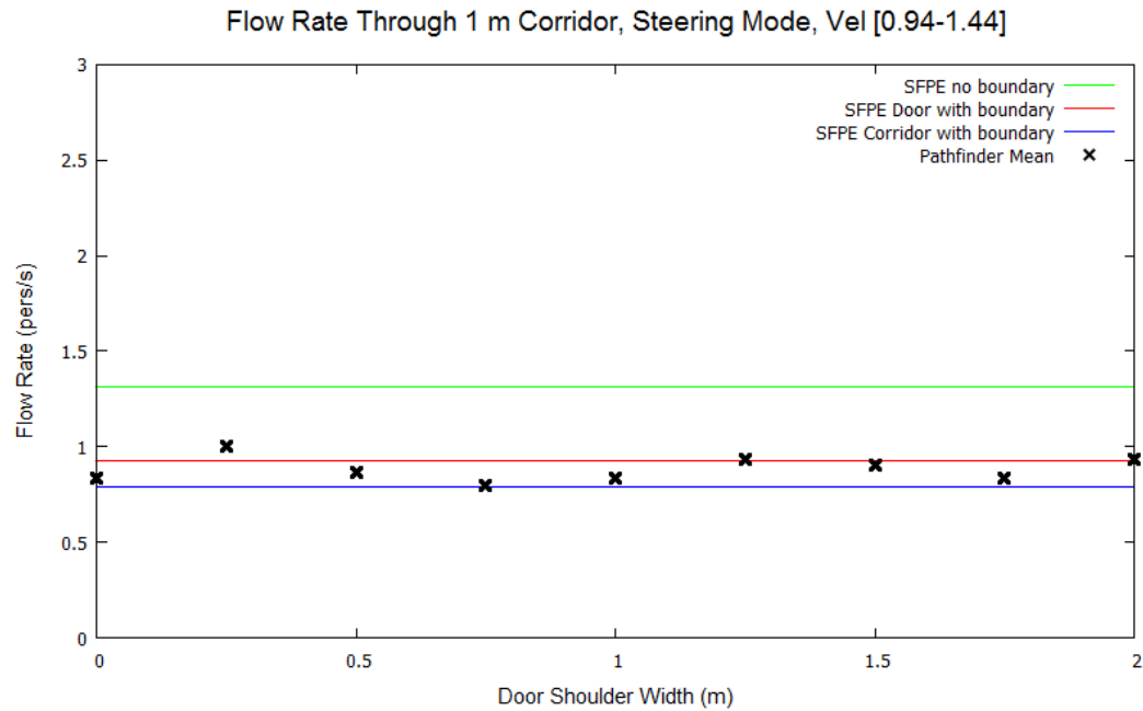
Figure 44: Corridor flow rates for 1 m corridor in Steering Mode with varying entry shoulder widths. Occupants have a max speed distribution of 1.19 \pm 0.25 m/s.
