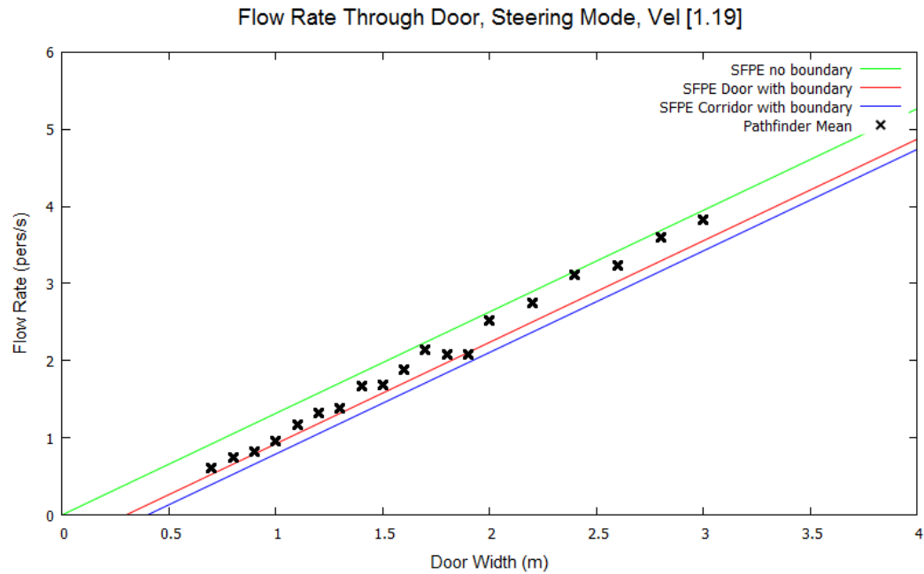
Figure 31: Door flow rates for Steering mode and occupants with a max speed of 1.19 m/s.
