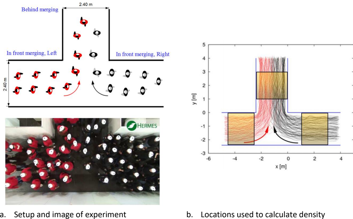
Figure 18: Setup and snapshot of T-junction experiment. The gray area in the sketch shows the location of measurement area (Ref. Zhang and Seyfried, 2012).
