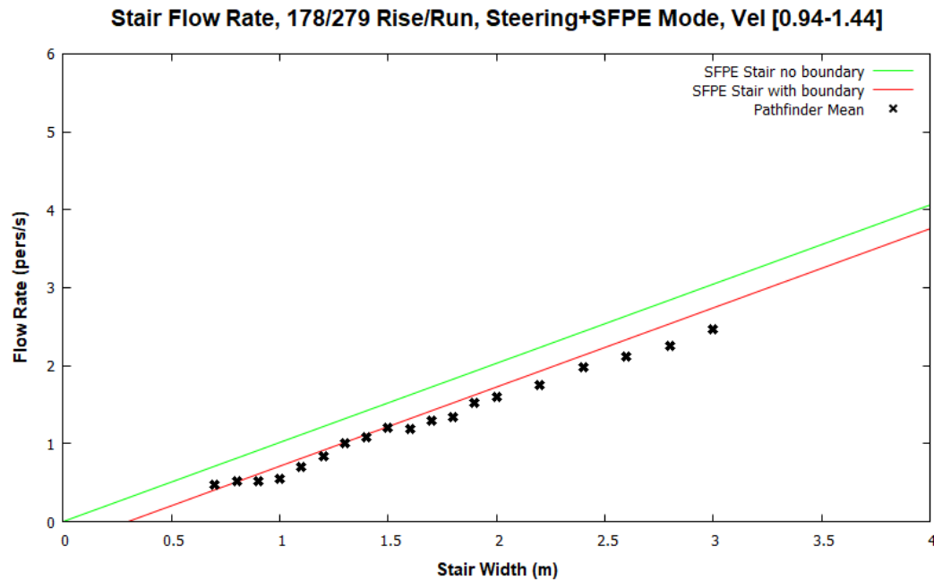
Figure 39: Stair flow rates for Steering+SFPE mode and occupants with a max speed distribution of 1.19 \pm 0.25 m/s.
