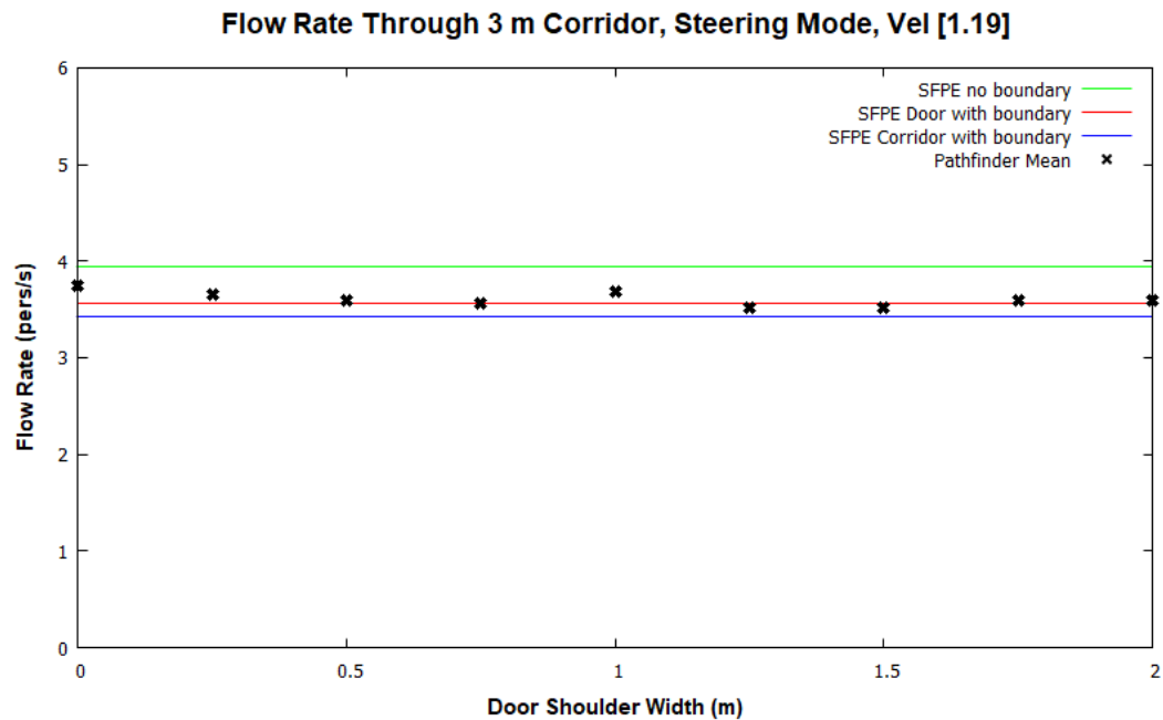
Figure 43: Corridor flow rates for 3 m corridor in Steering Mode with varying entry shoulder widths. Occupants have a constant max speed of 1.19 m/s.
