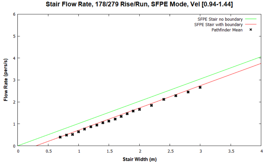
Figure 38: Stair flow rates for SFPE mode and occupants with a max speed distribution of 1.19 \pm 0.25 m/s.
