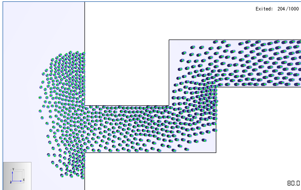
Figure 75: Steering mode showing use of the corridor with two corners.
