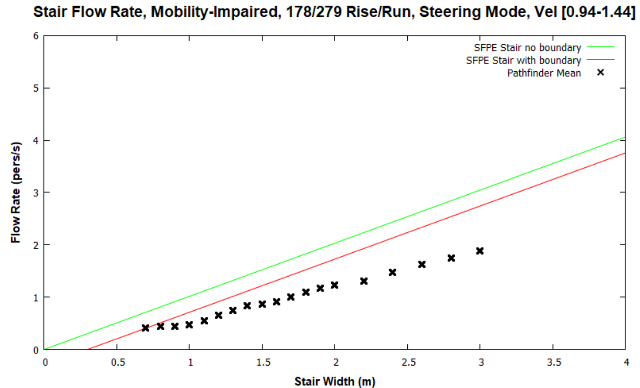
Figure 71: Stair flow rates for Steering mode, 90 percent of occupants have a max speed distribution of 1.19 \pm 0.25 m/s, 10 percent have a constant speed of 0.5 m/s.
