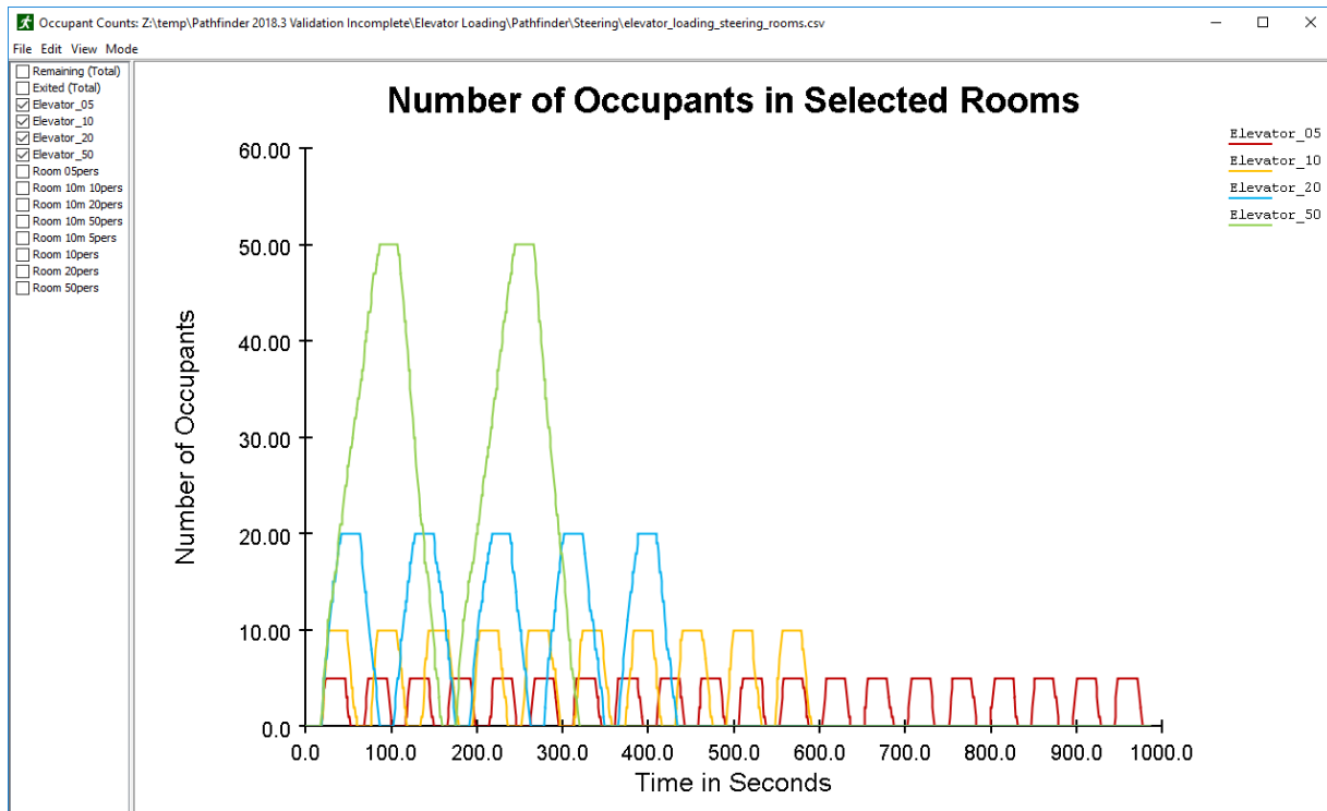
Figure 73: Observed elevator loading for steering mode
