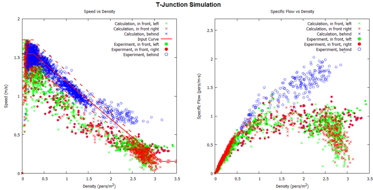
Figure 21: Speed-density results for Zhang and Seyfried experiment with measured speed-density input and uniform velocity distribution 1.55 \pm 0.18 m/s.
