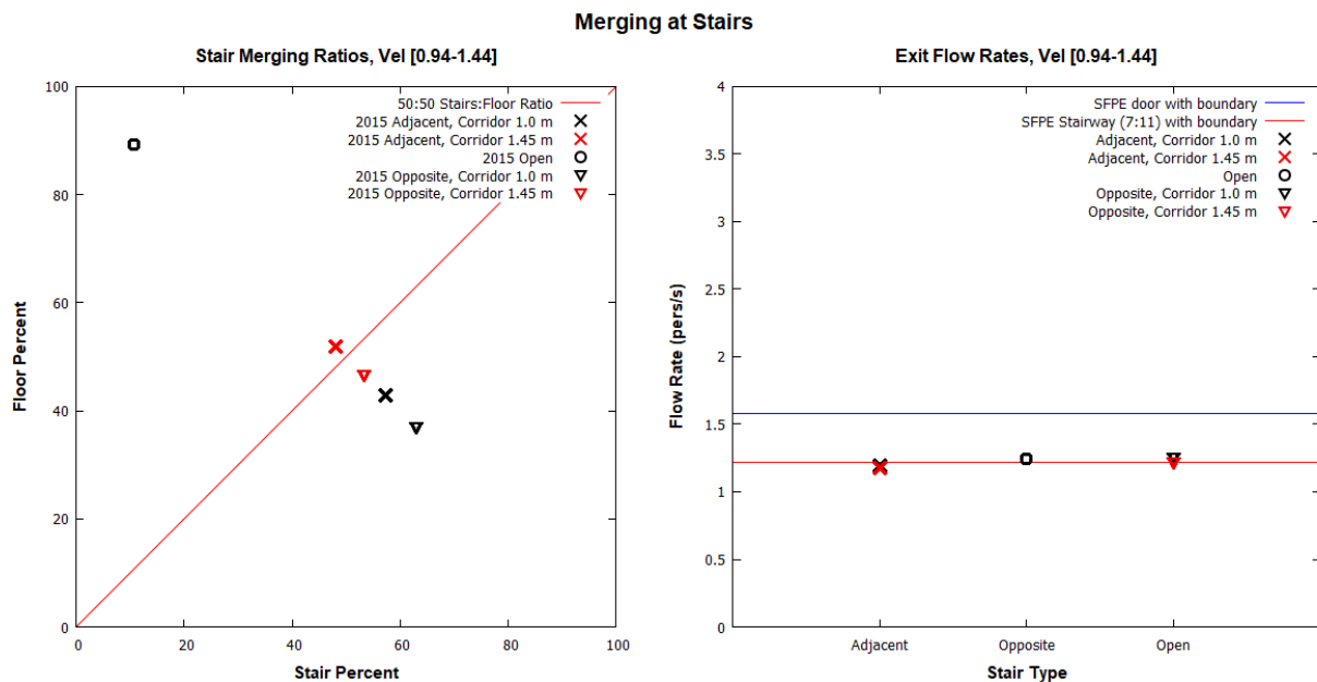
Figure 69: Merging ratios and exit flow rates for stair merging with a uniformly distributed maximum occupant speed of 1.19 \pm 0.25 m/s.
