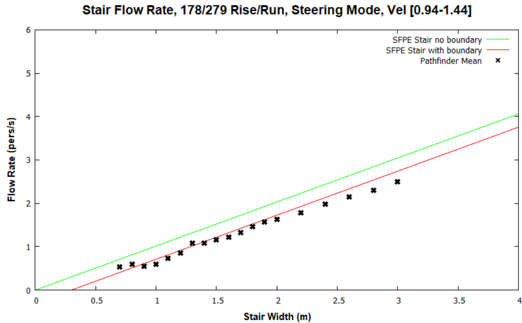
Figure 37: Stair flow rates for Steering mode and occupants with a max speed distribution of 1.19 \pm 0.25 m/s.
