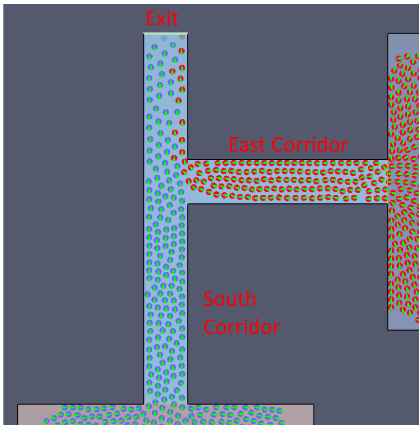
Figure 60: Model for merging at a corridor junction. Called an “adjacent’ geometry.
