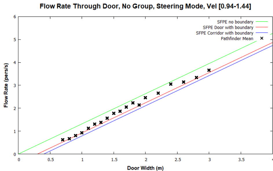
Figure 53: Door flow rates without grouping.
