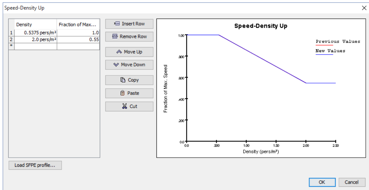
Figure 111: Normalized speed-density profile for 30-50 year old males on stairs up.
