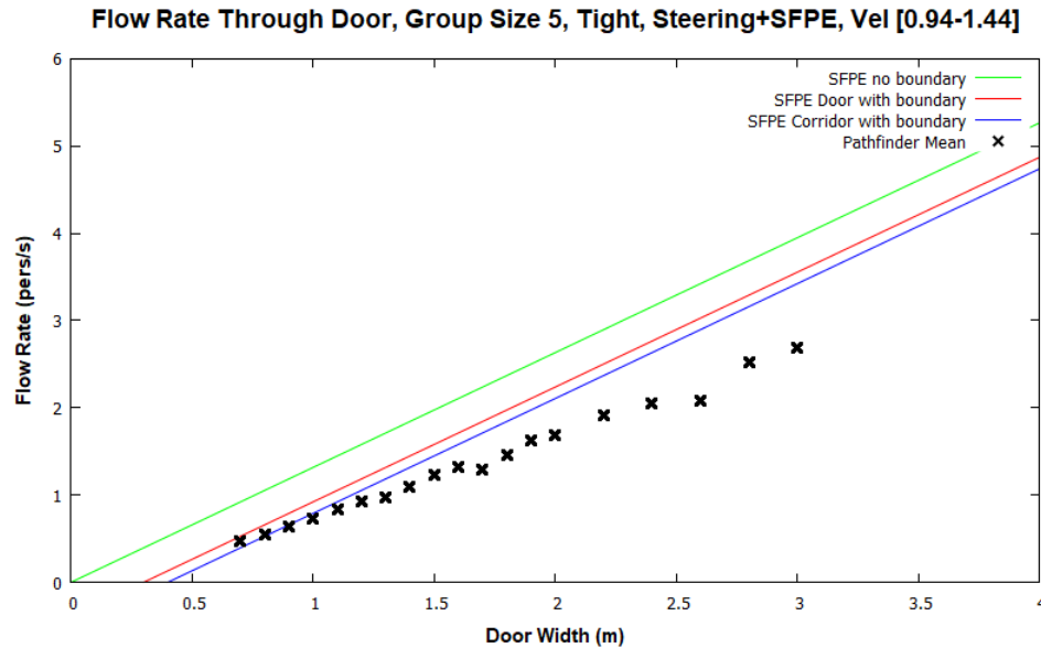
Figure 58: Door flow rates for steering+SFPE mode with default parameters and tight group of size 5.
