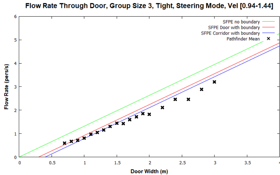
Figure 55: Door flow rates for steering mode with default parameters and tight group of size 3.
