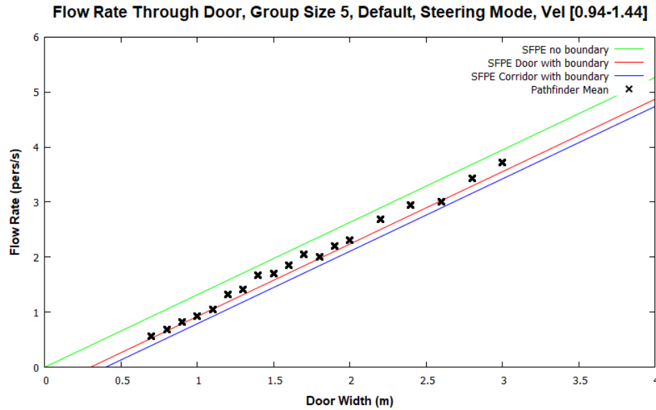
Figure 56: Door flow rates for steering mode with default parameters and group of size 5.
