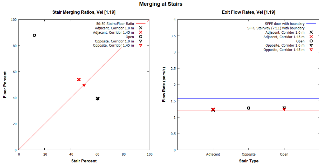
Figure 68: Merging ratios and exit flow rates for stair merging with a constant maximum occupant speed of 1.19 m/s.
