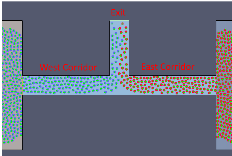
Figure 61: The geometry of a T-junction, called an "opposite" geometry.
