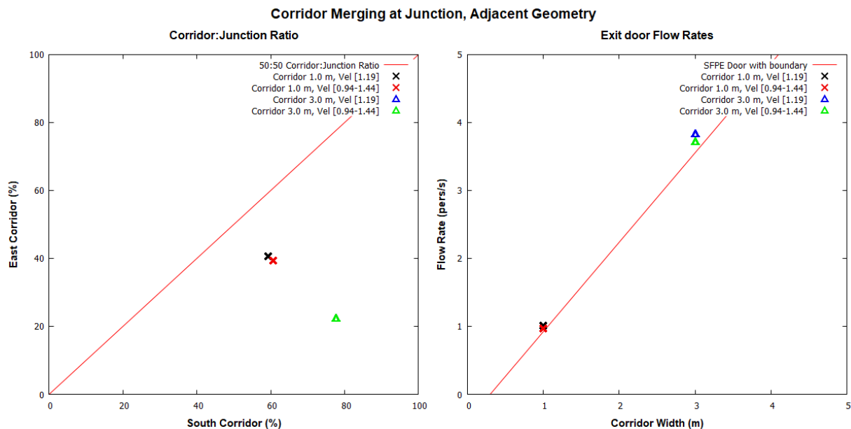
Figure 62: Merging ratios and exit door flow rates for merging at a corridor junction with “adjacent” configuration.
