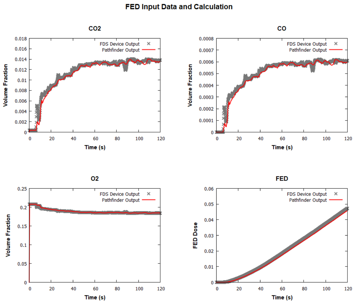
Figure 90: Comparison of FDS device output and Pathfinder input and FED calculation.
