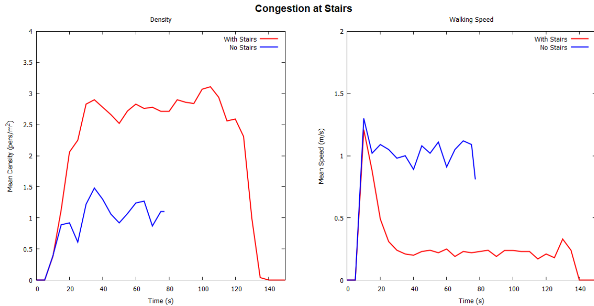
Figure 113: Comparison of density and walking speeds at base of stairs with and without stairs.
