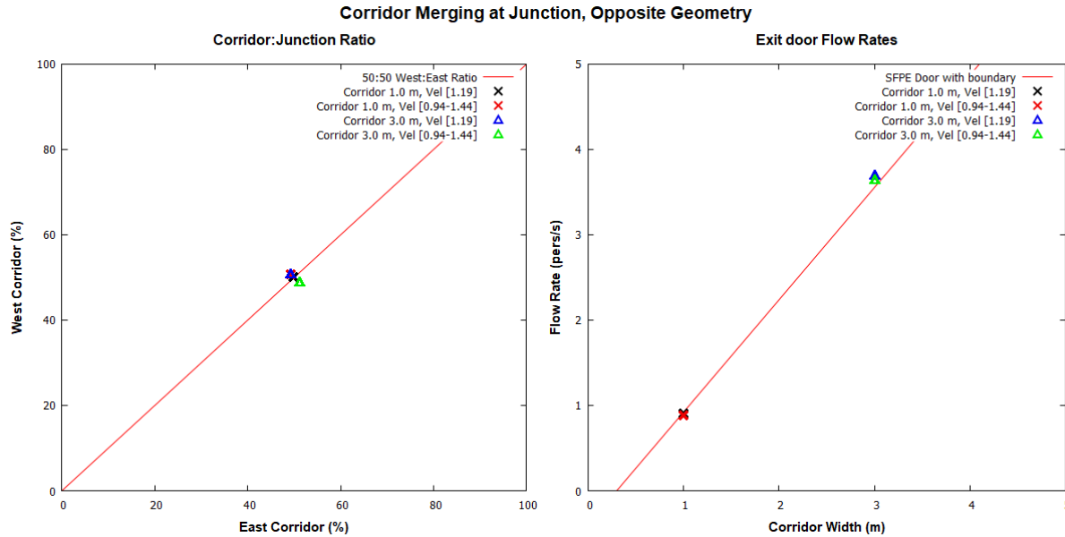
Figure 63: Merging ratios and exit door flow rates for merging at a corridor junction with "opposite" configuration.
