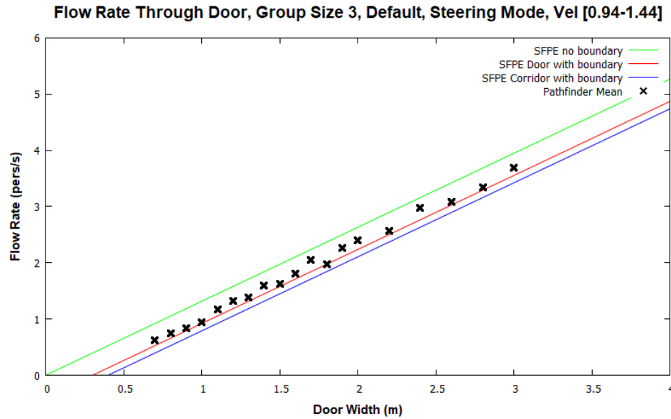
Figure 54: Door flow rates for steering mode with default parameters and group of size 3.
