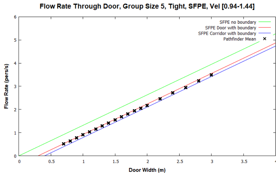
Figure 59: Door flow rates for SFPE mode with default parameters and tight group of size 5.
