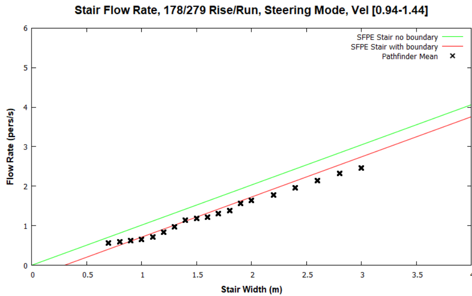
Figure 36: Stair flow rates for Steering mode and occupants with a max speed distribution of 1.19 \pm 0.25 m/s.
