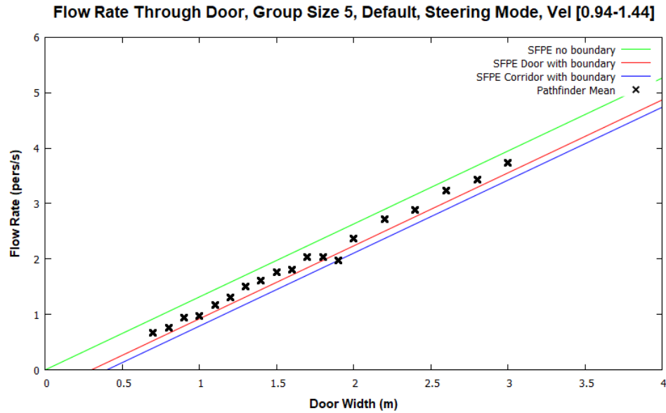
Figure 55: Door flow rates for steering mode with default parameters and group of size 5.
