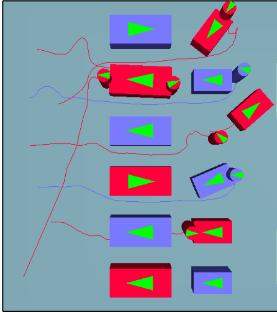
Figure 79: Solution at 9 seconds. Note that the order of evacuation was wheelchairs first. Three members of the red team are assisting wheelchairs, so the other two red team members are assisting the bed. The two blue team members are assisting wheelchairs.
