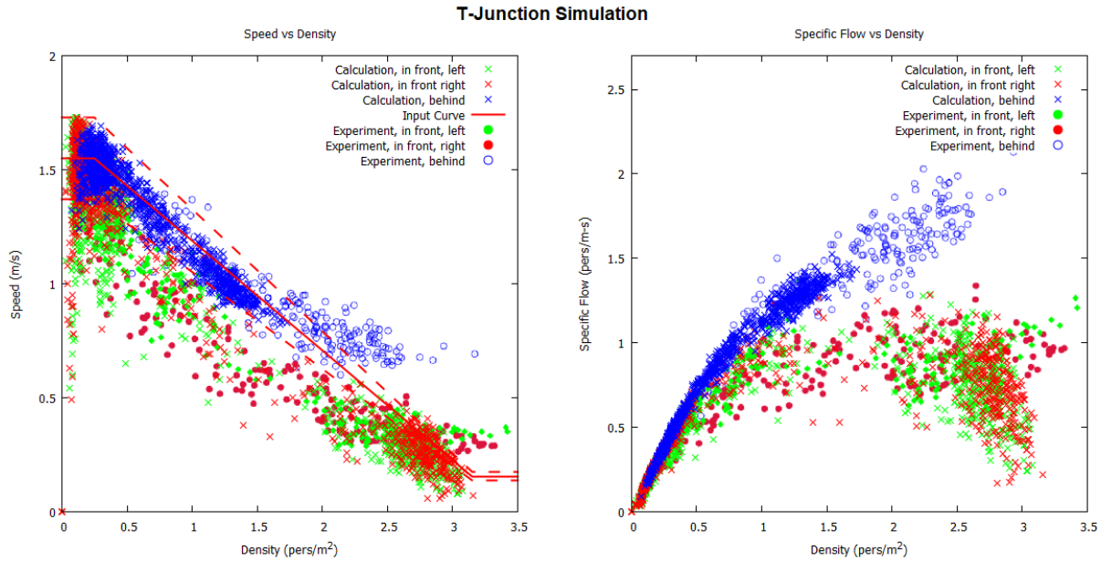
Figure 20: Speed-density results for Zhang and Seyfried experiment with measured speed-density input and uniform velocity distribution 1.55 \pm 0.18 m/s.
