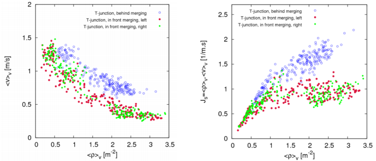
Figure 18: Fundamental diagrams for T-junction (Ref. Zhang et al., 2012).
