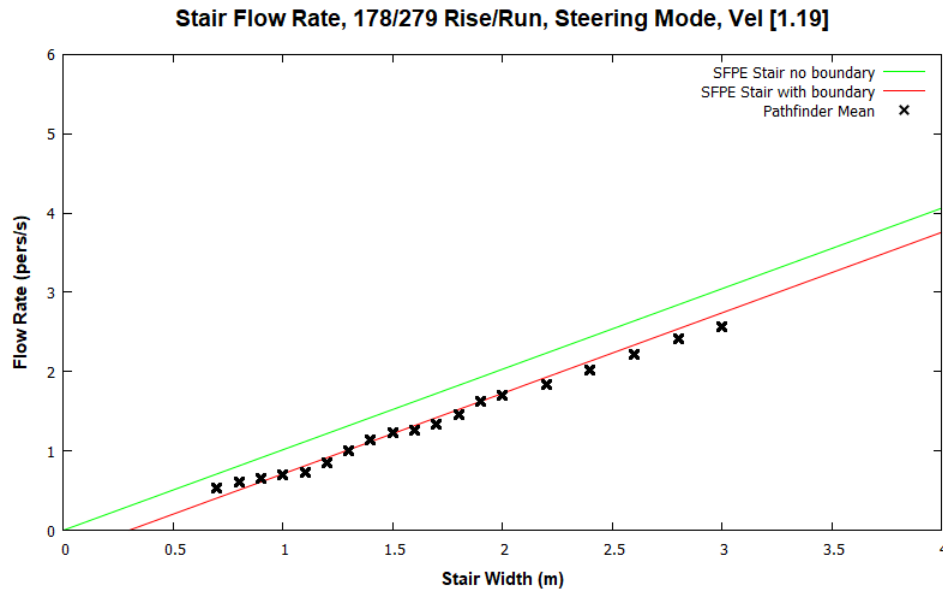
Figure 35: Stair flow rates for Steering mode and occupants with a max speed of 1.19 m/s.
