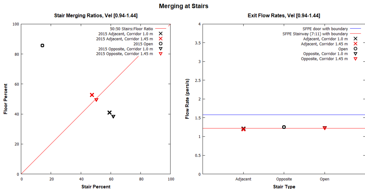
Figure 68: Merging ratios and exit flow rates for stair merging with a uniformly distributed maximum occupant speed of 1.19 \pm 0.25 m/s.
