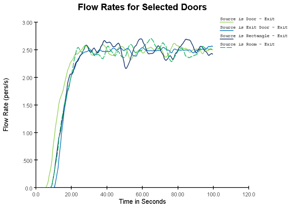
Figure 86: Exit door flow rates for the different source types. Results for steering behavior, SFPE and Steering+SFPE are similar.
