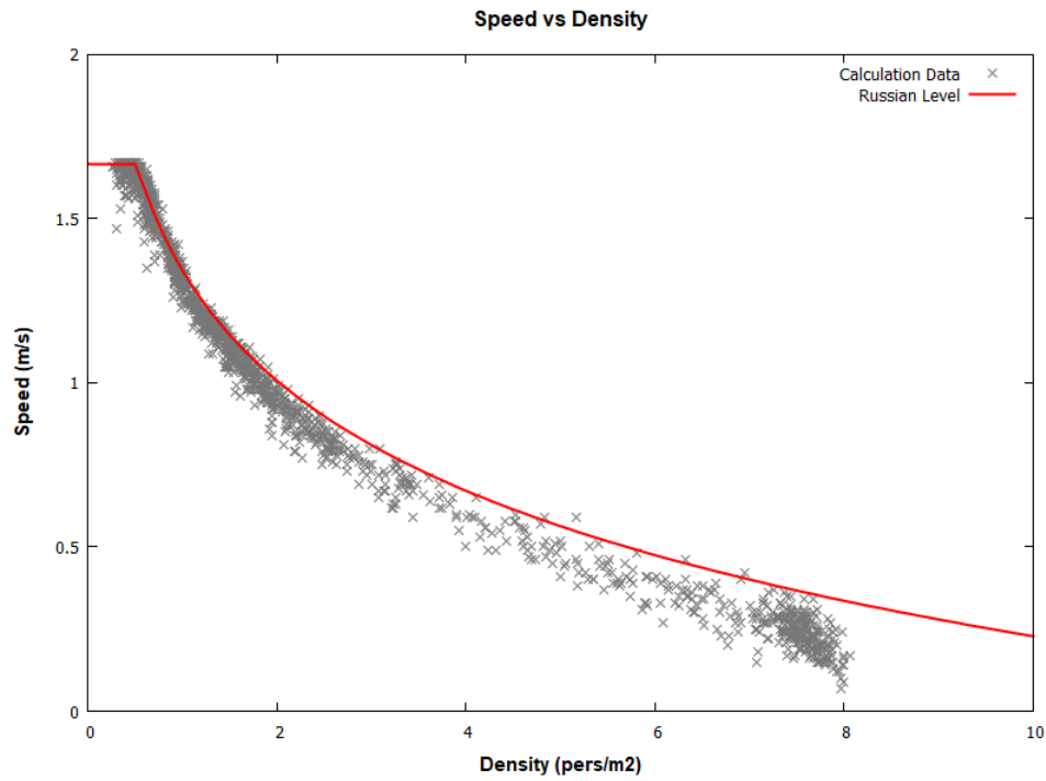
Figure 24: Speed-density results for Russian evacuation simulation, level path.
