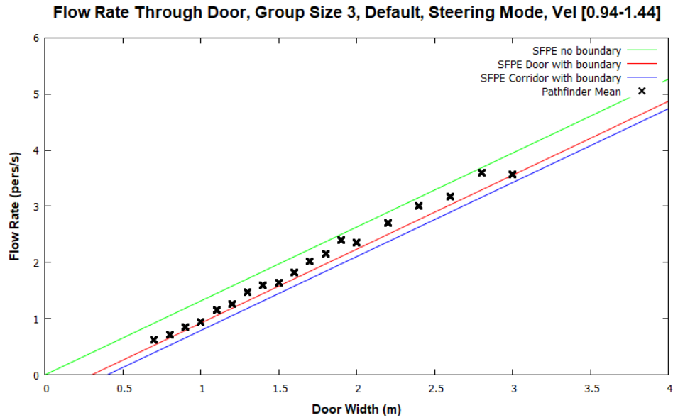
Figure 53: Door flow rates for steering mode with default parameters and group of size 3.
