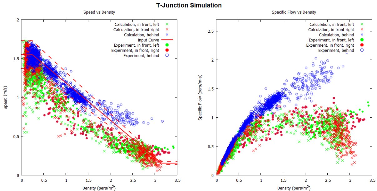
Figure 20: Speed-density results for Zhang and Seyfried experiment with measured speed-density input and uniform velocity distribution 1.55 \pm 0.18 m/s.
