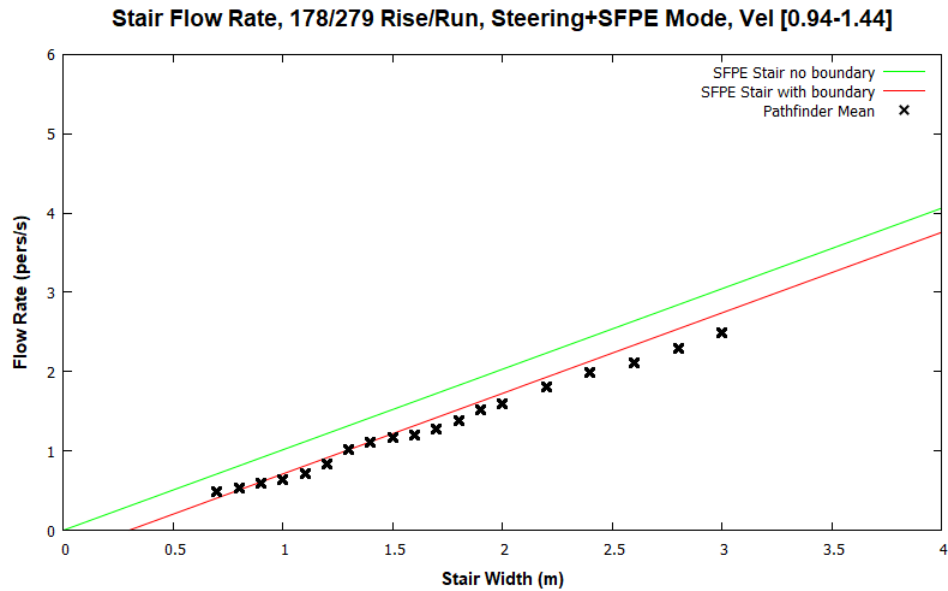
Figure 38: Stair flow rates for Steering+SFPE mode and occupants with a max speed distribution of 1.19 \pm 0.25 m/s.
