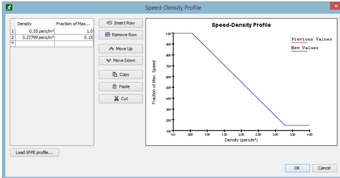
Figure 1: The default SFPE Speed-Density Profile
