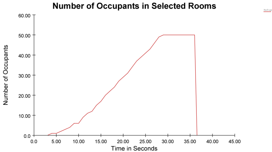
Figure 50: Occupants in the refuge room. Steering mode simulation.
