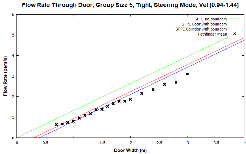
Figure 56: Door flow rates for steering mode with default parameters and tight group of size 5.
