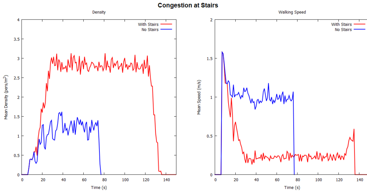
Figure 112: Comparison of density and walking speeds at base of stairs with and without stairs.
