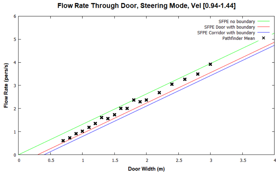
Figure 31: Door flow rates for Steering mode and occupants with a max speed distribution of 1.19 \pm 0.25 m/s.
