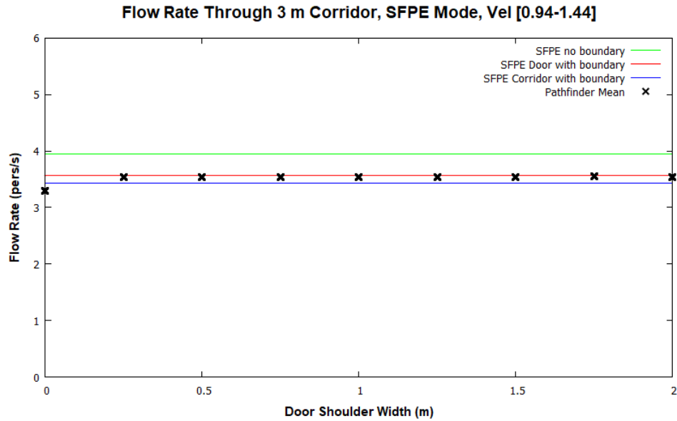
Figure 46: Corridor flow rates for 3 m corridor in SFPE Mode with varying entry shoulder widths. Occupants have a max speed distribution of 1.19 \pm 0.25 m/s.
