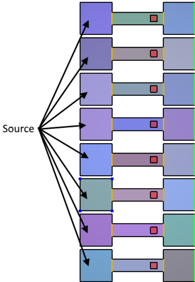
Figure 22: Pathfinder model for user-defined fundamental diagram. This case is for level movement. Similar models were used for stairs and ramps. The sources introduce occupants to the model, the red squares indicate where speed-density is measured, and the occupants exit on the right.
