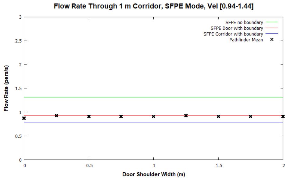
Figure 45: Corridor flow rates for 1 m corridor in SFPE Mode with varying entry shoulder widths. Occupants have a max speed distribution of 1.19 \pm 0.25 m/s.
