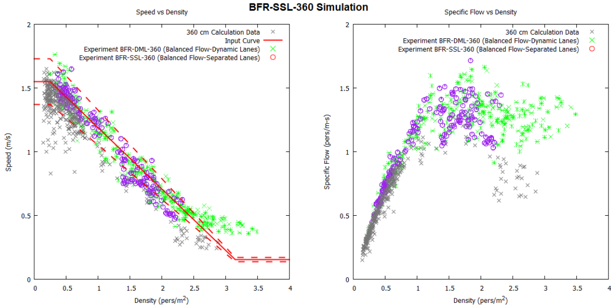
Figure 13: Speed-density results for Zhang and Seyfried experiment geometry, free choice of destination, with unidirectional speed-density input and uniform velocity distribution 1.55 \pm 0.18 m/s.
