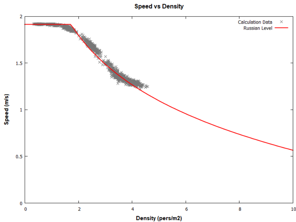
Figure 27: Speed-density results for Russian evacuation simulation, ramp down. For this case, the speed of occupants down the ramp is so large that it is not possible to feed occupants from the level supply room at a rate that gives a ramp density exceeding 4 pers/m 2 .
