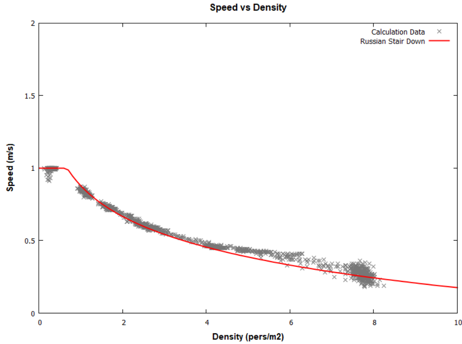
Figure 26: Speed-density results for Russian evacuation simulation, stairs up.
