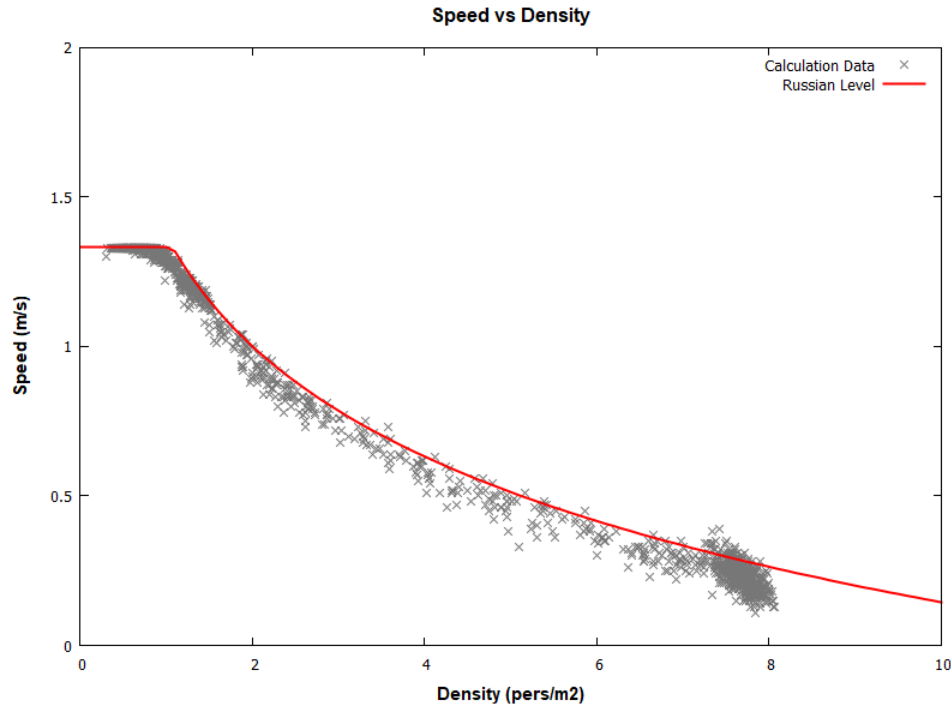
Figure 28: Speed-density results for Russian evacuation simulation, ramp up.
