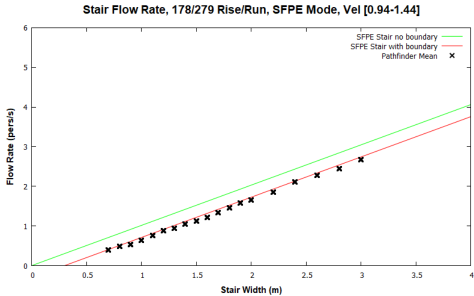
Figure 37: Stair flow rates for SFPE mode and occupants with a max speed distribution of 1.19 \pm 0.25 m/s.
