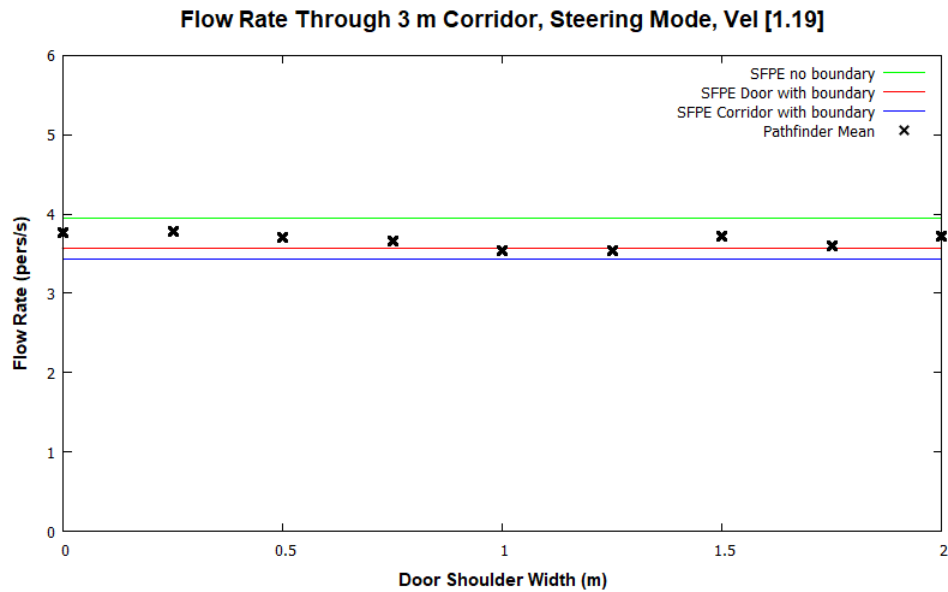
Figure 42: Corridor flow rates for 3 m corridor in Steering Mode with varying entry shoulder widths. Occupants have a constant max speed of 1.19 m/s.
