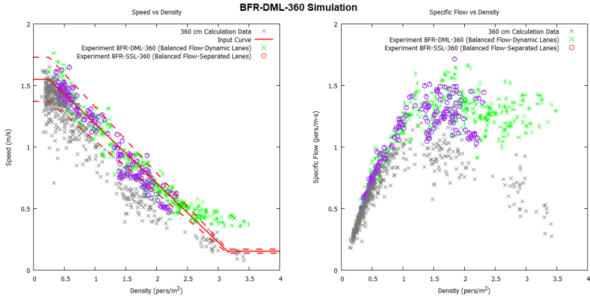
Figure 15: Speed-density results for Zhang and Seyfried experiment geometry, assigned destination, with unidirectional speed-density input and uniform velocity distribution 1.55 \pm 0.18 m/s.
