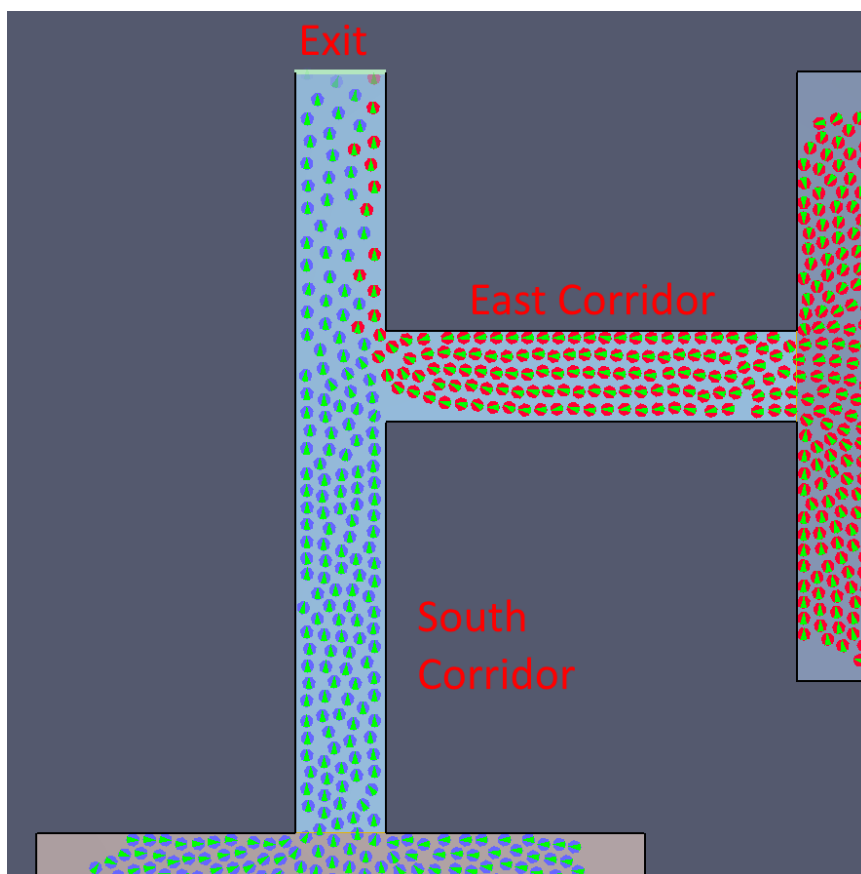
Figure 59: Model for merging at a corridor junction. Called an “adjacent’ geometry.
