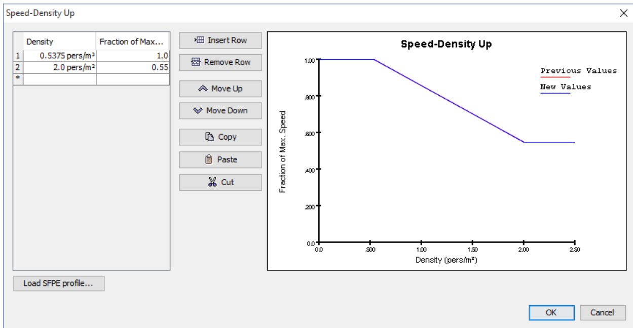
Figure 110: Normalized speed-density profile for 30-50 year old males on stairs up.
