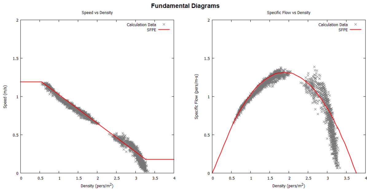
Figure 8: Speed-density and specific flow results with SFPE speed-density input and constant velocity 1.19 m/s.
