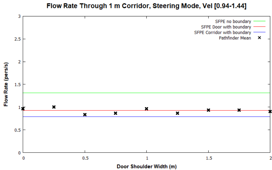
Figure 43: Corridor flow rates for 1 m corridor in Steering Mode with varying entry shoulder widths. Occupants have a max speed distribution of 1.19 \pm 0.25 m/s.
