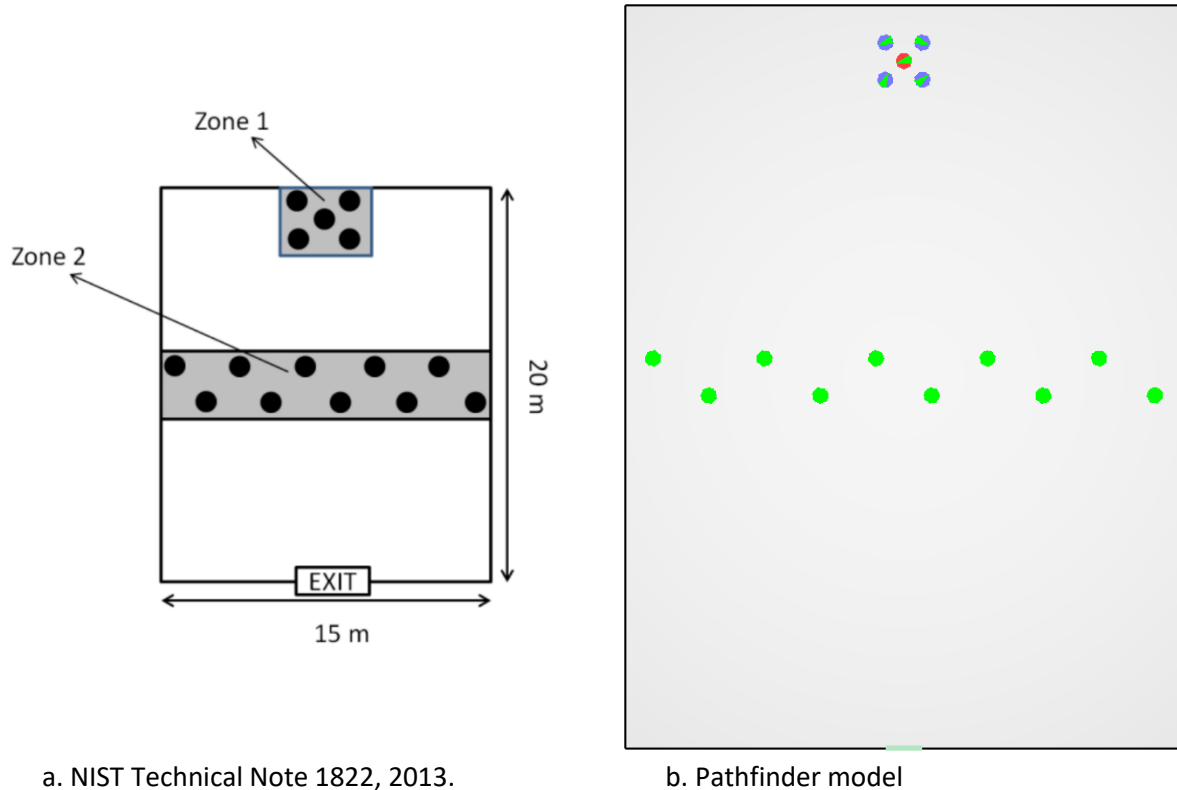
Figure 117: Geometry used for group behaviors verification (Verif.2.9).
