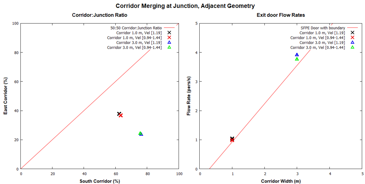
Figure 61: Merging ratios and exit door flow rates for merging at a corridor junction with "adjacent" configuration.
