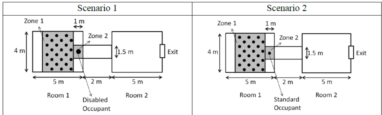
Figure 119: Geometry of movement disabilities verification (Verif.2.10). Figure from NIST Technical Note 1822, 2013.
