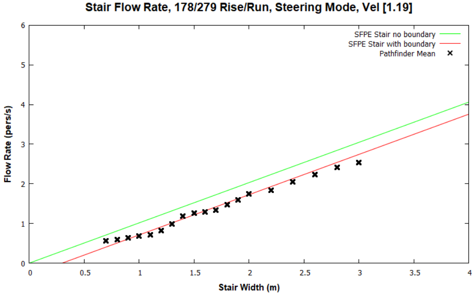
Figure 35: Stair flow rates for Steering mode and occupants with a max speed of 1.19 m/s.
