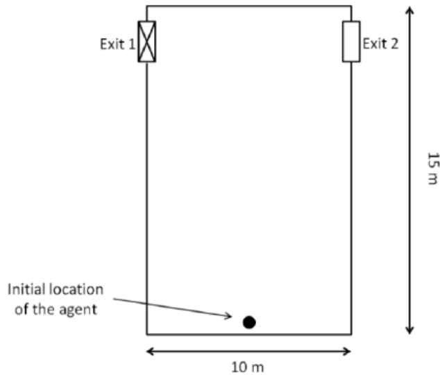
Figure 122: Geometry for dynamic availability of exits (Verif.4.1). Figure from NIST Technical Note 1822, 2013.
