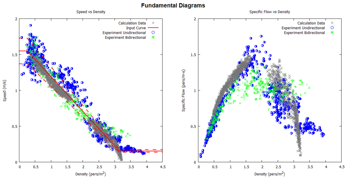
Figure 7: Speed-density results for Zhang and Seyfried experiment with measured speed-density input and uniform velocity distribution 1.55 \pm 0.18 m/s.
