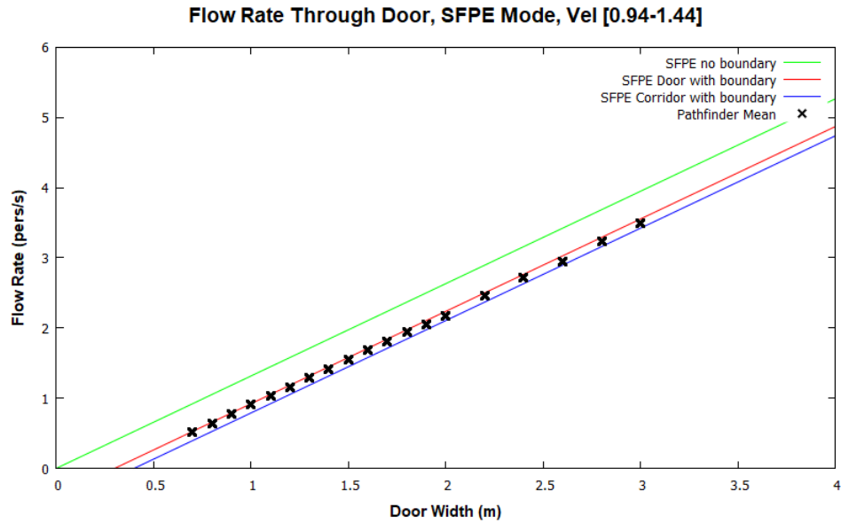
Figure 32: Door flow rates for SFPE mode and occupants with a max speed distribution of 1.19 \pm 0.25 m/s.
