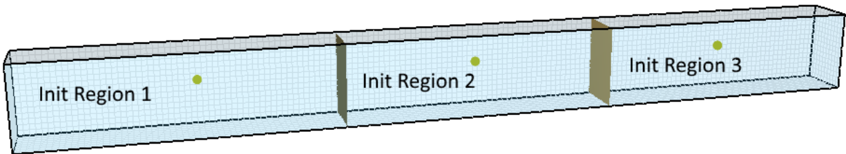
Figure 90: PyroSim model of FED calculation for moving occupant.
