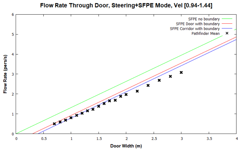
Figure 33: Door flow rates for Steering+SFPE mode and occupants with a max speed distribution of 1.19 \pm 0.25 m/s.
