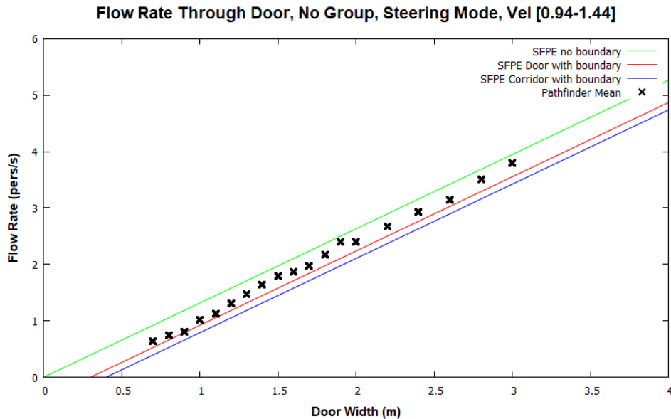
Figure 52: Door flow rates without grouping.
