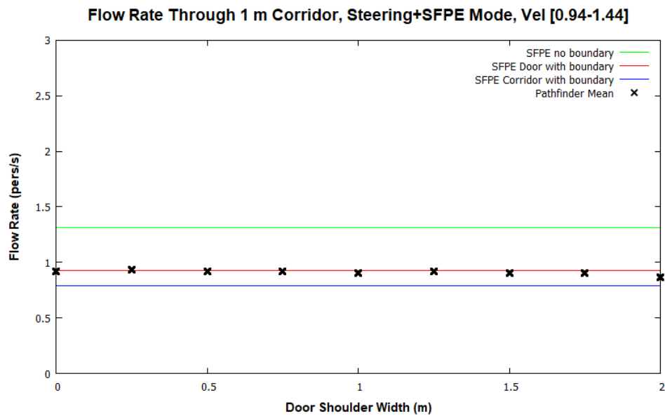
Figure 47: Corridor flow rates for 1 m corridor in Steering+SFPE Mode with varying entry shoulder widths. Occupants have a max speed distribution of 1.19 \pm 0.25 m/s.
