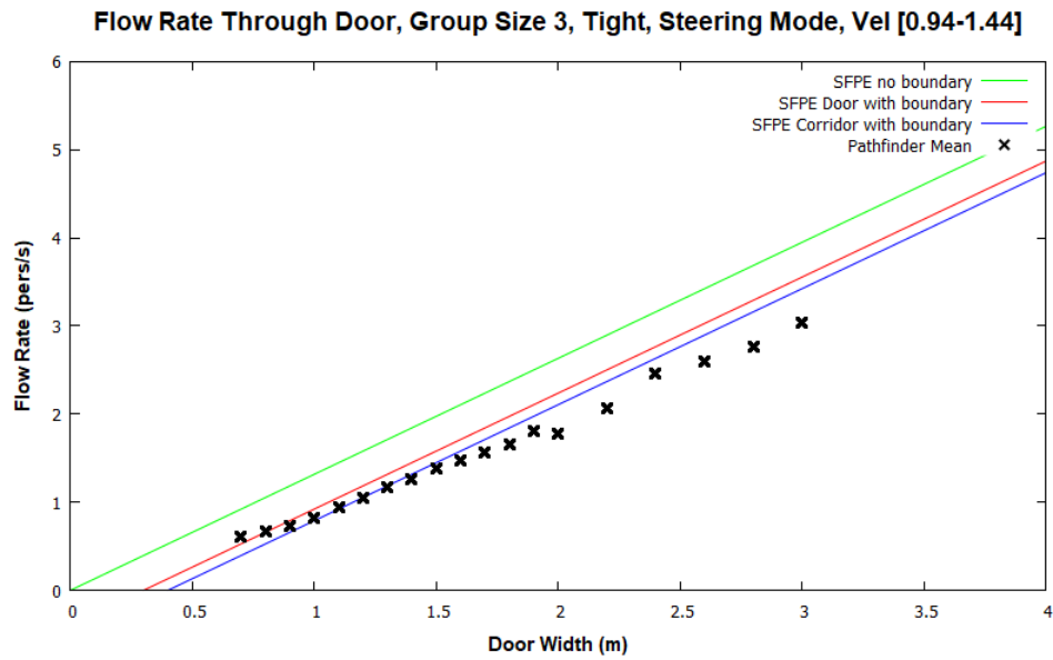
Figure 54: Door flow rates for steering mode with default parameters and tight group of size 3.
