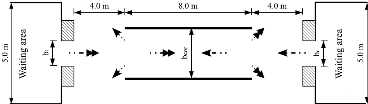
Figure 10: Setup and of bidirectional flow experiment. The widths of the corridor, left entrance, and right entrance were varied in the experiment (Ref. Zhang et al., 2012).
