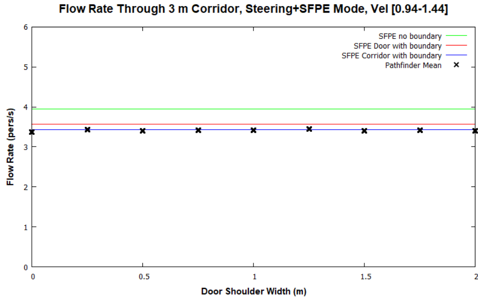
Figure 48: Corridor flow rates for 3 m corridor in Steering+SFPE Mode with varying entry shoulder widths. Occupants have a max speed distribution of 1.19 \pm 0.25 m/s.
