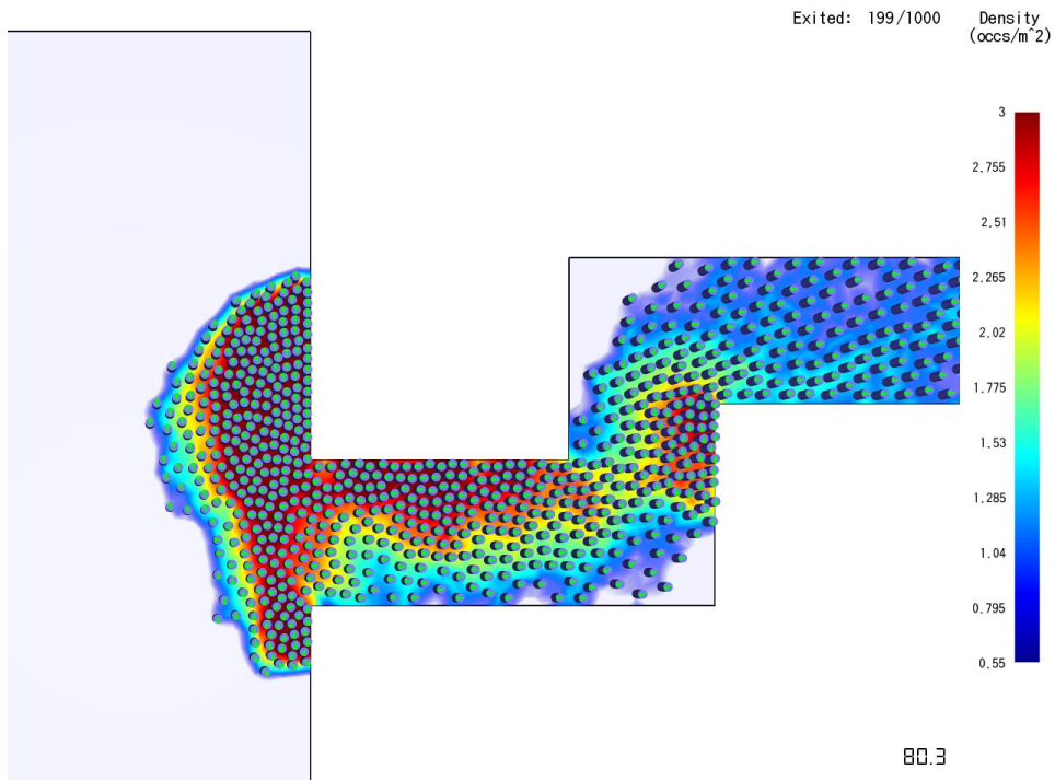
Figure 74: Steering mode showing use of the corridor with two corners.
