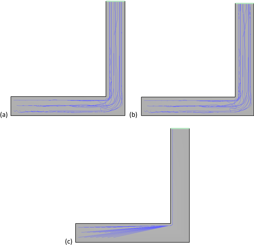
Figure 99: Occupant trails for boundary test: (a) Steering mode, (b) Steering+SFPE mode, (c) SFPE mode (in this mode occupants can overlap).
