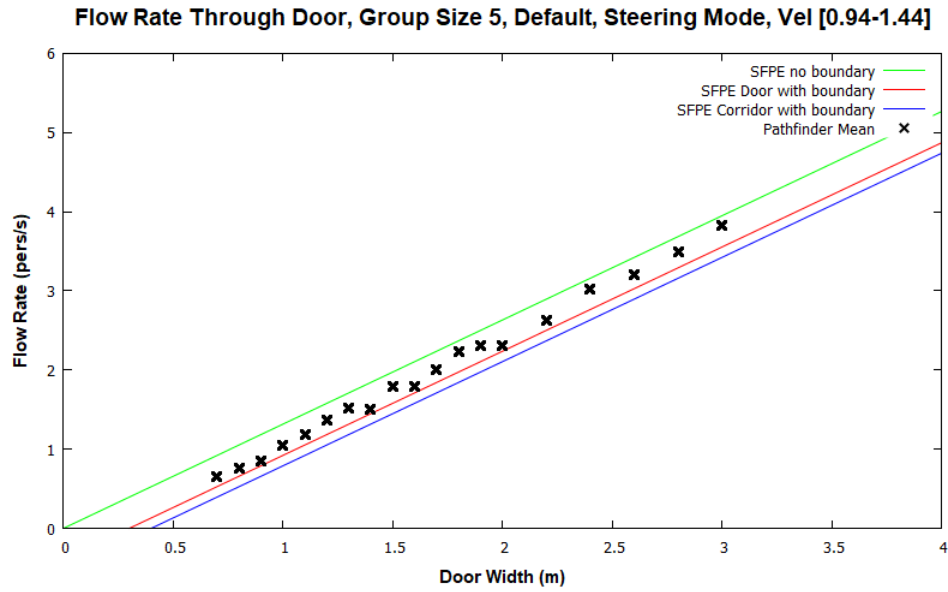
Figure 55: Door flow rates for steering mode with default parameters and group of size 5.
