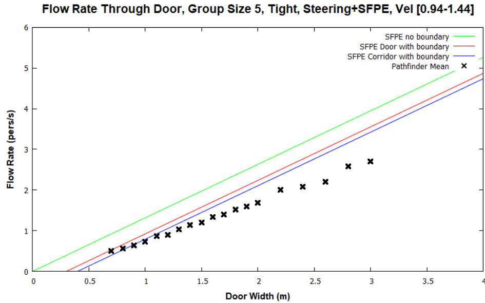
Figure 57: Door flow rates for steering+SFPE mode with default parameters and tight group of size 5.
