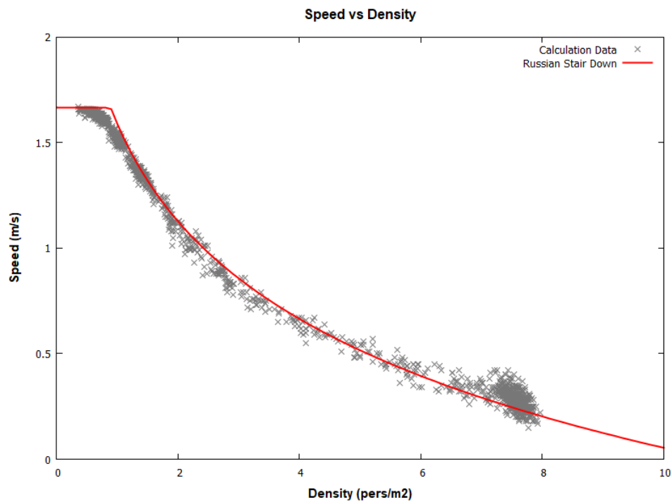
Figure 25: Speed-density results for Russian evacuation simulation, stairs down.
