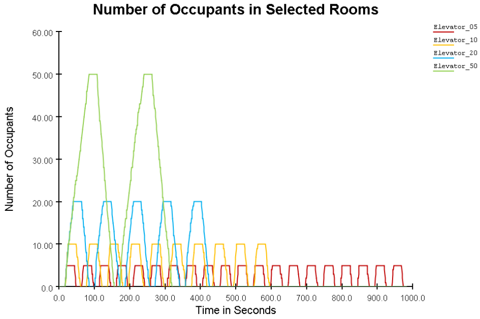
Figure 72: Observed elevator loading for steering mode
