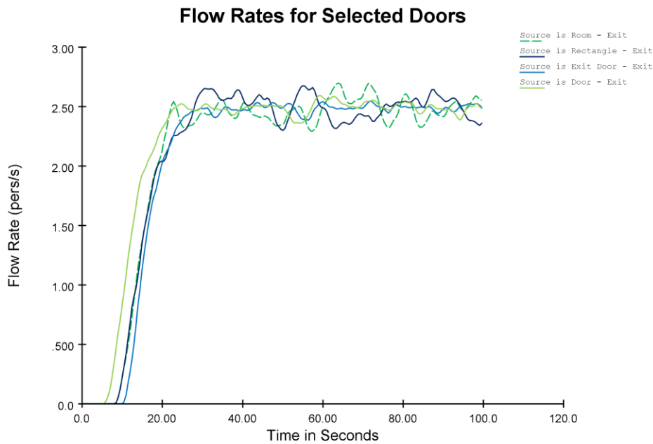
Figure 86: Exit door flow rates for the different source types. Results for steering behavior (shown). SFPE and Steering+SFPE are similar.
