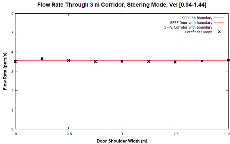
Figure 44: Corridor flow rates for 3 m corridor in Steering Mode with varying entry shoulder widths. Occupants have a max speed distribution of 1.19 \pm 0.25 m/s.
